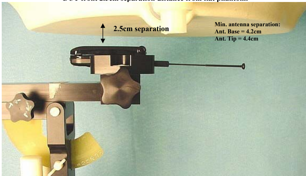
Figure 7. Assessment @ the Face (Flip closed) DUT front 2.5cm separation distance from flat phantom.
