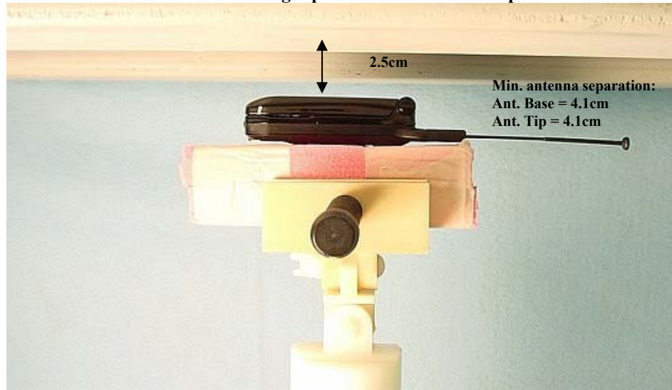
Figure 10. Body assessment @ 2.5cm DUT with back housing separated 2.5cm from the phantom.
