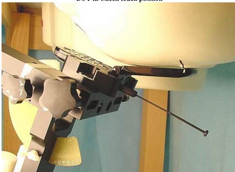
Figure 3. Assessment @ the Left ear DUT in Cheek touch position
