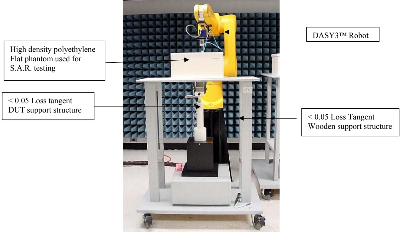
Figure 10: Robot Test System (Flat Phantom)
