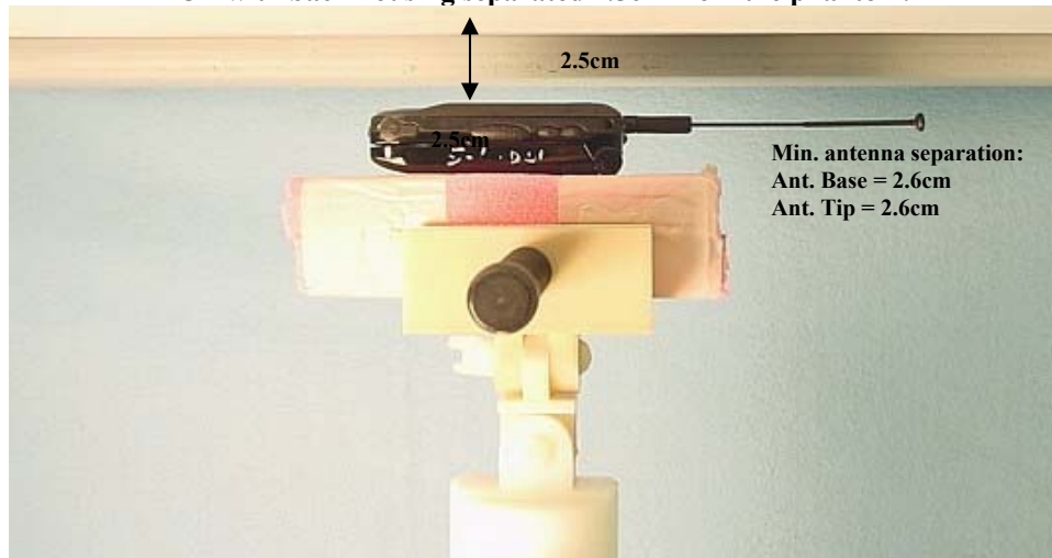
Figure 10. Body assessment @ 2.5cm DUT with back housing separated 2.5cm from the phantom.
