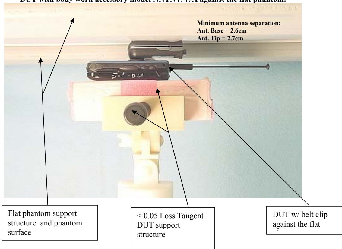
Figure 1: Highest S.A.R. Test Position (@ body) DUT with body worn accessory model NNTN4747A against the flat phantom.
