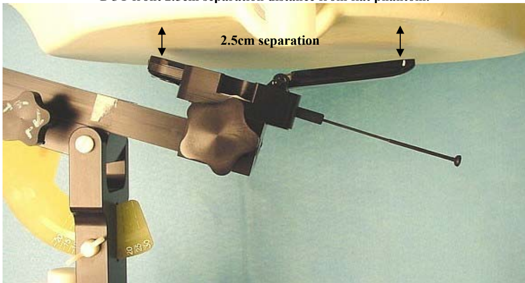
Figure 7. Assessment @ the Face (Flip closed) DUT front 2.5cm separation distance from flat phantom.
