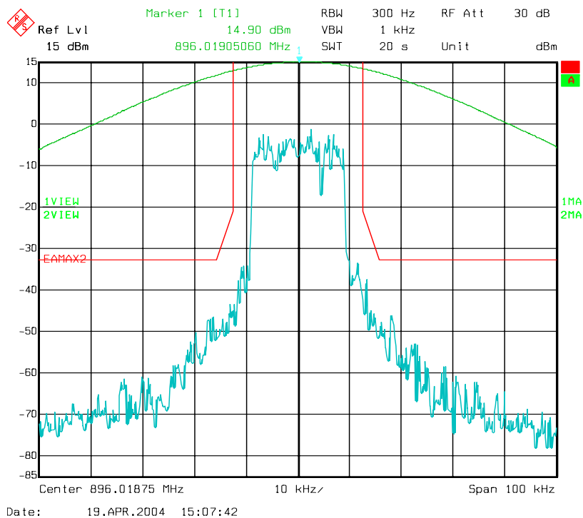
Figure 6-21: Quad-64QAM Modulation performance relative to EA-mask 47 CFR 90.669(a) (MAXIMUM POWER SETTING)
