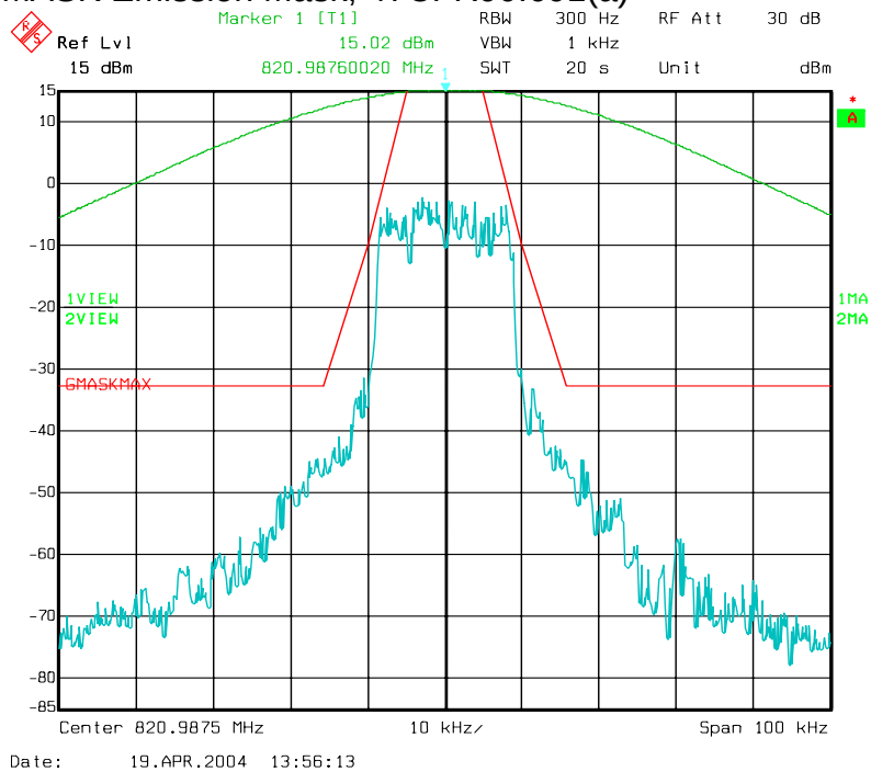
Figure 6-5: Quad-QPSK Modulation performance relative to GMASK 47 CFR 90.210(g)
