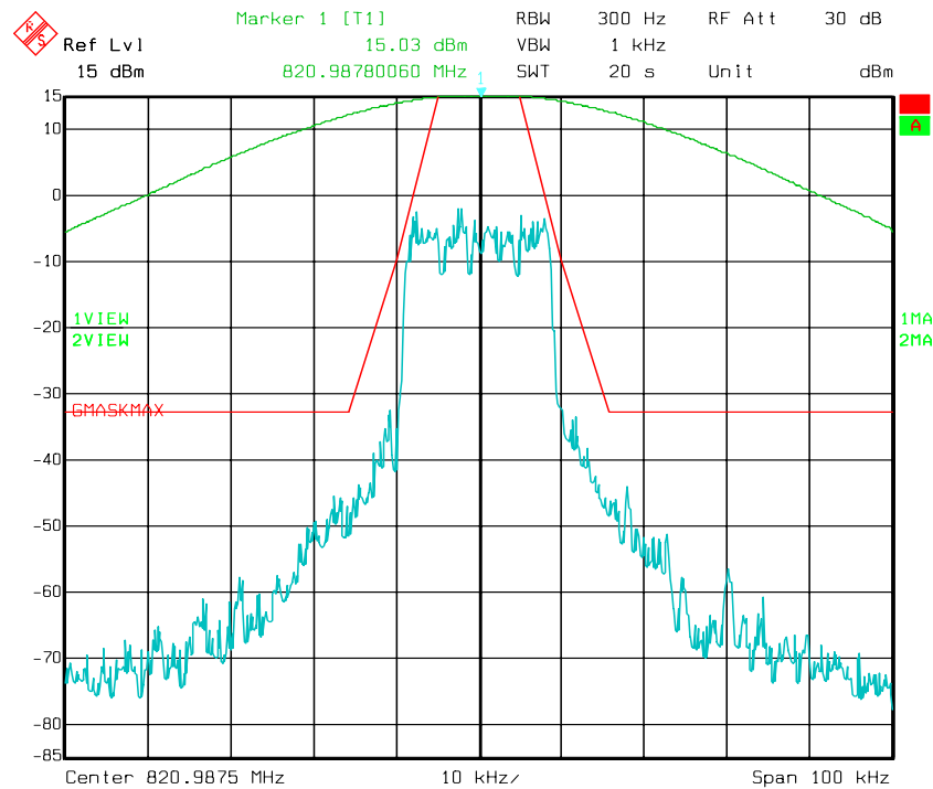
Figure 6-9a: Quad-16QAM Modulation performance relative to G-Mask 47 CFR 90.210(g) (MAXIMUM POWER SETTING)
