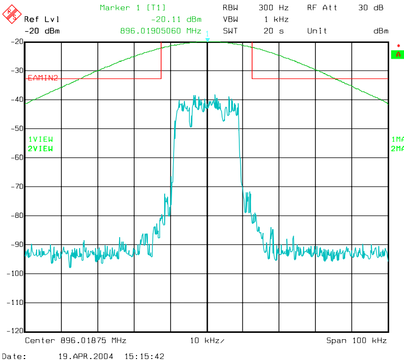
Figure 6-22: Quad-64QAM Modulation performance relative to EA-mask 47 CFR 90.669(a) (MINIMUM POWER SETTING)
