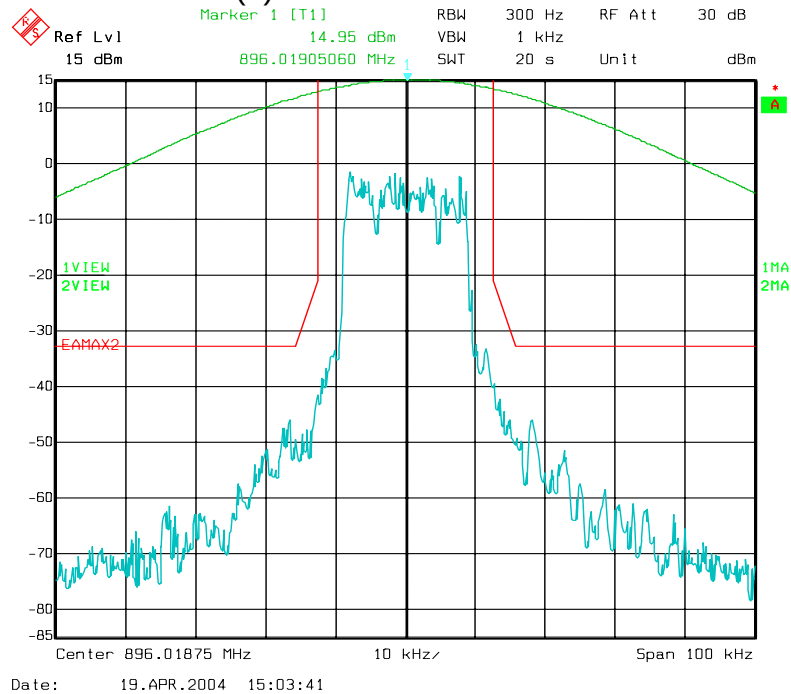
Figure 6-17: Quad-QPSK Modulation performance relative to EA-mask 47 CFR 90.669(a) (MAXIMUM POWER SETTING)
