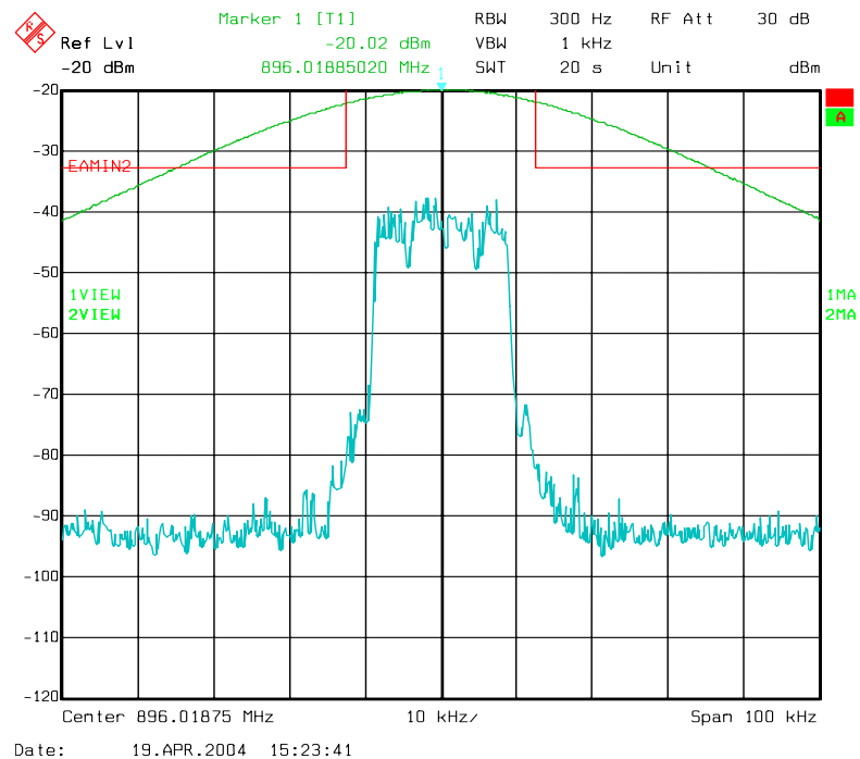
Figure 6-18: Quad-QPSK Modulation performance relative to EA-mask 47 CFR 90.669(a) (MINIMUM POWER SETTING)
