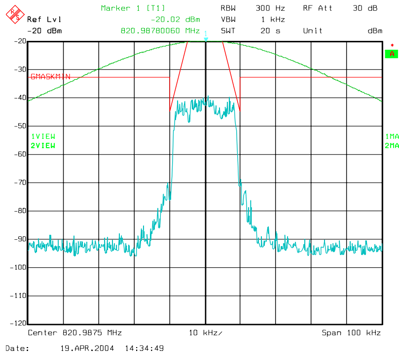
Figure 6-14: Quad-64QAM Modulation performance relative to G-mask 47 CFR 90.210(g) (MINIMUM POWER SETTING)
