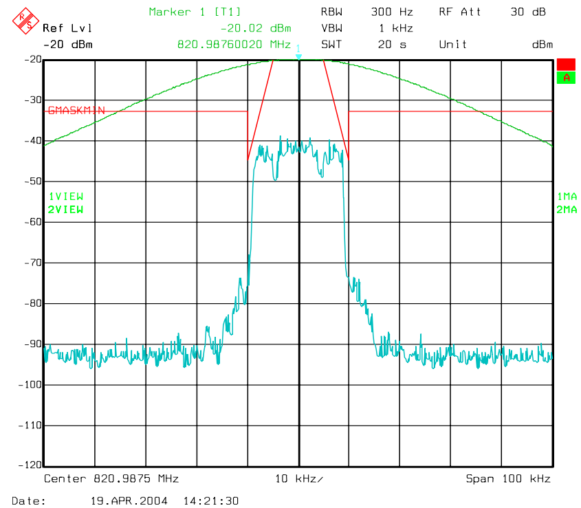
Figure 6-10a: Quad-16QAM Modulation performance relative to G-Mask 47 CFR 90.210(g) (MINIMUM POWER SETTING)
