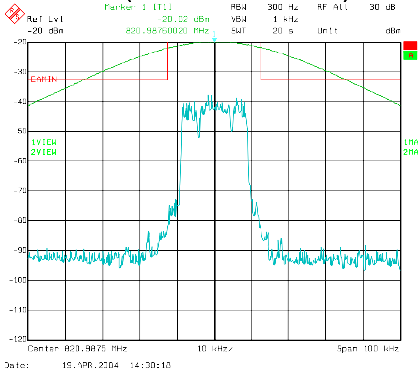
Figure 6-8: Quad-QPSK Modulation performance relative to EA-mask 47 CFR 90.691. (MINIMUM POWER SETTING)
