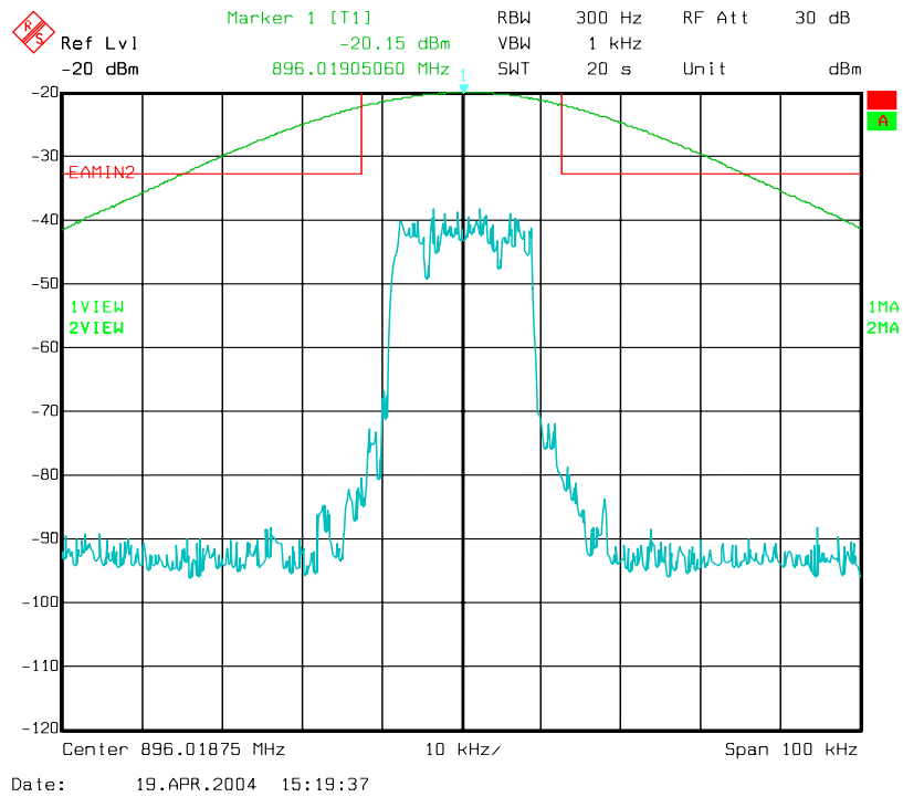
Figure 6-20a: Quad-16QAM Modulation performance relative to EA-mask 47 CFR 90.669(a) (MINIMUM POWER SETTING)
