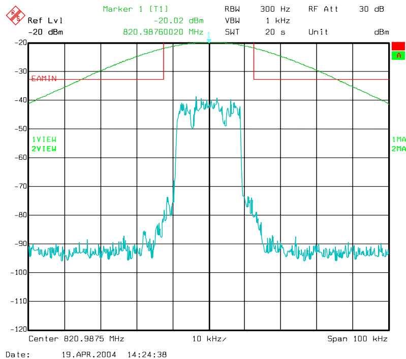
Figure 6-12a: Quad-16QAM Modulation performance relative to EA-mask 47 CFR 90.691. (MINIMUM POWER SETTING)
