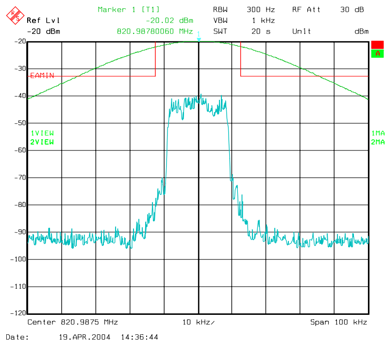
Figure 6-16: Quad-64QAM Modulation performance relative to EA-mask 47 CFR 90.691. (MINIMUM POWER SETTING)
