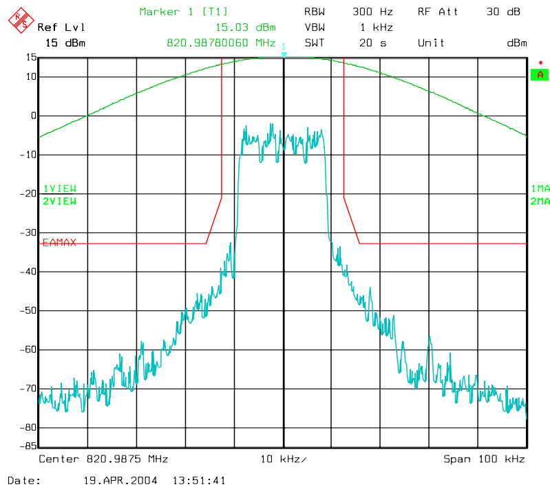
Figure 6-11a: Quad-16QAM Modulation performance relative to EA-mask 47 CFR 90.691. (MAXIMUM POWER SETTING)
