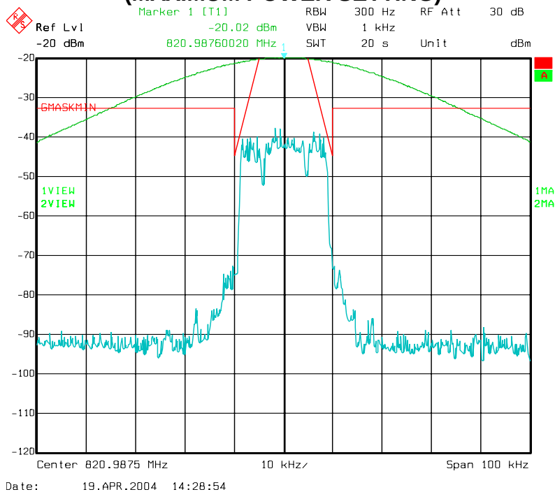
Figure 6-6: Quad-QPSK Modulation performance relative to GMASK 47 CFR 90.210(g)
