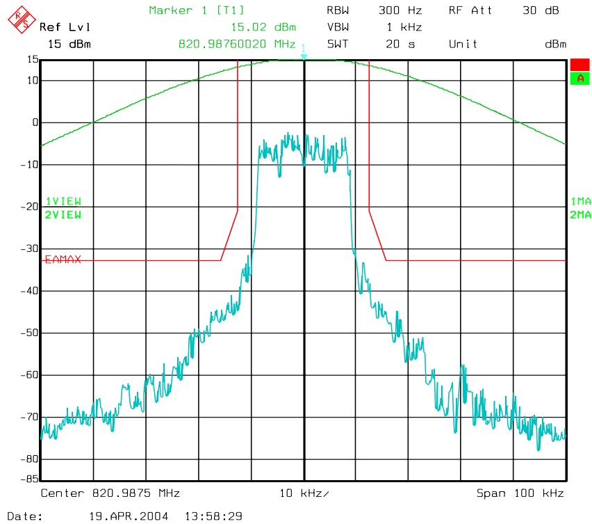
Figure 6-7: Quad-QPSK Modulation performance relative to EA-mask 47 CFR 90.691.
