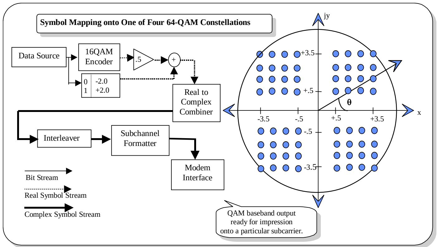
Figure 6-5: Symbol Mapping onto One of Four 64-QAM Constellations
