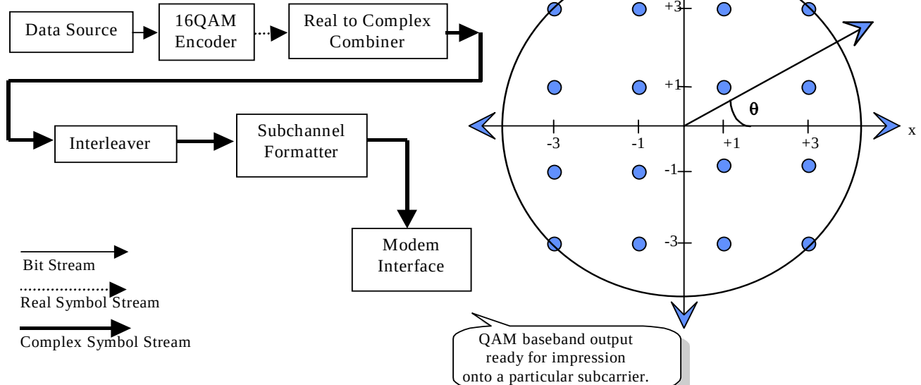
Figure 6-4: Symbol Mapping onto One of Four 16-QAM Constellations
