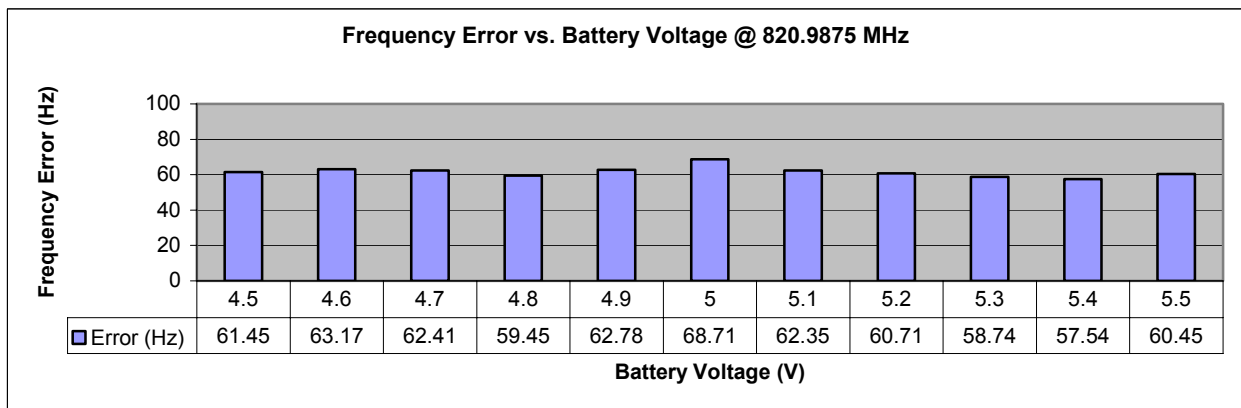
Figure 6-43: Transmitter Frequency Stability (800 MHz band) - Frequency Error vs. Voltage
