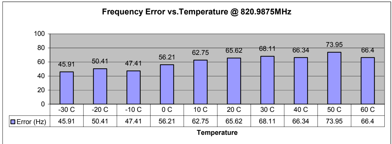
Figure 6-42: Transmitter Frequency Stability (800 MHz band) – Frequency Error vs. Temperature
