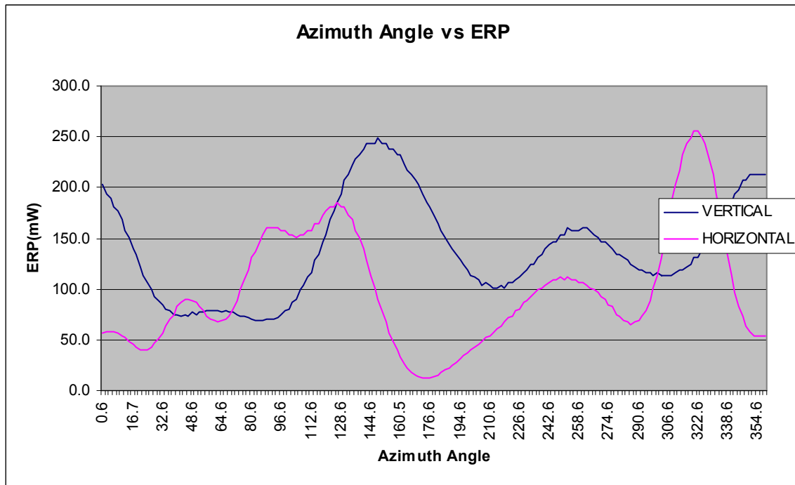
Figure 6-44: Land mobile Band: Scaled Maximum ERP(mW) vs. Azimuth Angle
