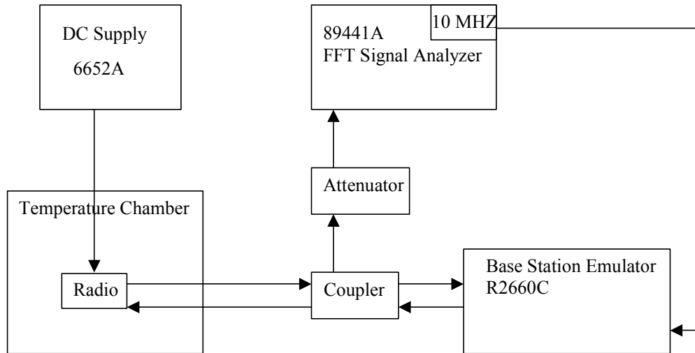
Figure 7-1: Transmit Frequency Measurement Setup
