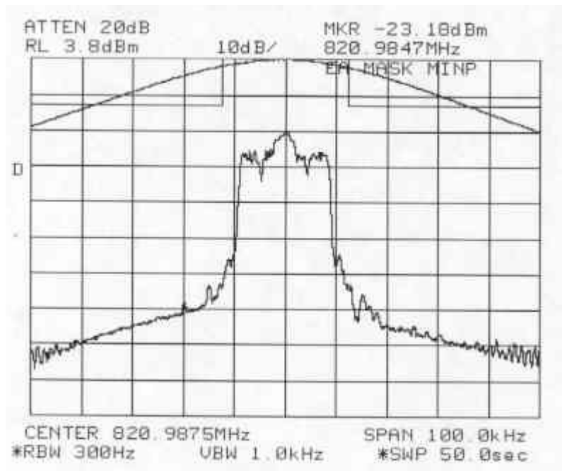
Figure 6-12b: Quad-16QAM Modulation performance relative to mask 47 CFR 90.691. (MINIMUM POWER SETTING) (Split 3:1 Interleaving)
