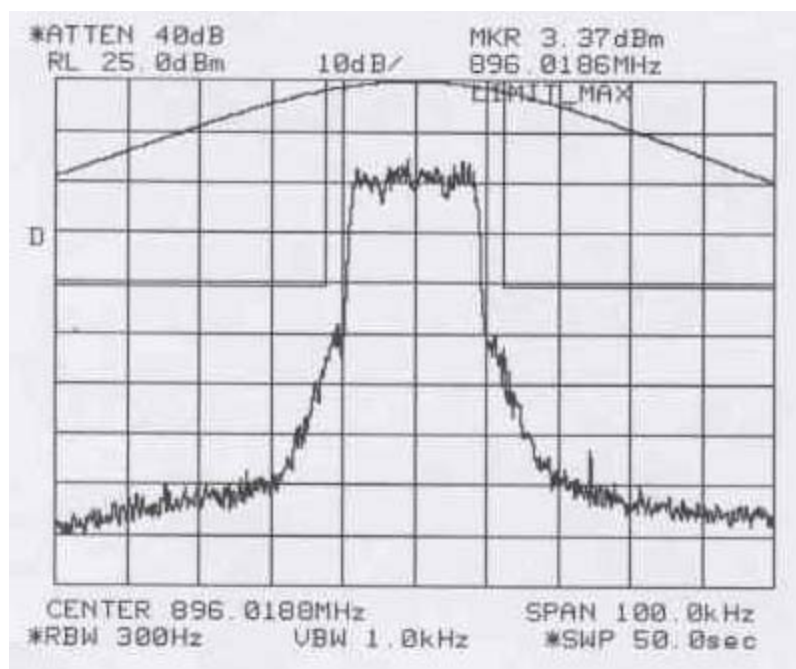
Figure 6-19b: Quad-16QAM Modulation performance relative to mask 47 CFR 90.669(a) (MAXIMUM POWER SETTING) (Split 3:1 Interleaving)
