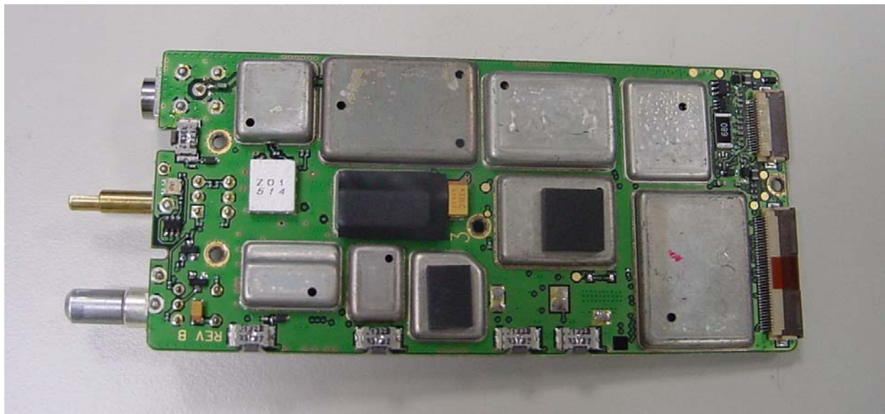
Figure 9-1: Top Side of RF PCB with shields.
