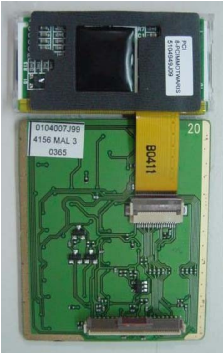
Figure 9-4: Bottom Side of Controller PCB.
