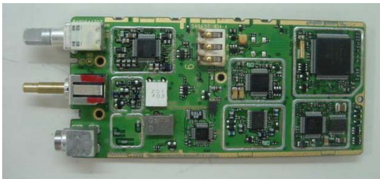
Figure 9-4: Bottom Side of RF PCB.
