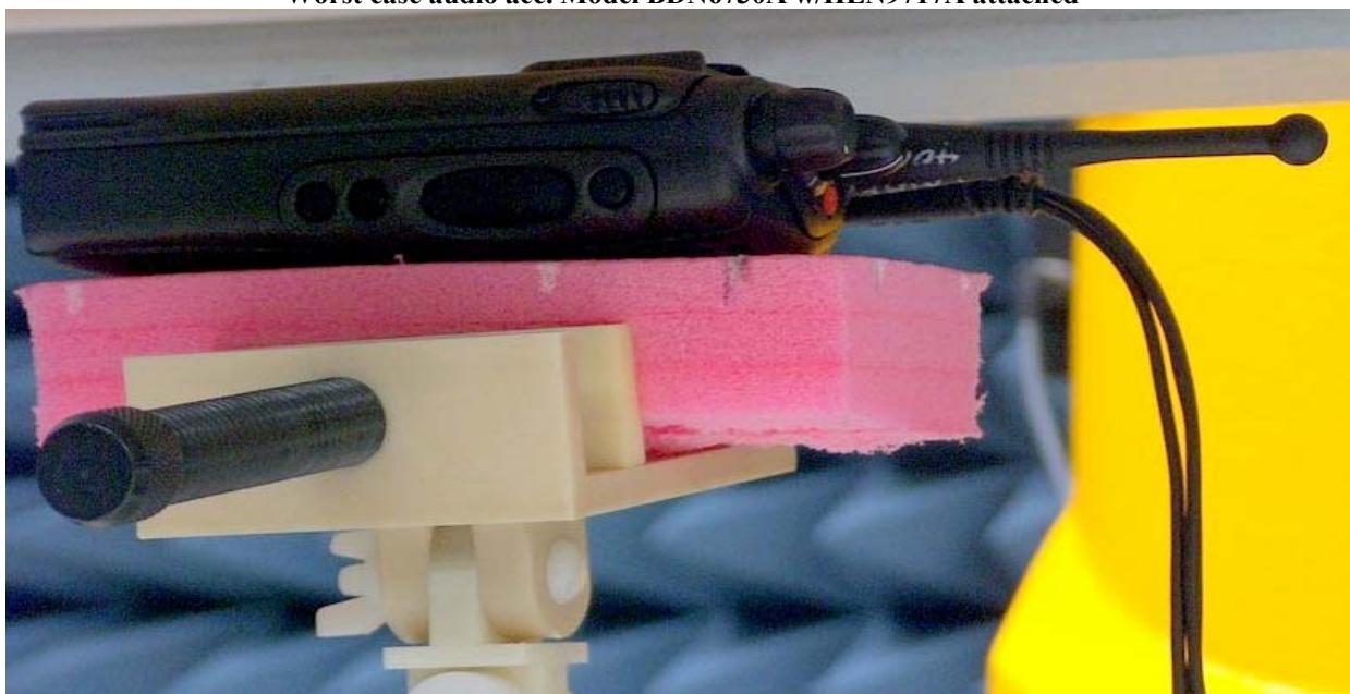
Figure 3: Body Assessment DUT w/ back housing separated 2.5cm from the phantom Worst case audio acc. Model BDN6730A w/HLN9717A attached
