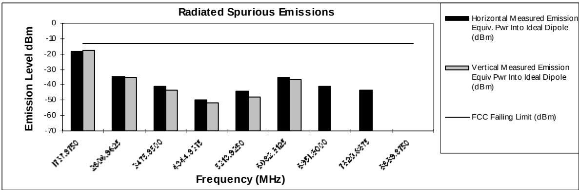
Figure 6G-6: 2 Watts, 869.00 MHz
