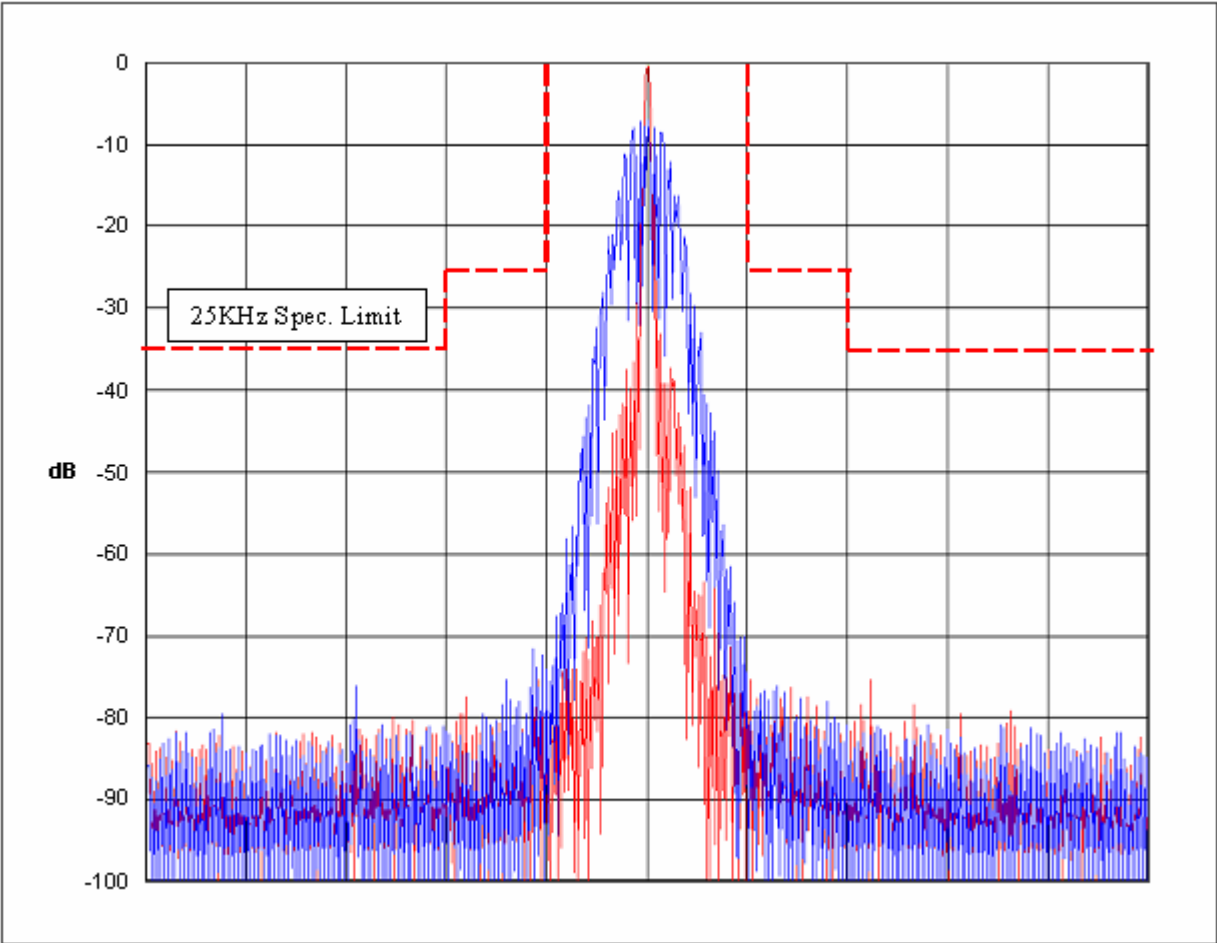
Figure 6E-5: Mask B; 25 kHz Channel Spacing, DTMF Modulation and TPL Tone Modulation; 16K0F3E
