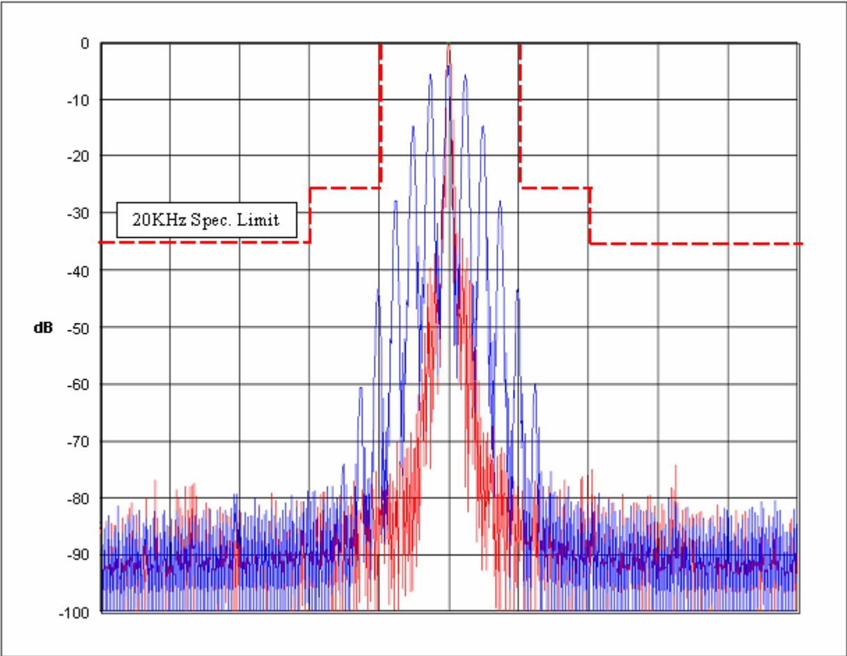
Figure 6E-7: Mask B; 20 kHz Channel Spacing, 2500 Hz Audio Modulation Only; 16K0F3E
