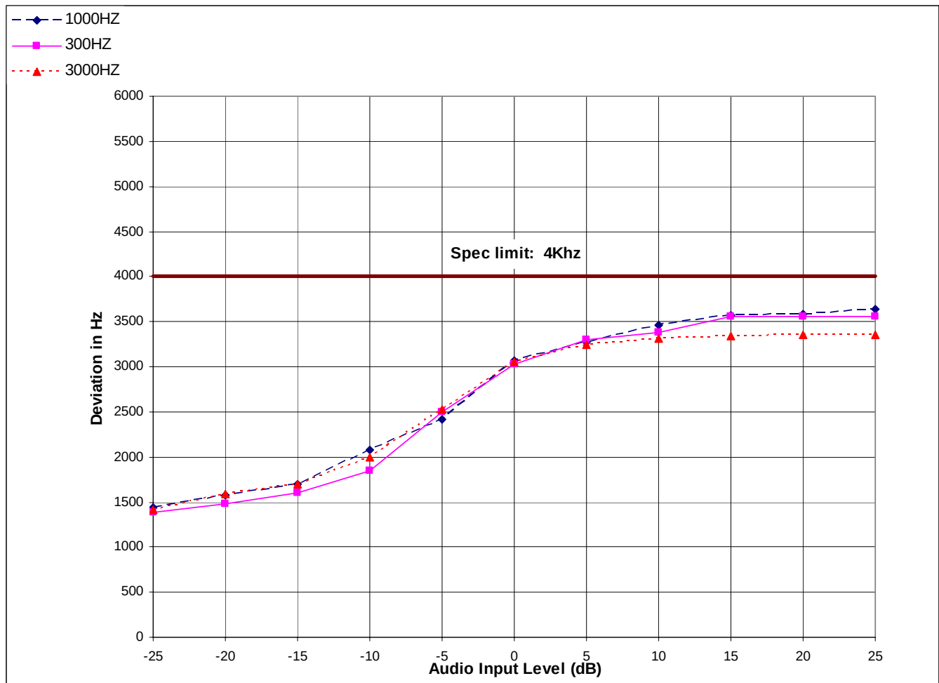
Figure 6D-4: 20 kHz Channel Spacing, Carrier Squelch Mode
