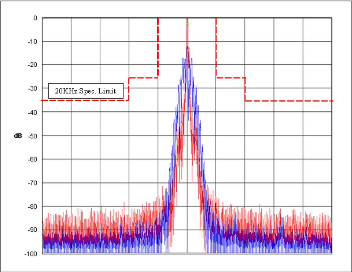
Figure 6E-12: Mask B; 20 kHz Channel Spacing, DTMF Modulation and DPL Tone Modulation; 16K0F3E
