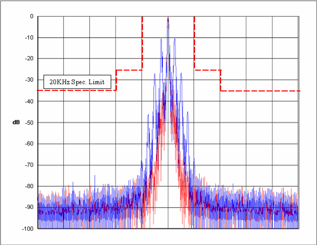
Figure 6E-8: Mask B; 20 kHz Channel Spacing, 2500 Hz Audio and TPL Tone Modulation; 16K0F3E
