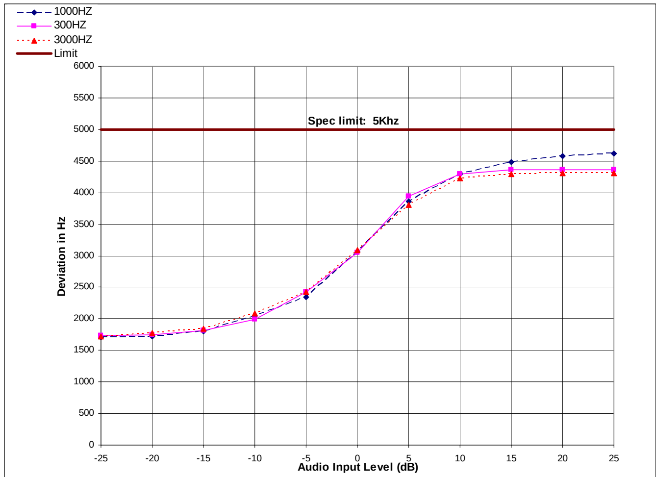
Figure 6D-2: 25 kHz Channel Spacing, Tone Private Line (TPL) Mode
