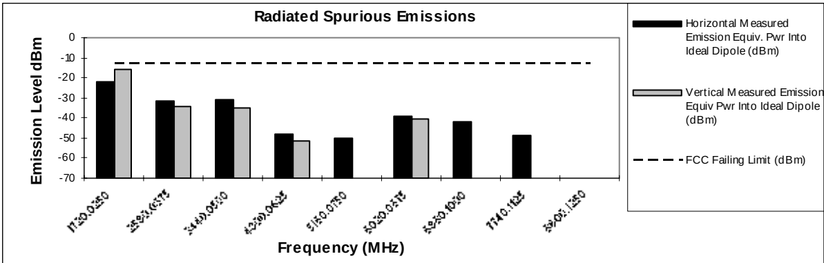
Figure 6G-5: 2 Watts, 860.0125 MHz
