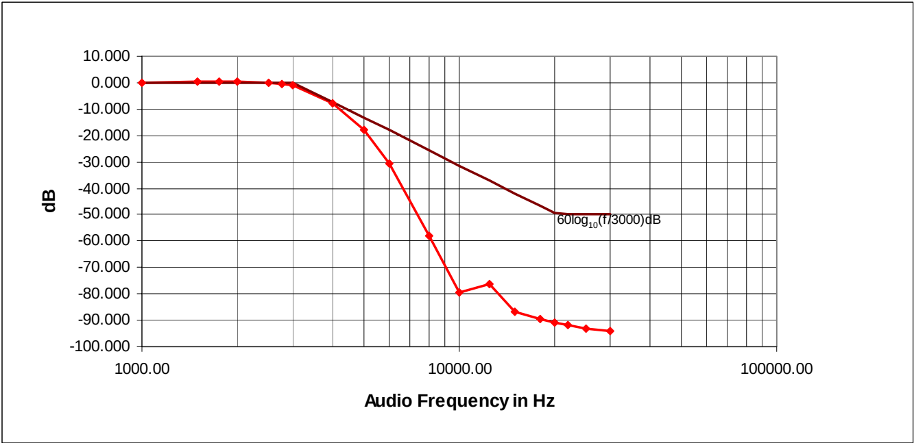
Figure 6C-2: 20 kHz Channel Spacing, Transmit Audio Post Limiter Lowpass Filter Response
