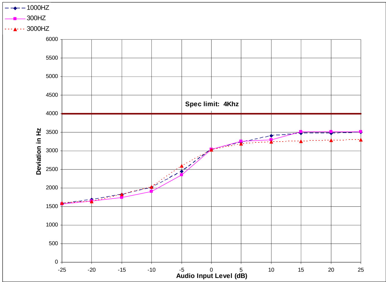
Figure 6D-6: 20 kHz Channel Spacing, Digital Private Line (DPL) Mode
