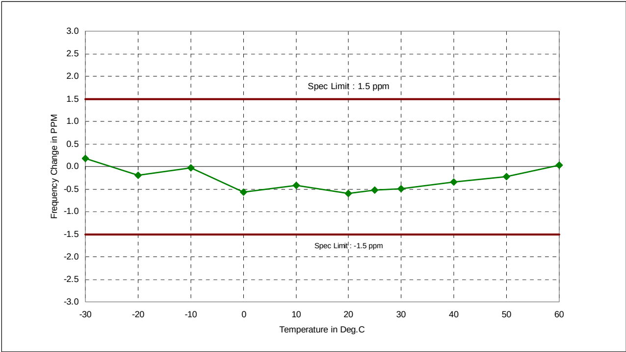
Figure 6H-1: Frequency Stability vs. Temperature
