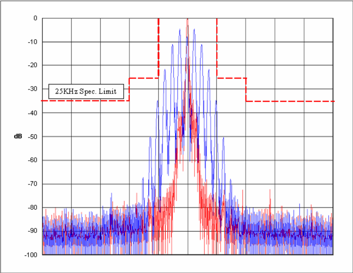
Figure 6E-3: Mask B; 25 kHz Channel Spacing, 2500 Hz Audio and DPL Tone Modulation; 16K0F3E
