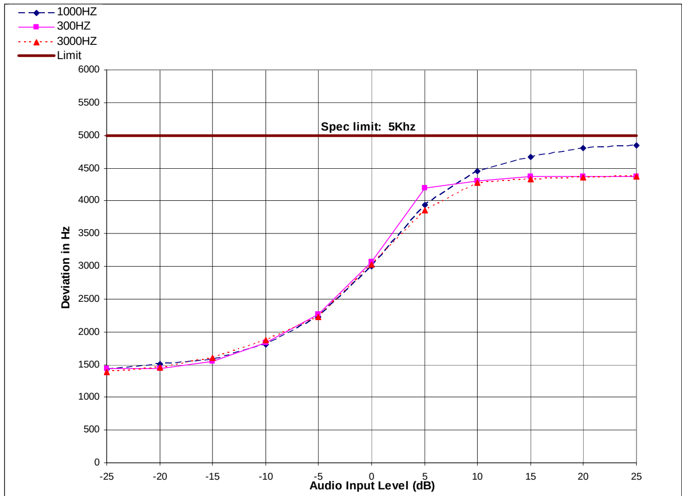
Figure 6D-1: 25 kHz Channel Spacing, Carrier Squelch Mode
