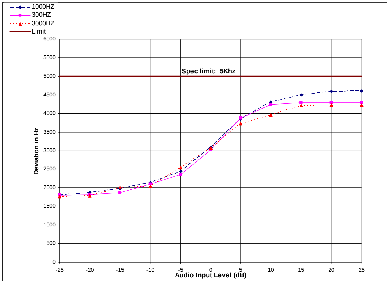
Figure 6D-3: 25 kHz Channel Spacing, Digital Private Line (DPL) Mode
