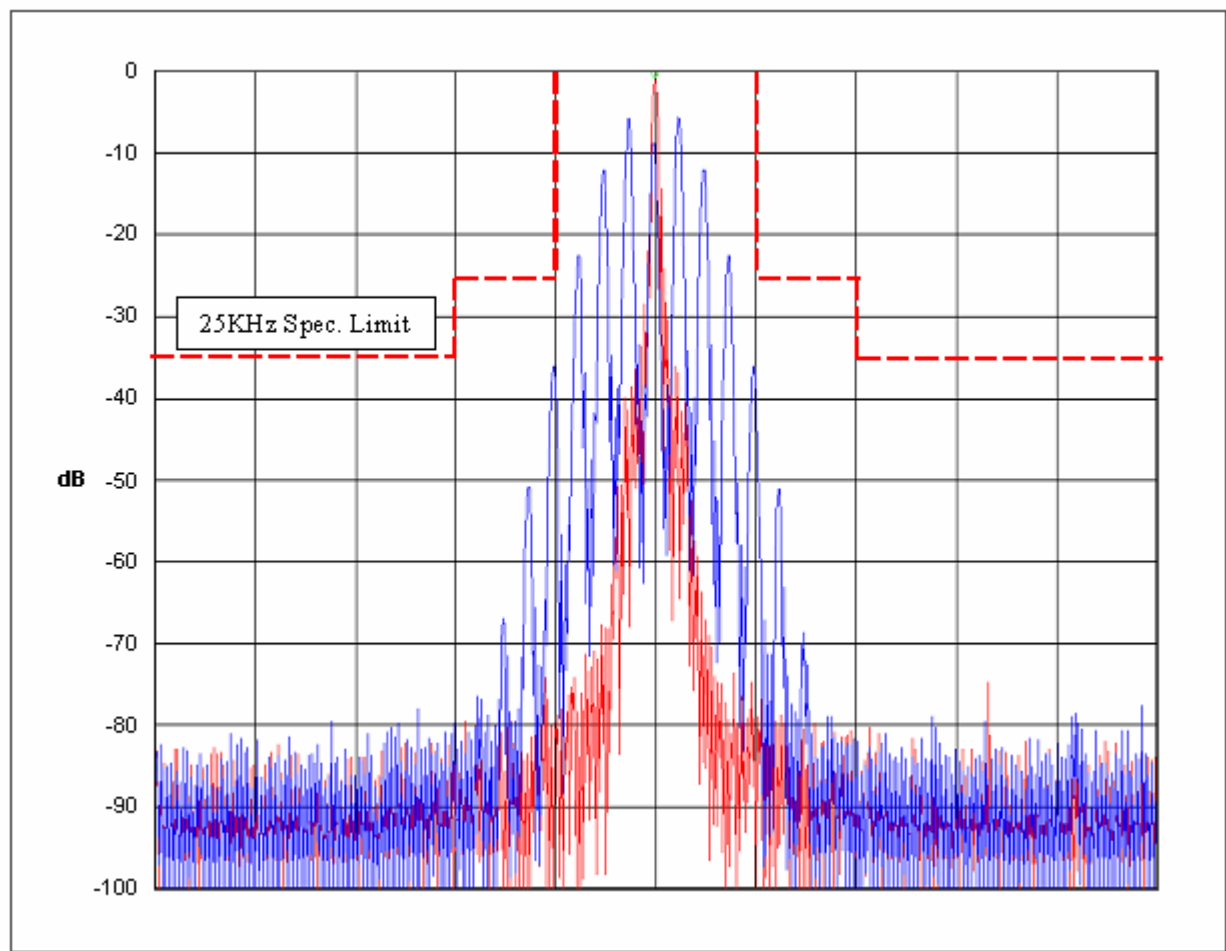
Figure 6E-1: Mask B; 25 kHz Channel Spacing, 2500 Hz Audio Modulation Only; 16K0F3E
