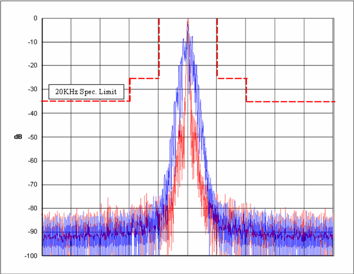
Figure 6E-10: Mask B; 20 kHz Channel Spacing, DTMF Modulation Only; 16K0F3E
