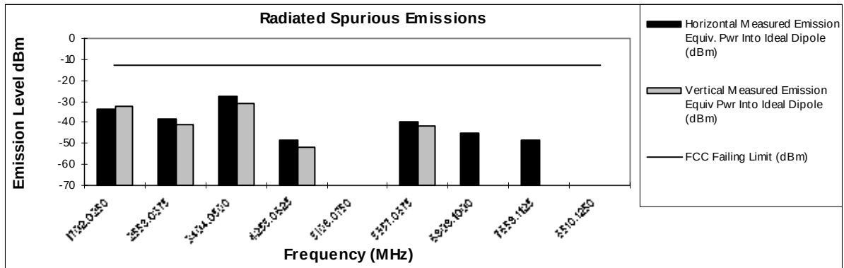
Figure 6G-4: 2 Watts, 851.0125 MHz
