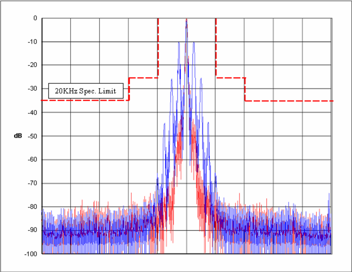
Figure 6E-9: Mask B; 20 kHz Channel Spacing, 2500 Hz Audio and DPL Tone Modulation; 16K0F3E
