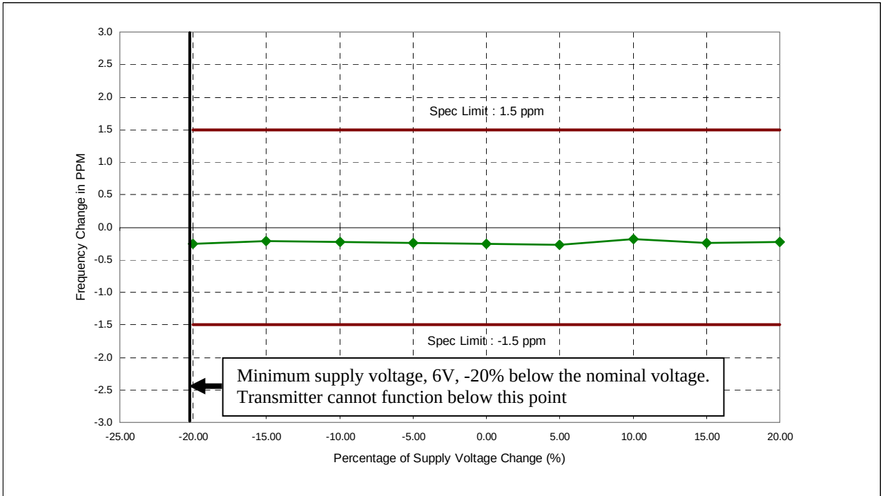
Figure 6H-2: Frequency Stability vs. Voltage
