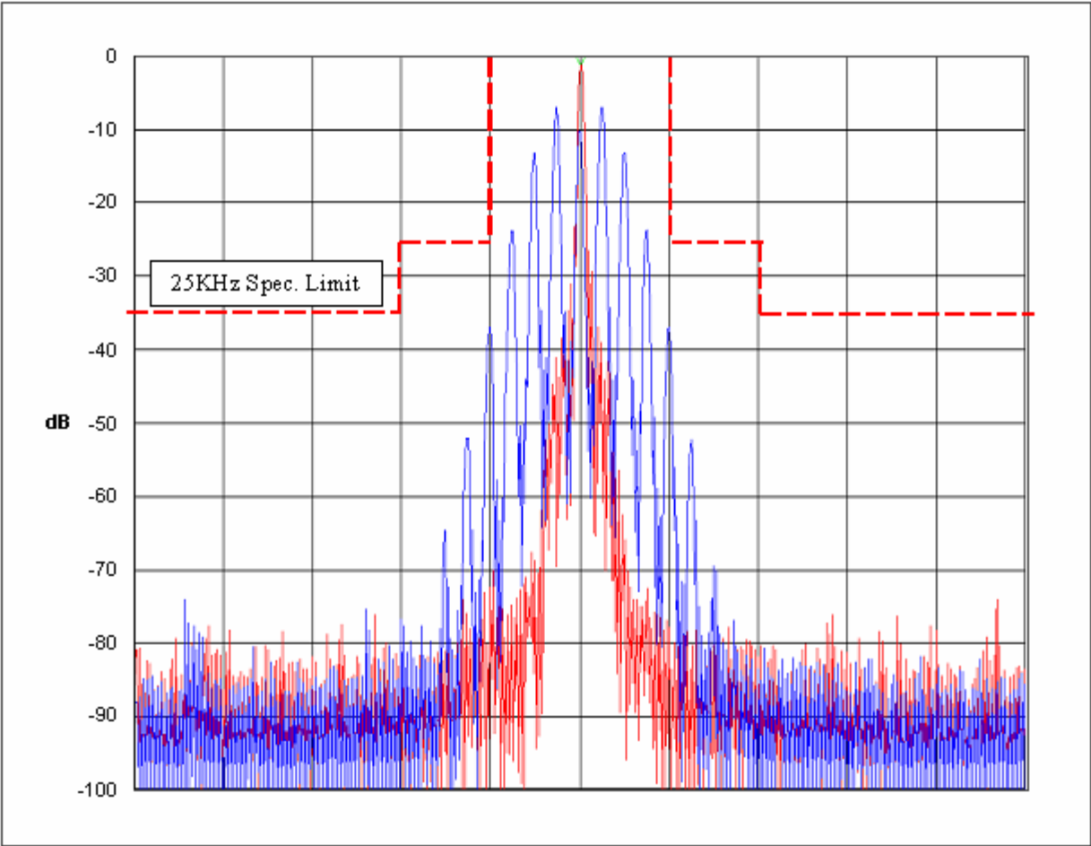
Figure 6E-2: Mask B; 25 kHz Channel Spacing, 2500 Hz Audio and TPL Tone Modulation; 16K0F3E
