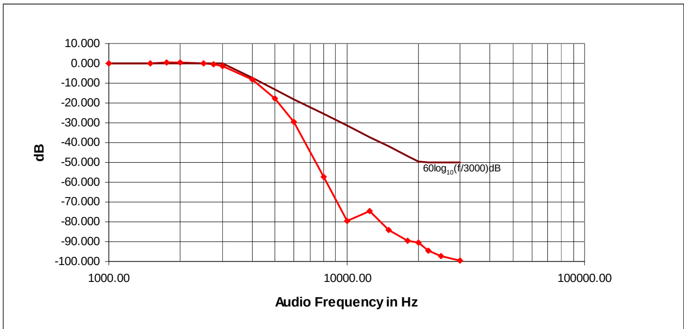
Figure 6C-1: 25 kHz Channel Spacing, Transmit Audio Post Limiter Lowpass Filter Response
