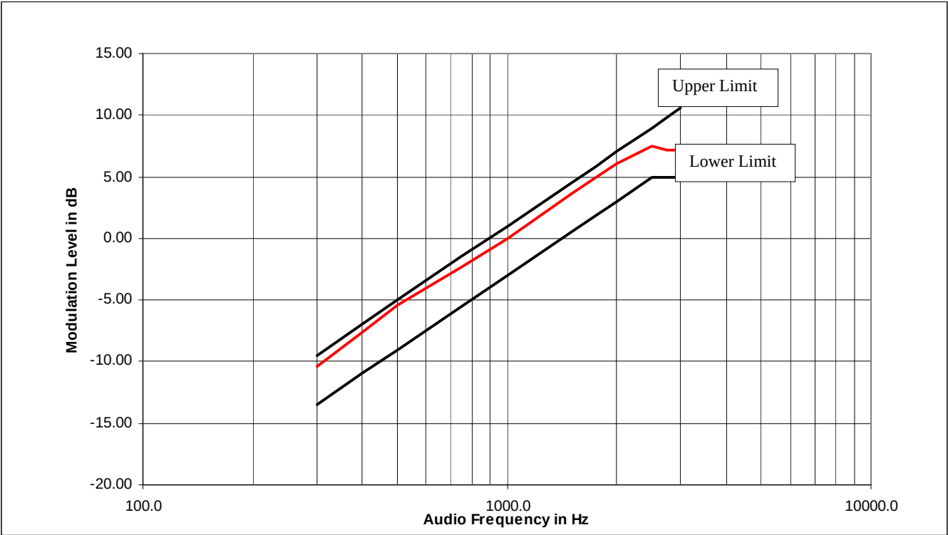
Figure 6B-1: 25 kHz Channel Spacing, Transmit Audio Response
