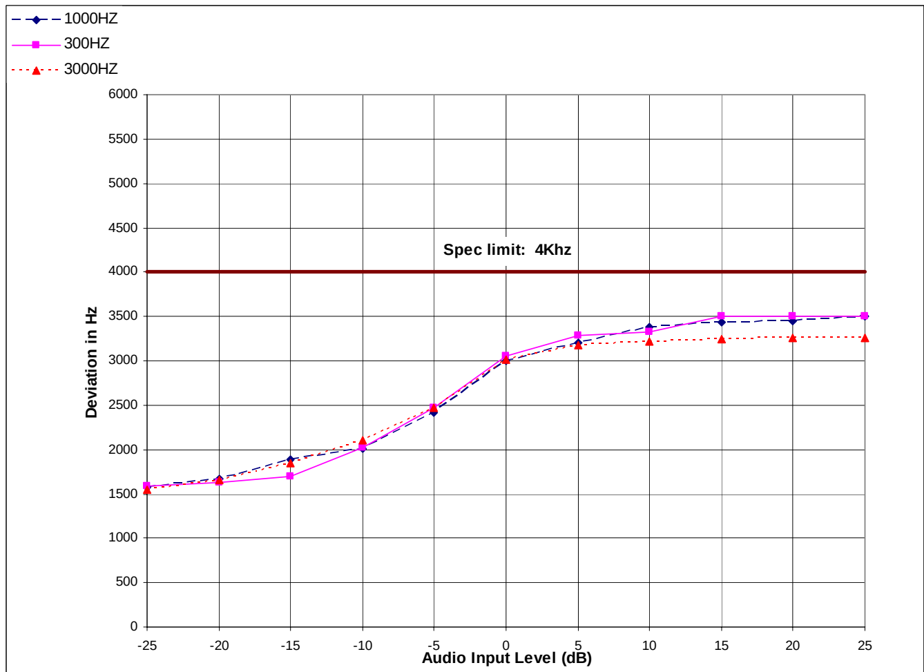
Figure 6D-5: 20 kHz Channel Spacing, Tone Private Line (TPL) Mode
