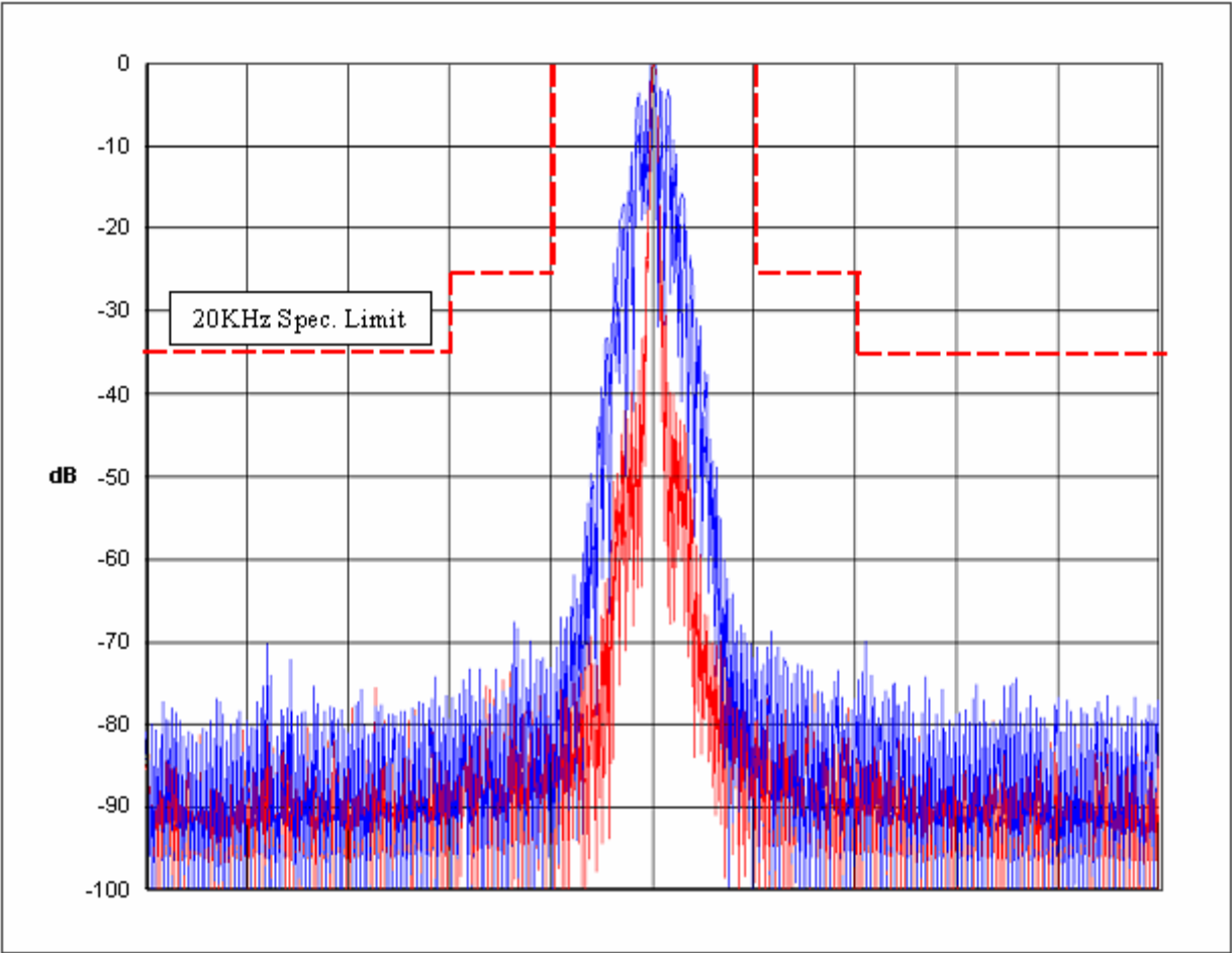
Figure 6E-11: Mask B; 20 kHz Channel Spacing, DTMF Modulation and TPL Tone Modulation; 16K0F3E
