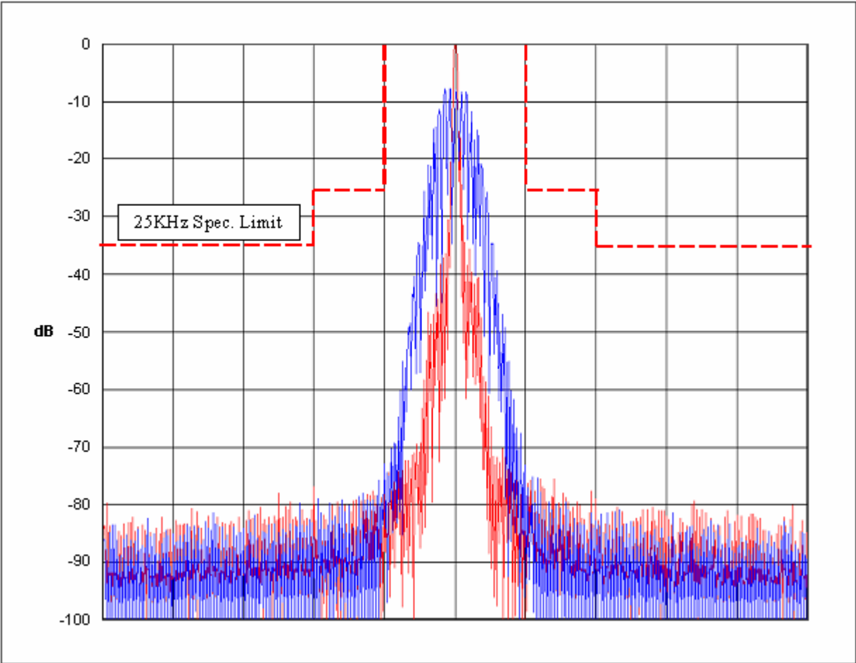
Figure 6E-4: Mask B; 25 kHz Channel Spacing, DTMF Modulation Only; 16K0F3E
