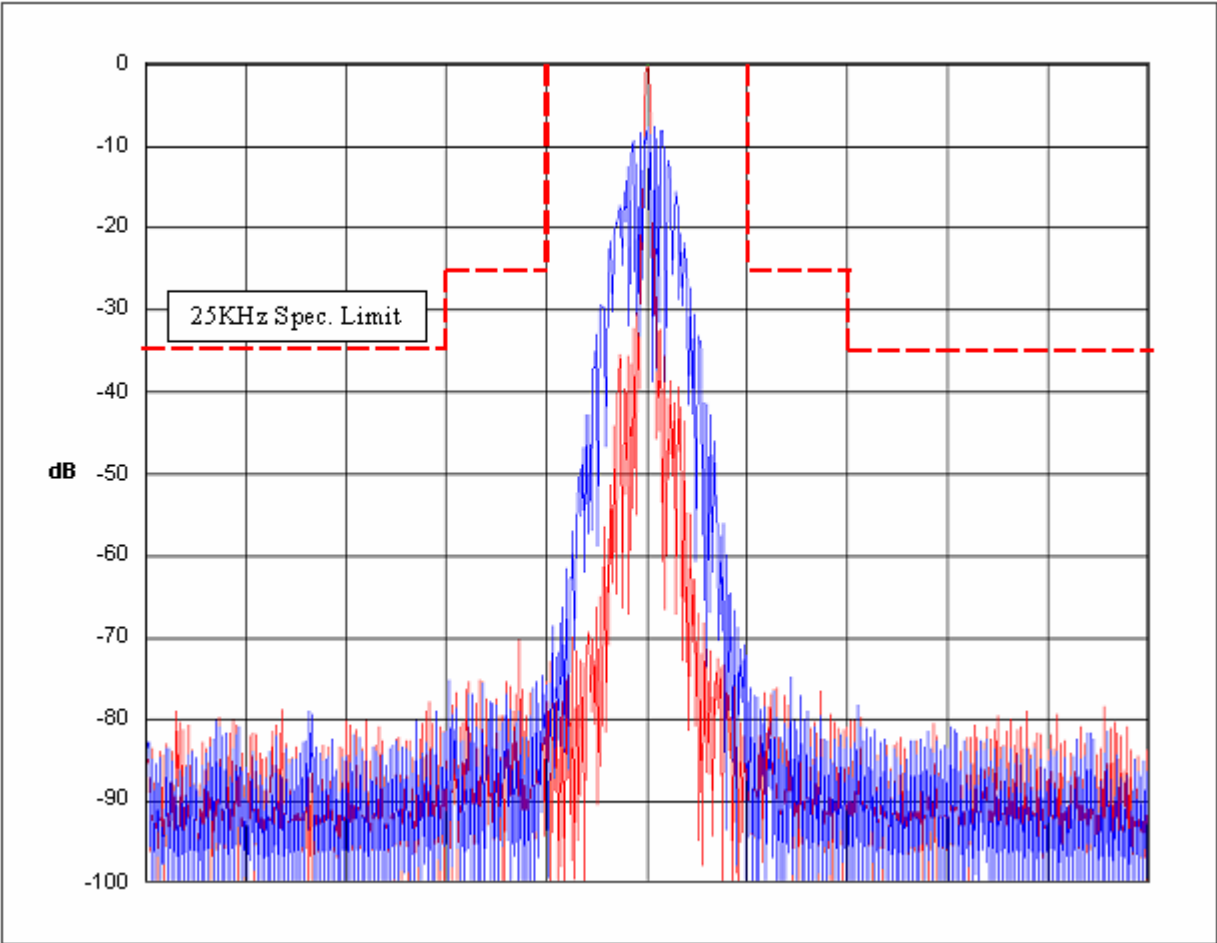
Figure 6E-6: Mask B; 25 kHz Channel Spacing, DTMF Modulation and DPL Tone Modulation; 16K0F3E
