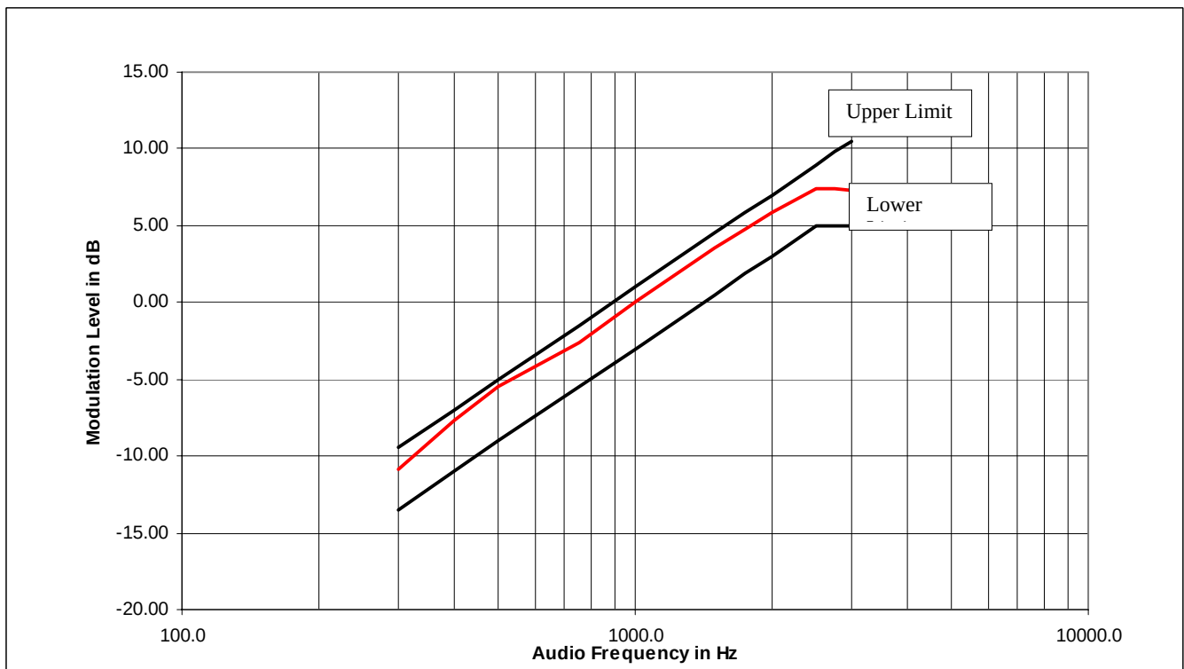
Figure 6B-2: 20 kHz Channel Spacing, Transmit Audio Response
