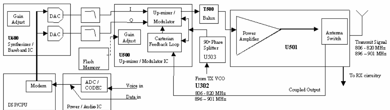
Figure 4-2: Transmitter Modulation System/Line-up System
