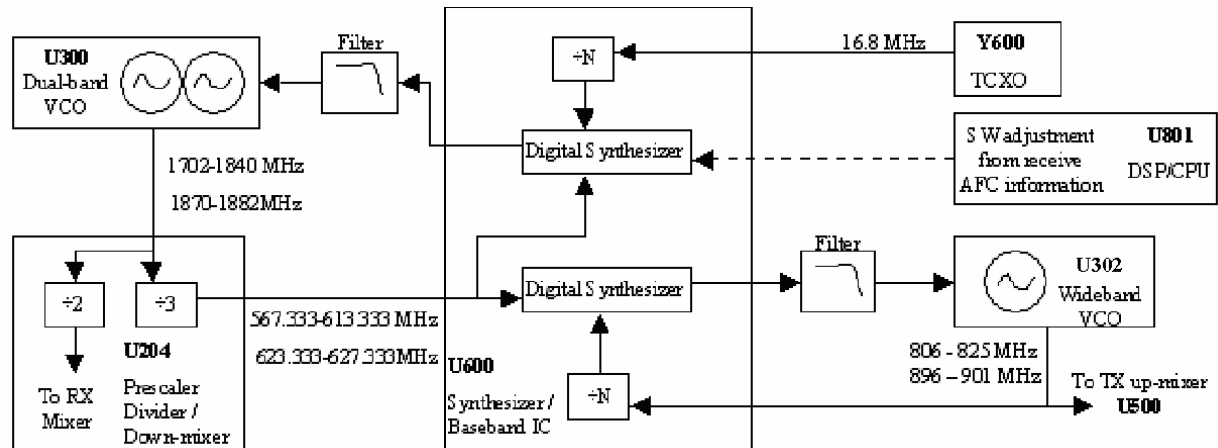
Figure 4-1: Frequency Generation Block Diagram
