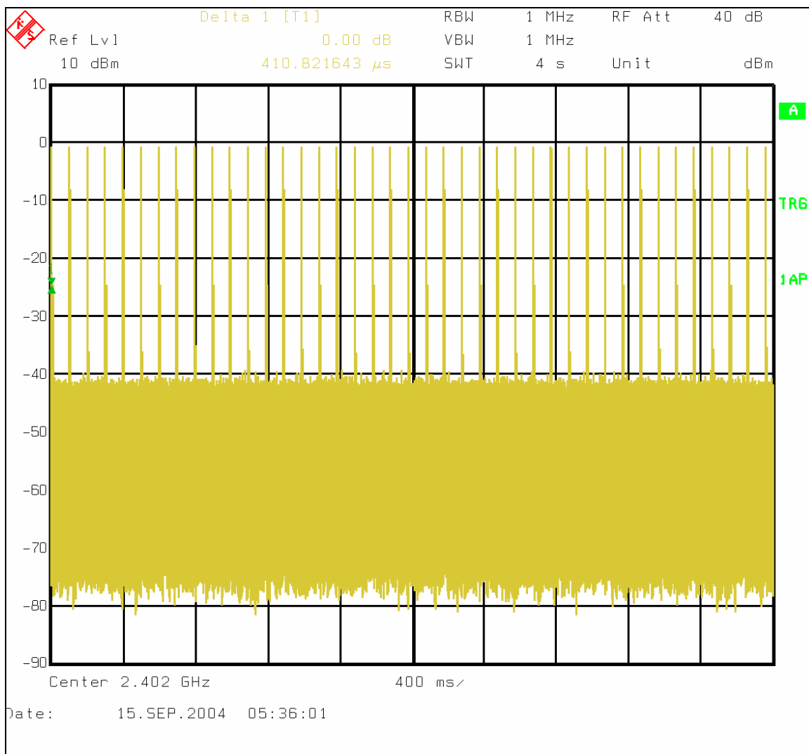
Figure 6-41: Plot of dwell time over 4 second period
