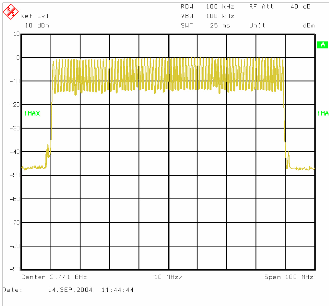
Figure 6-39: Plot of number of Bluetooth hopping frequencies
