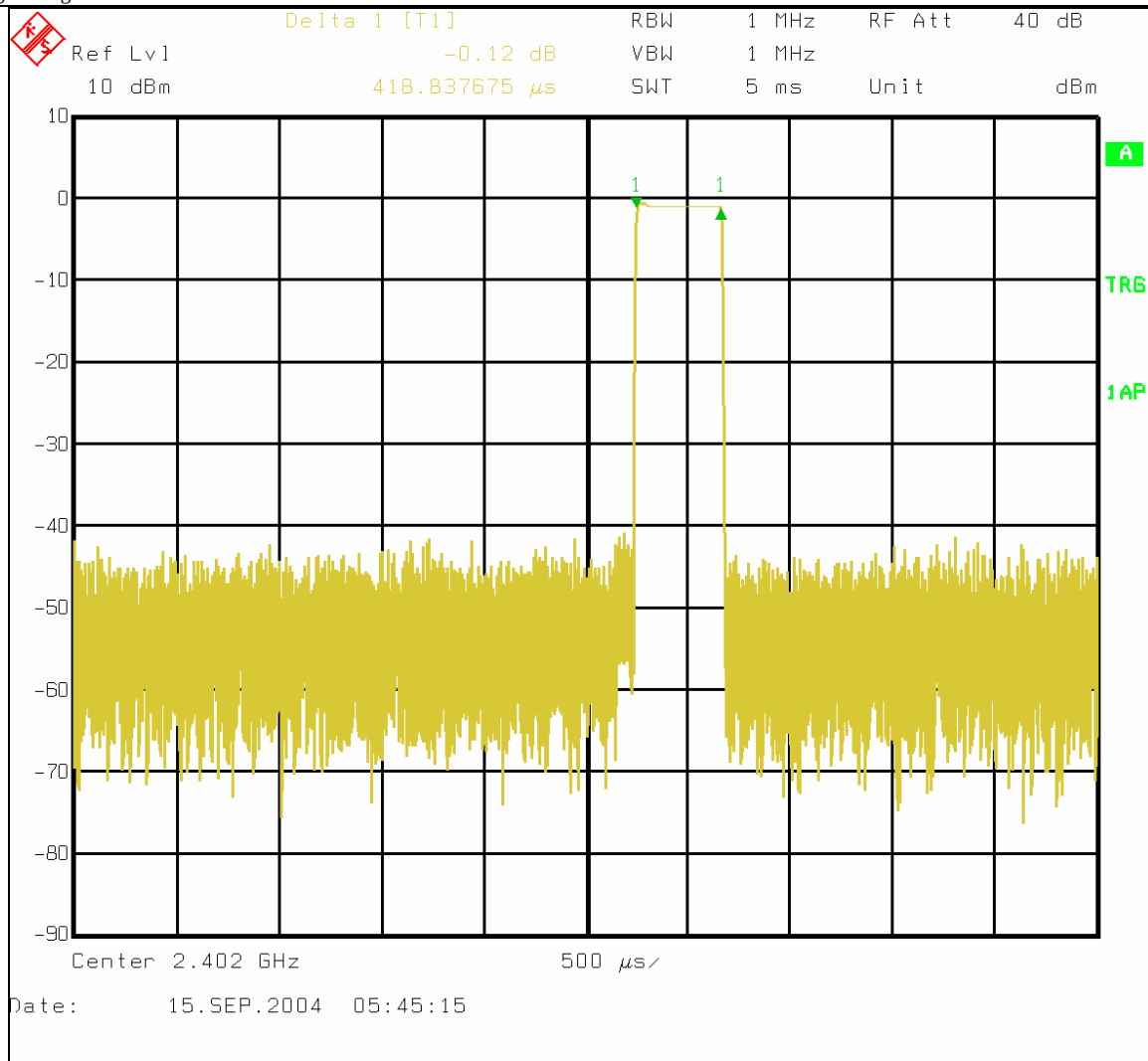
Figure 6-42: Plot of dwell time over 5 mili-second period
