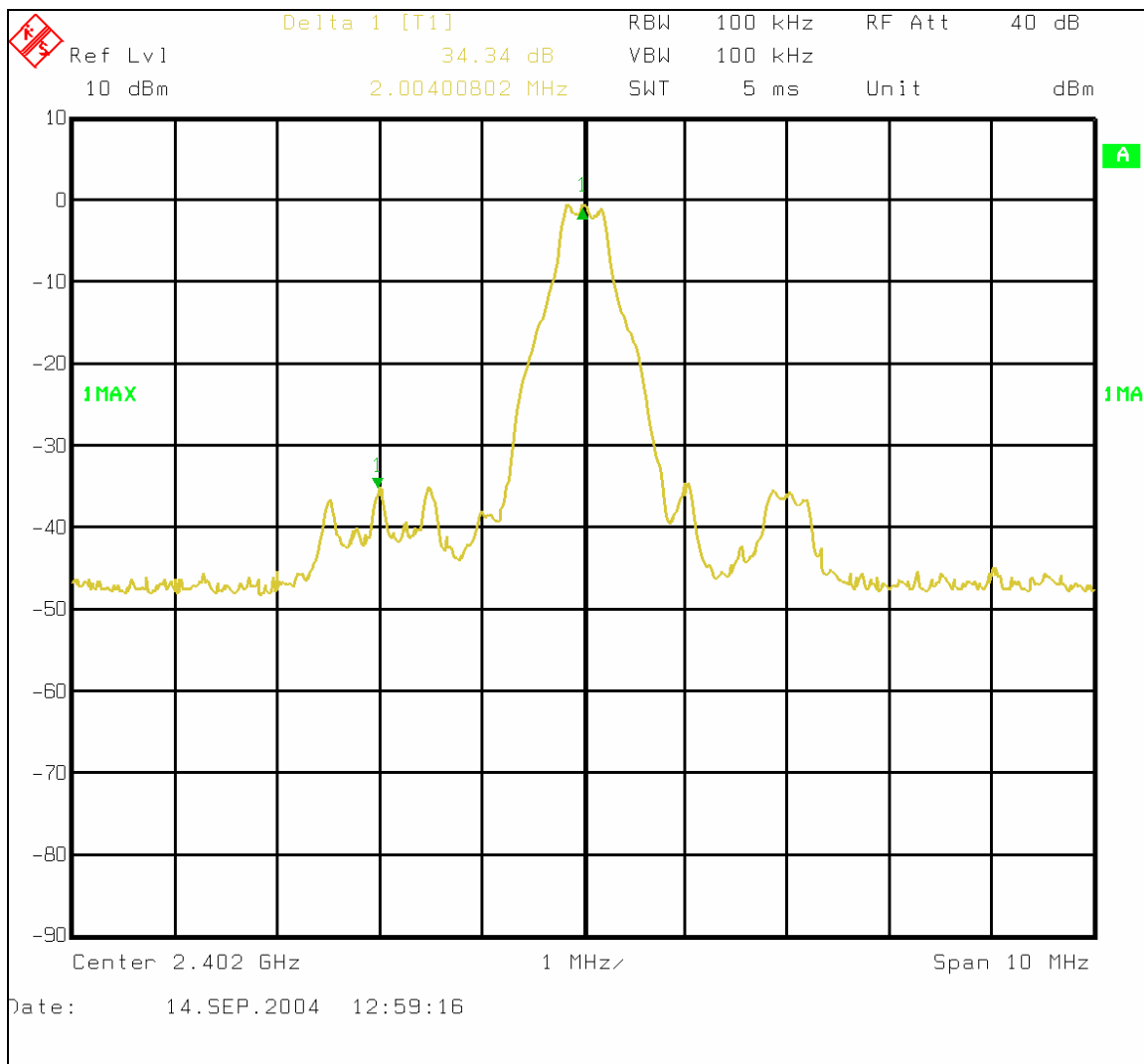
Figure 6-45: Plot of lower band-edge conducted emissions with hopping disabled
