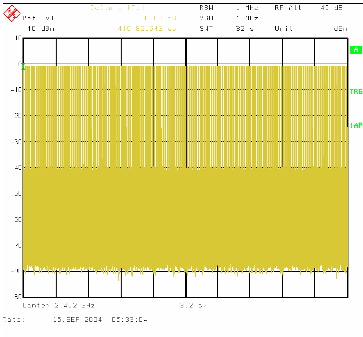
Figure 6-40: Plot of dwell time over 32 second period
