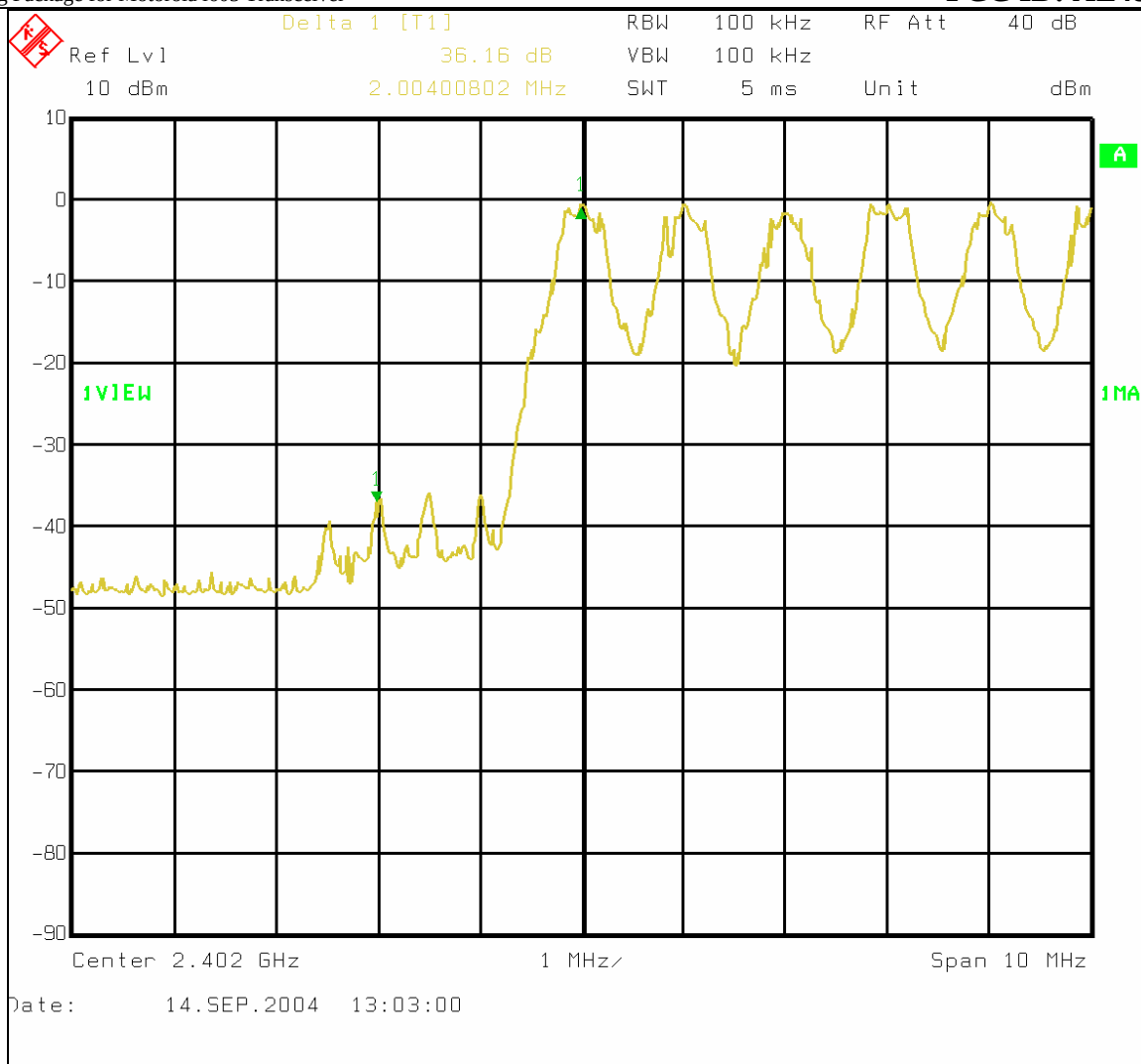
Figure 6-47: Plot of lower band-edge conducted emissions with hopping enabled
