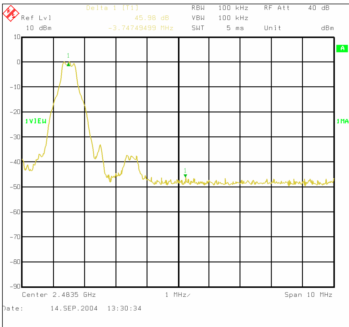
Figure 6-46: Plot of upper band-edge conducted emissions with hopping disabled
