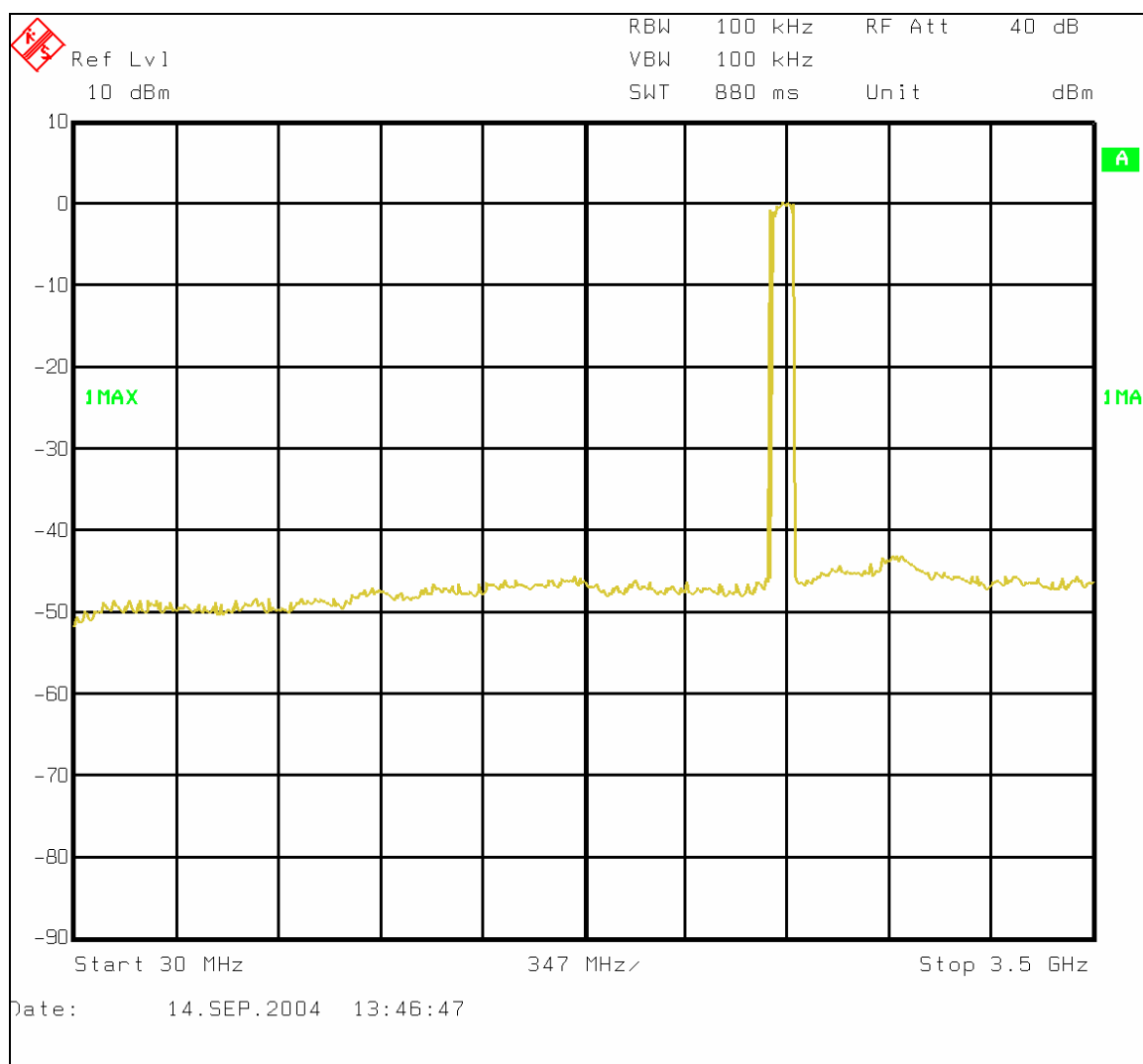
Figure 6-49: Plot of spurious conducted emissions 30 MHz – 3.5 GHz
