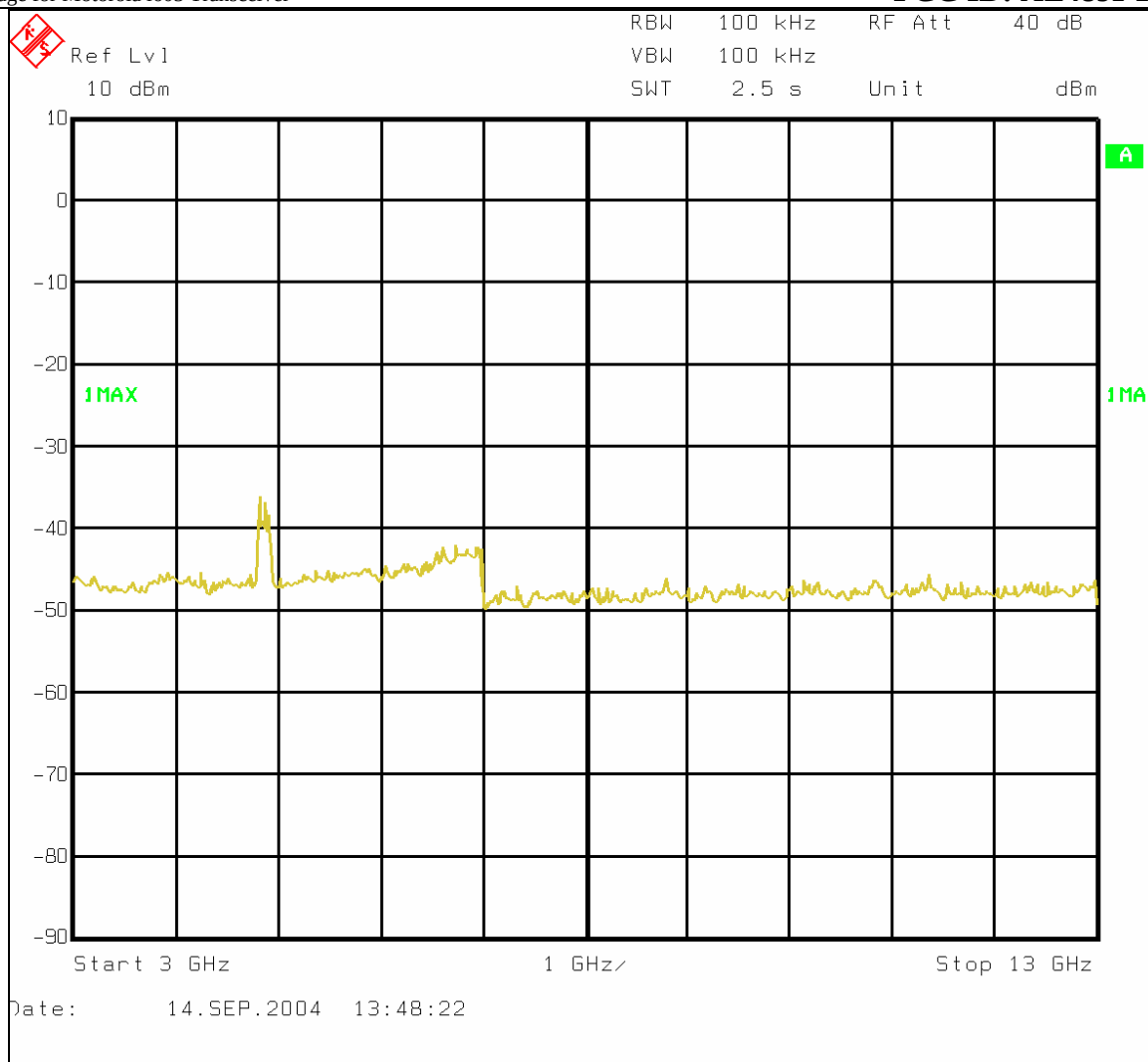
Figure 6-50: Plot of spurious conducted emissions 3 GHz – 13 GHz
