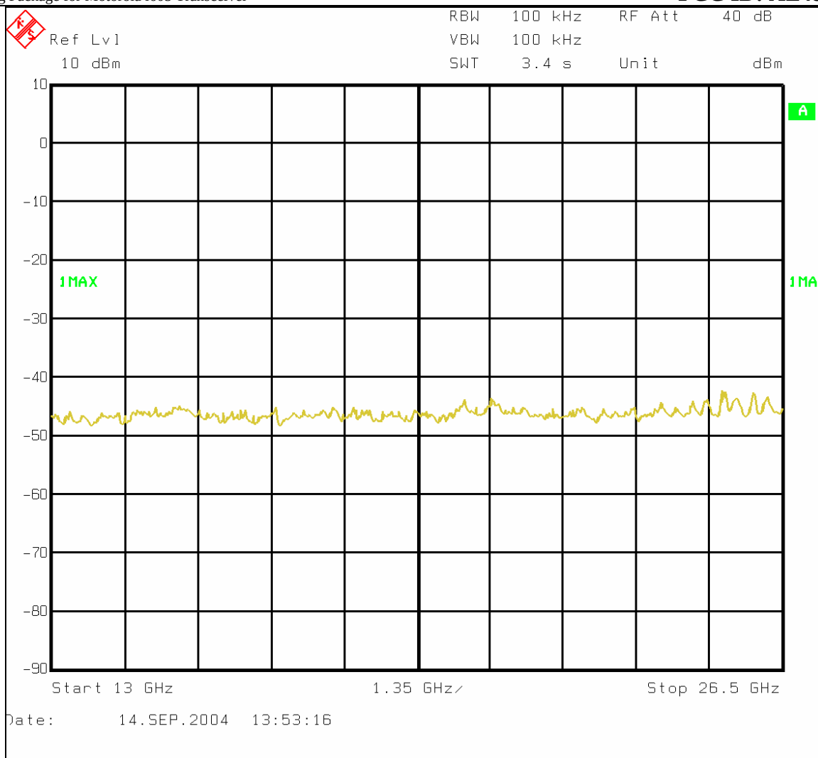
Figure 6-51: Plot of spurious conducted emissions 13 GHz – 26.5 GHz
