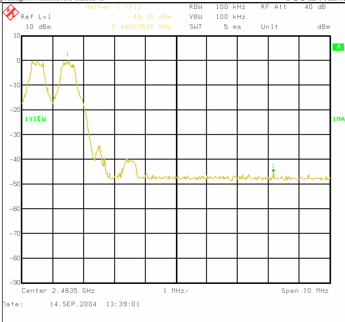
Figure 6-48: Plot of upper band-edge conducted emissions with hopping enabled
