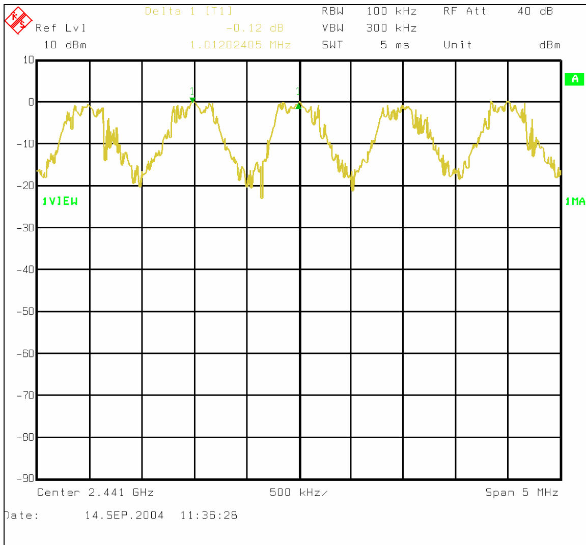
Figure 6-38: Plot of Bluetooth carrier frequency separation
