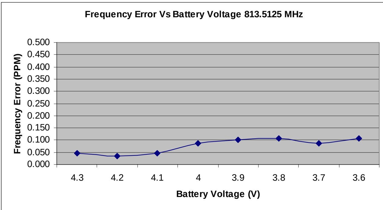
Figure 6-33: Transmitter Frequency Stability (800 MHz band) - Frequency Error vs. Battery Voltage
