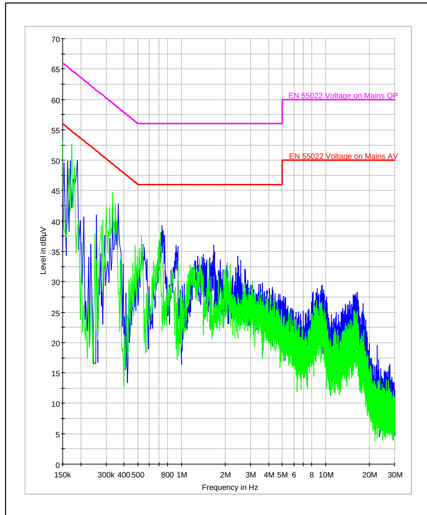
Figure 6-36: Neutral Line Voltage with a Peak and Average detector (Radio in receive mode at 851.0625 MHz)
