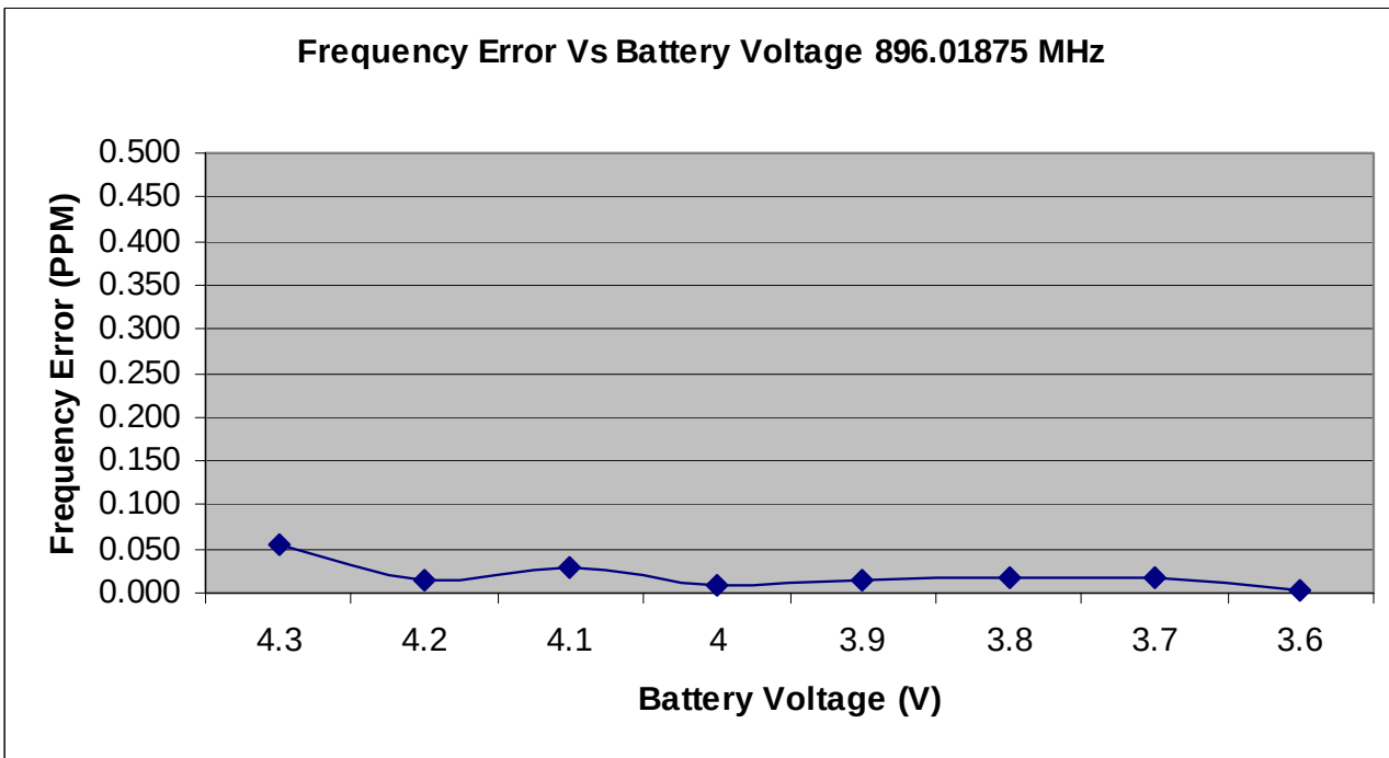
Figure 6-34: Transmitter Frequency Stability (900 MHz band)- Frequency Error vs. Battery Voltage
