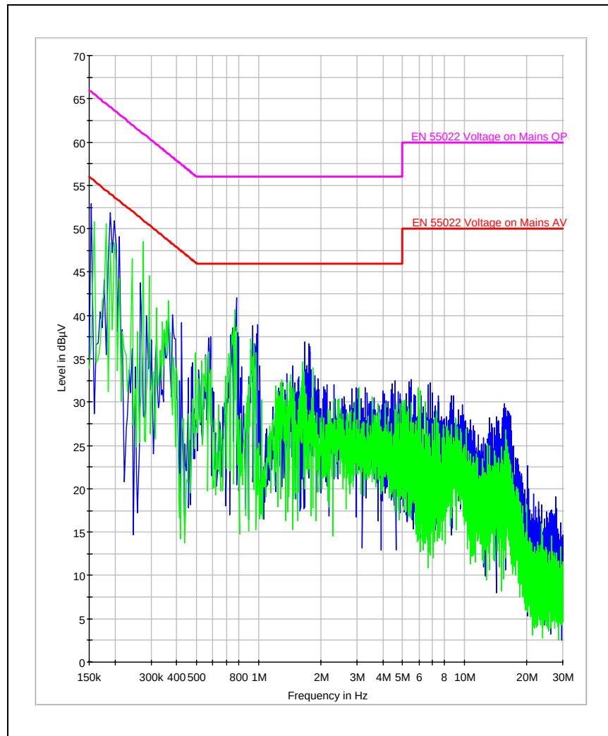
Figure 6-35: Phase Line Voltage with a Peak and Average Detector (Radio in transmit mode at 806.0625 MHz)
