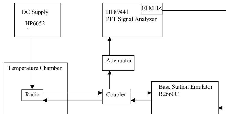
Figure 7-1: Transmit Frequency Measurement Setup
