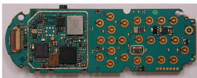
Photograph 9.4: Front side view of radio PCB without shields.
