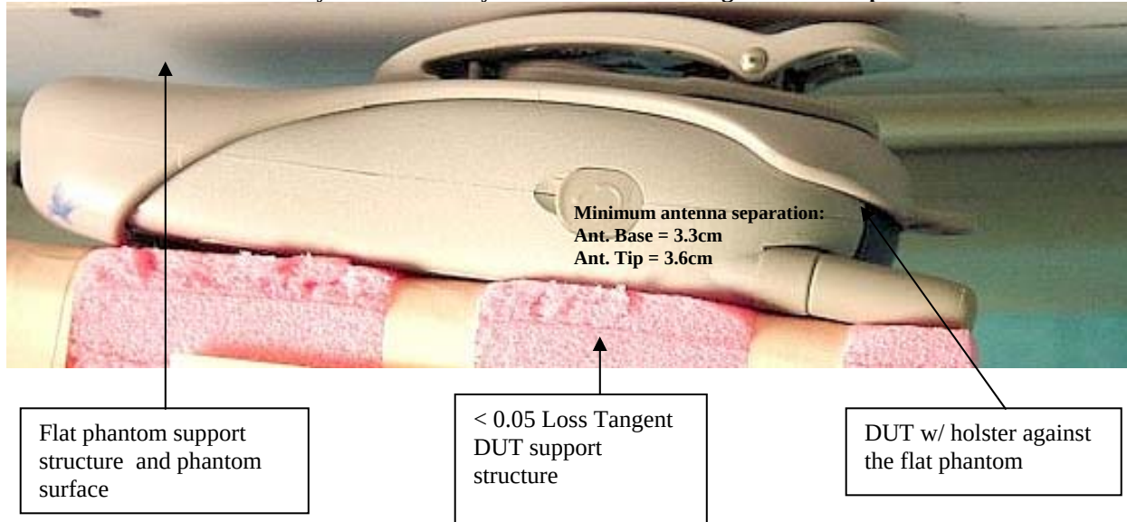
Figure 1: Highest S.A.R. Test Position (@ body) DUT with body worn accessory model NNTN5845A against the flat phantom.
