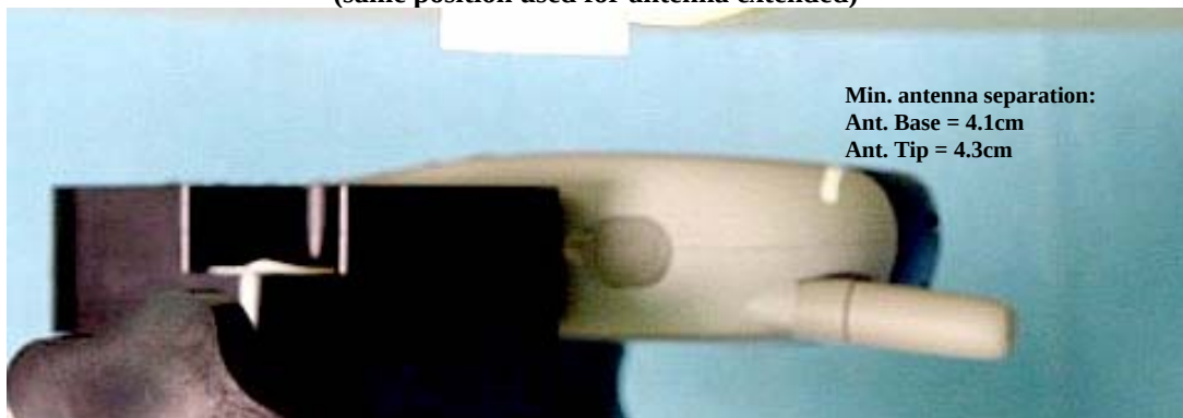
Figure 8. Assessment @ Face DUT front 2.5cm separation distance from flat phantom. (same position used for antenna extended)
