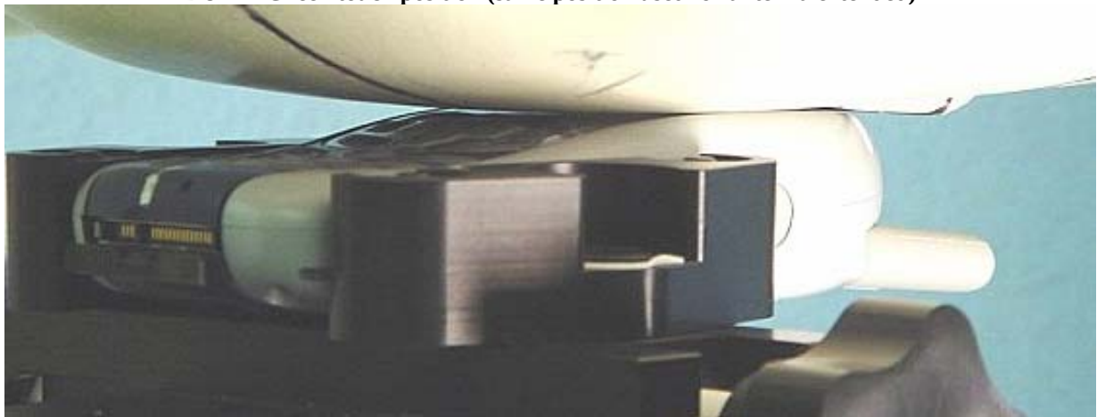
Figure 2. Assessment @ the Left ear DUT in Cheek touch position (same position used for antenna extended)
