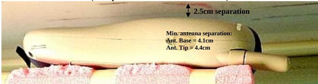
Figure 7. Assessment @ the body DUT back 2.5cm separation distance from flat phantom. (same position used for antenna extended)
