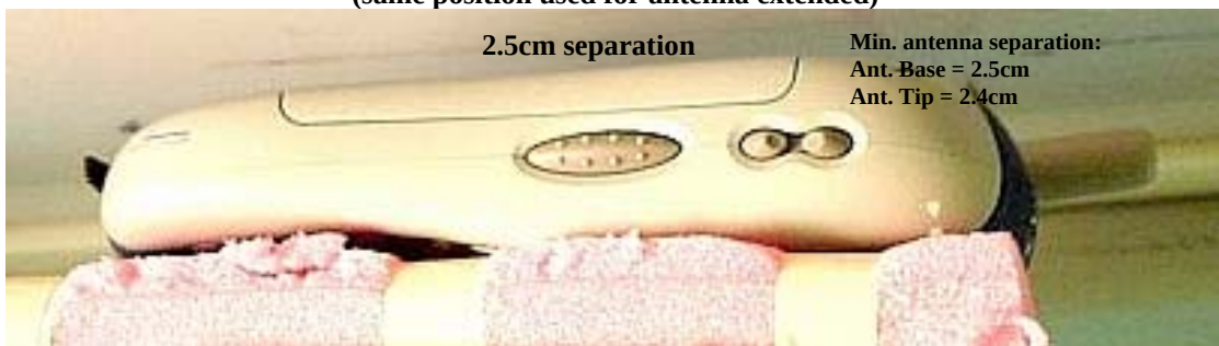
Figure 8. Assessment @ Face DUT front 2.5cm separation distance from flat phantom. (same position used for antenna extended)
