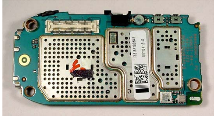
Figure 9-2. Main assembly – side 2.
