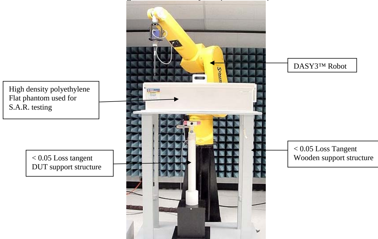
Figure 11: Robot Test System (Flat Phantom)
