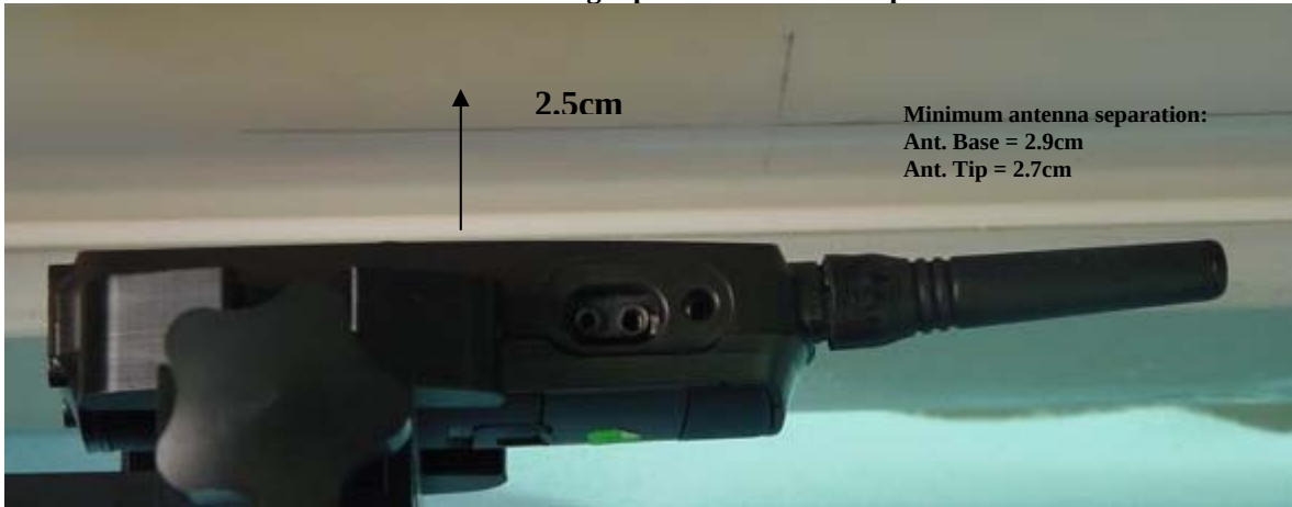
Figure 1. Highest S.A.R. Test Position (@ Face) DUT with front housing separated 2.5cm from phantom
