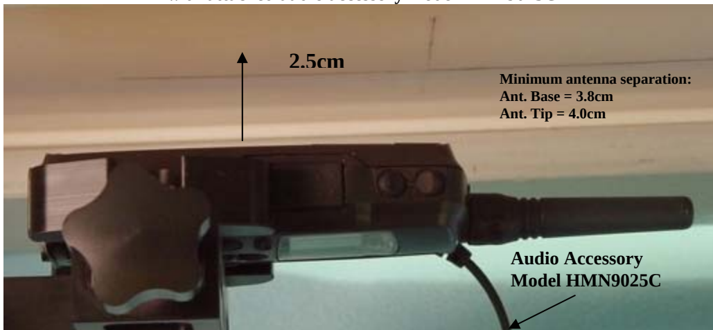
Figure 4. Assessment @ body DUT with back separated 2.5cm from phantom with attached audio accessory model HMN9025C
