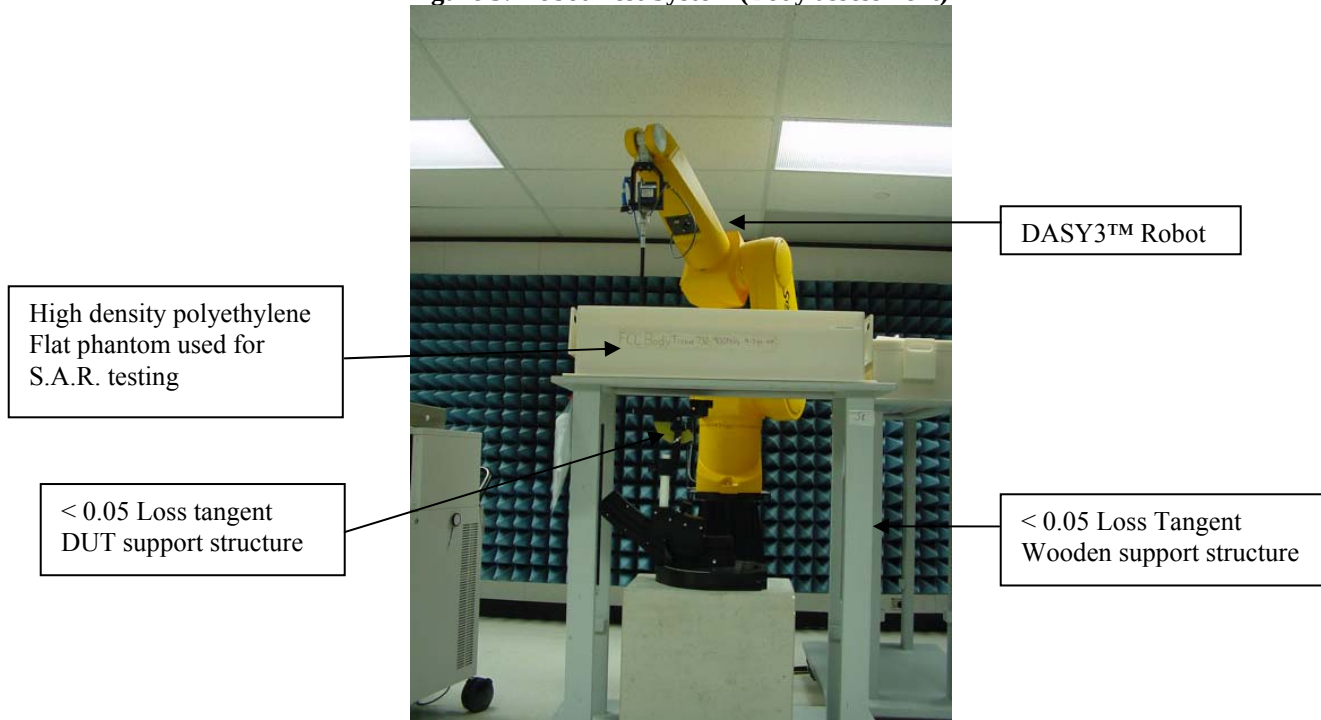
Figure 6: Robot Test System (Face assessment)
