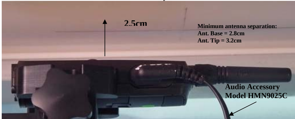
Figure 3. Assessment @ body DUT with front separated 2.5cm from phantom with attached audio accessory model HMN9025C
