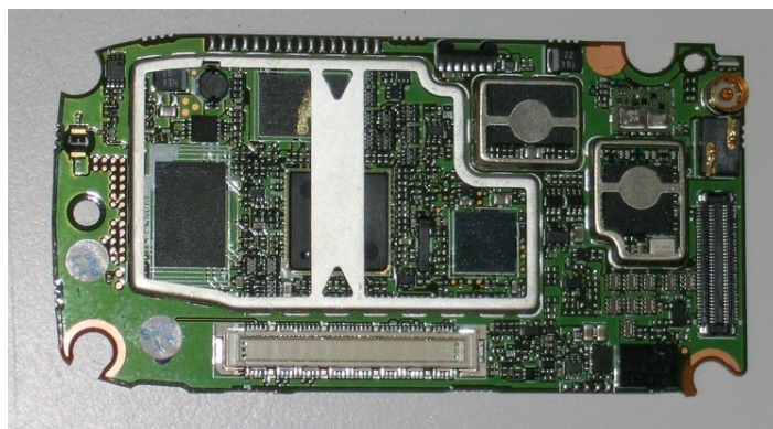
Photograph 9-6: Back side view of radio PCB2 without shields.
