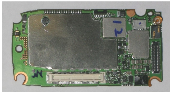
Photograph 9-5: Back side view of radio product PCB2.
