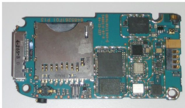
Photograph 9-2: Back side view of radio PCB1 without shields.
