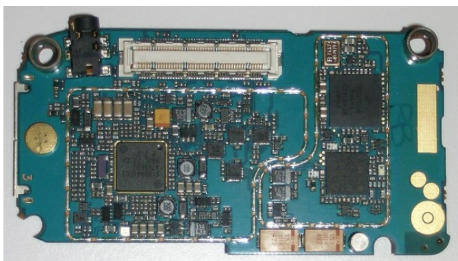
Photograph 9-4: Front side view of radio PCB1 without shields.
