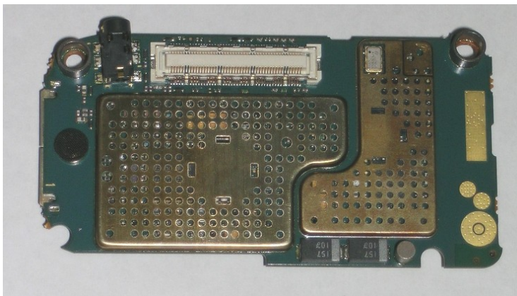
Photograph 9-3: Front side view of radio product PCB1.
