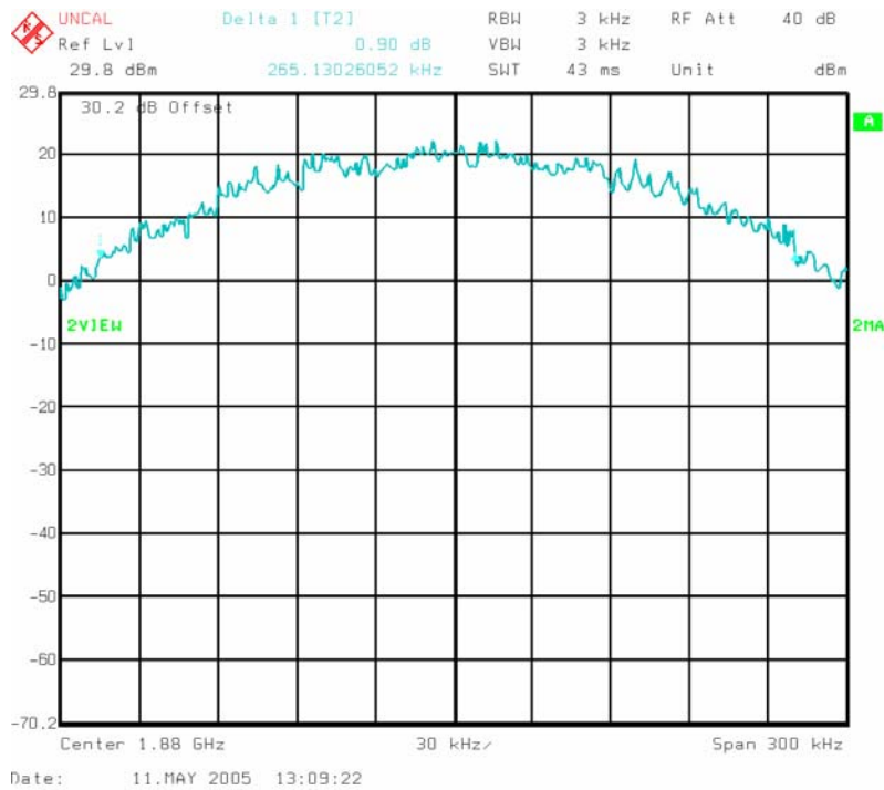
Figure 6-2. Occupied bandwidth
