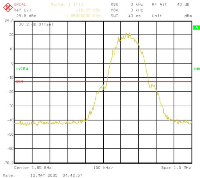
Figure 6-3. GSM/PCS 1900 Ch 512 Lower Band Edge
