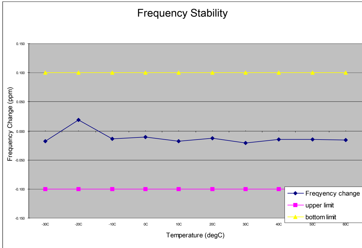
Figure 6-5. Frequency stability chart.
