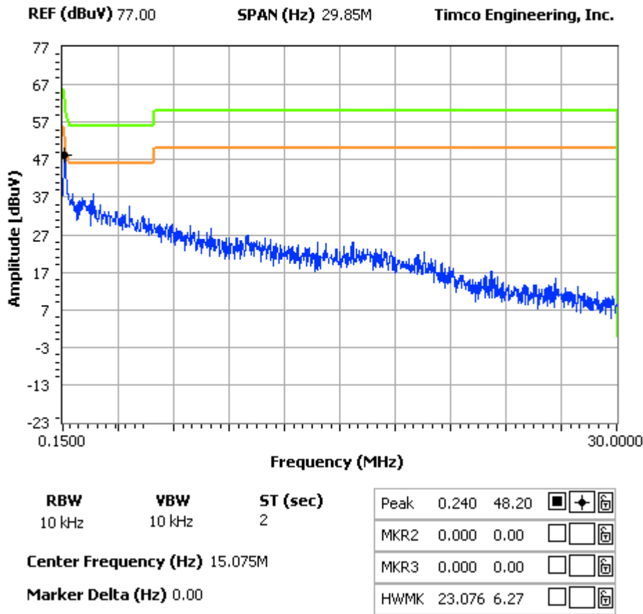
Figure 6-8. Mains Voltage with Peak and AverageDetector.
