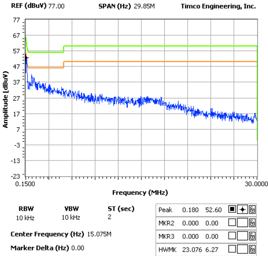
Figure 6-7. Mains Voltage with Peak and AverageDetector.
