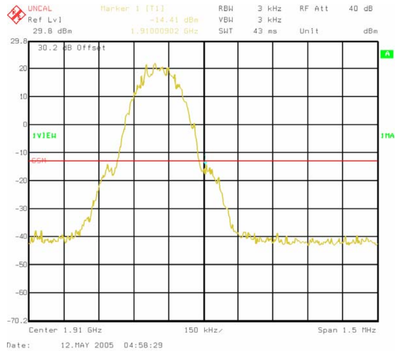
Figure 6-4. GSM/PCS 1900 Ch 810 Upper Band Edge
