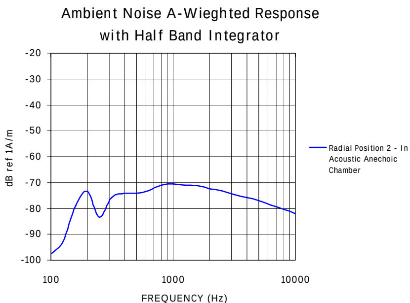
Figure 8-3 – Radial Position 2 Ambient Magnetic frequency distribution
