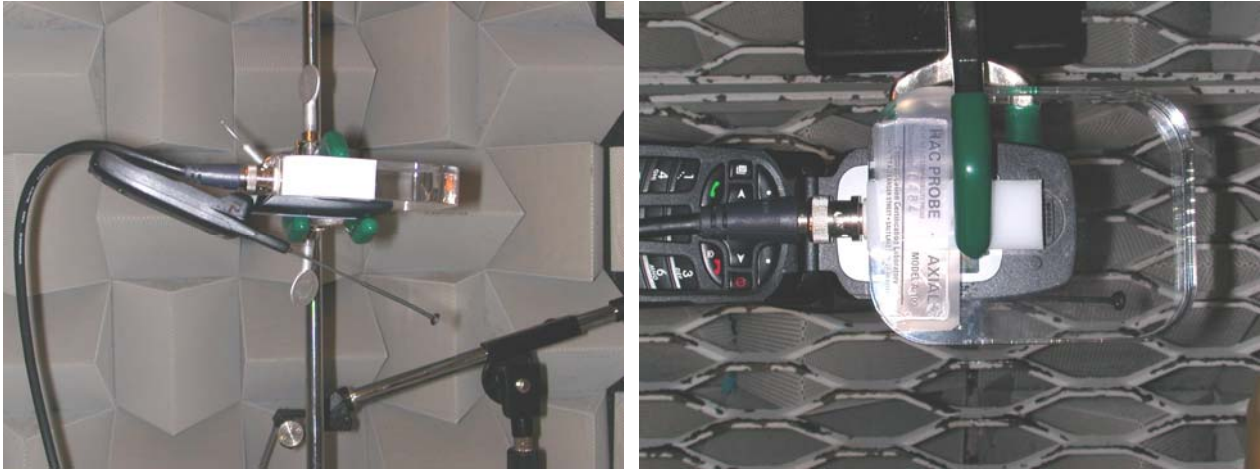
Figure 7-1 – Test holder
