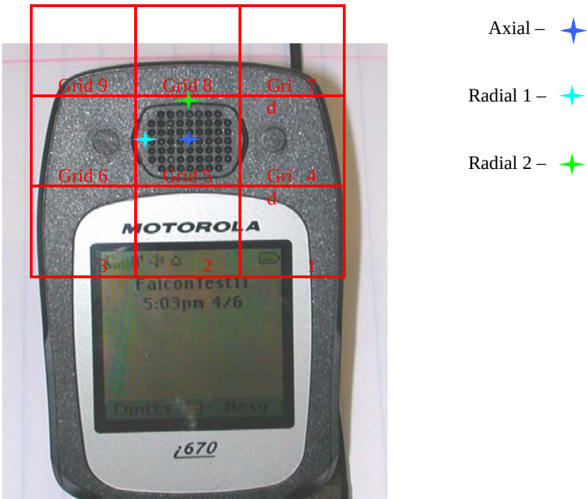
Figure 7-2 – Measurement location coordinates
