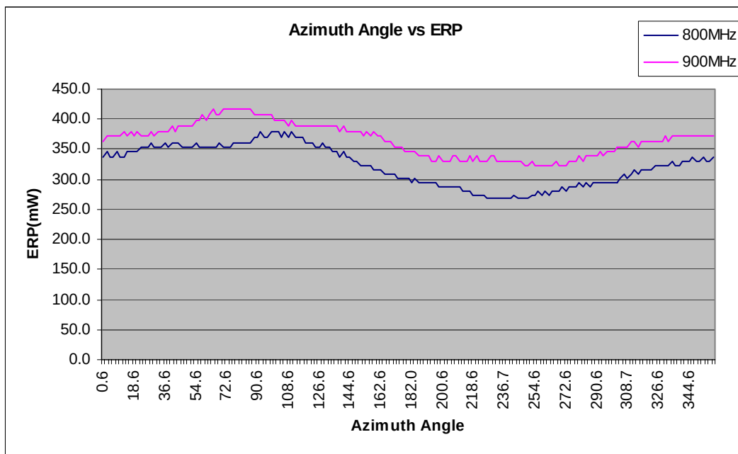
Figure 6a-94. Scaled ERP vs. Azimuth Angle
