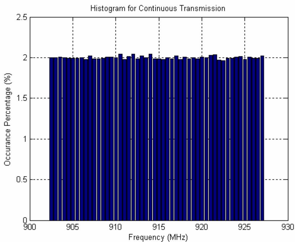
Figure 6b-9. Histogram for 900 MHz ISM Band Continuous Transmission
