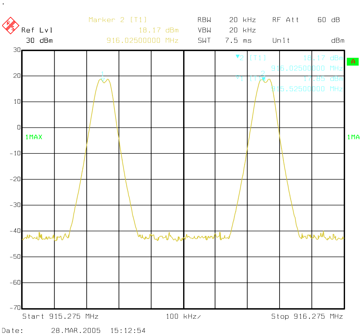
Figure 6b-5. Plot of 900 MHz ISM Band adjacent channel separation within a hops
