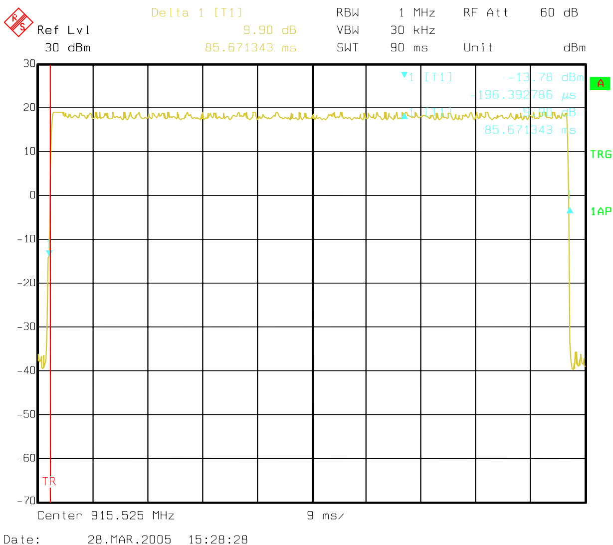
Figure 6b-8. 900 MHz ISM Band Average Measured Time of Occupancy.
