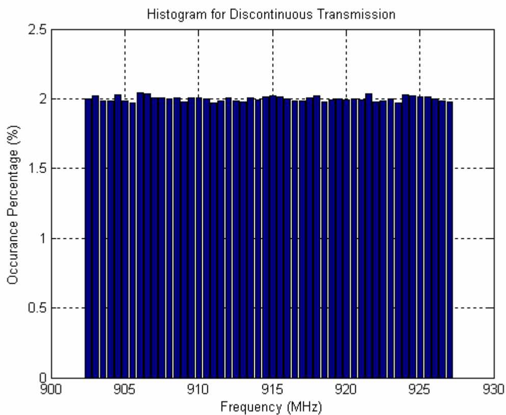
Figure 6b-10. Histogram for 900 MHz ISM Band Discontinuous Transmission
