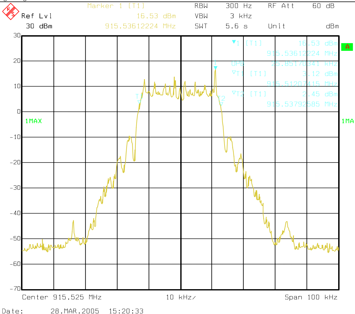
Figure 6b-6. Spectrum analyzer plot of 900 MHz ISM Band 8-FSK traffic channel signal's 99% Bandwidth
