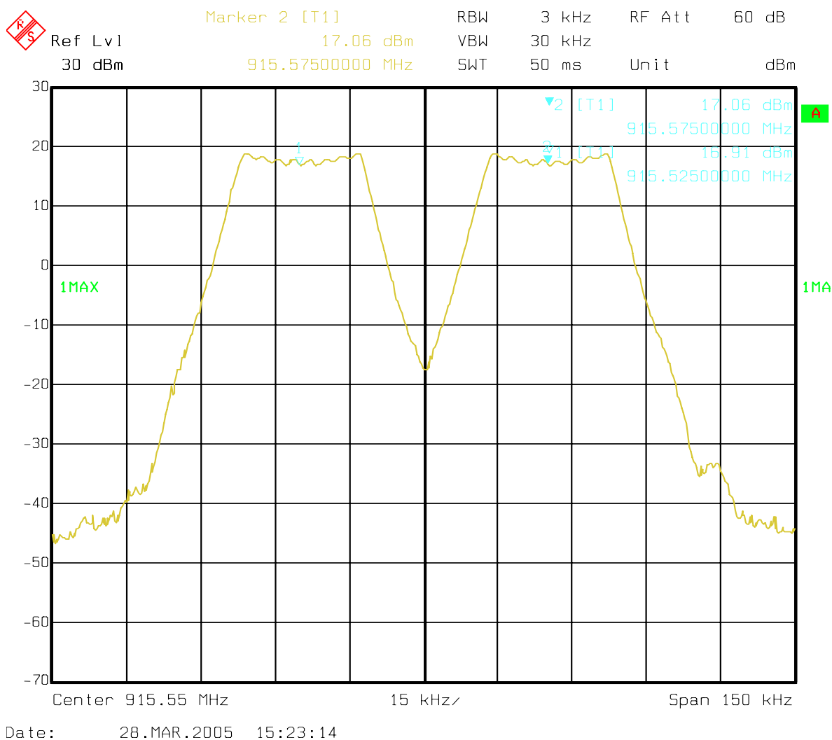
Figure 6b-7. Adjacent hopset separation.
