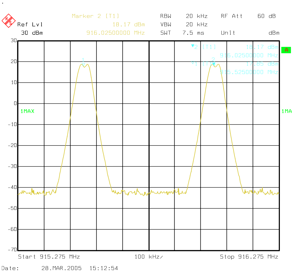
Figure 6b-5. Plot of 900 MHz ISM Band adjacent channel separation within a hopset.
