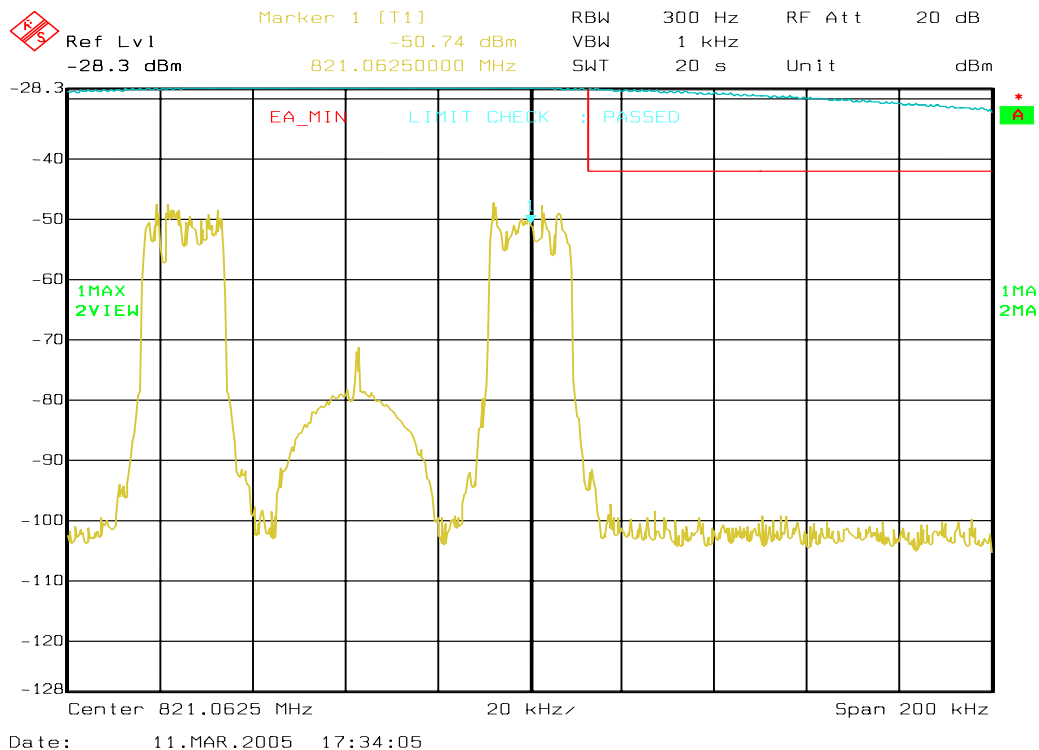
Figure 6a-57 . WiDEN_50_Split 800 MHz Band, QAM16, Minimum Power, EA Emission
