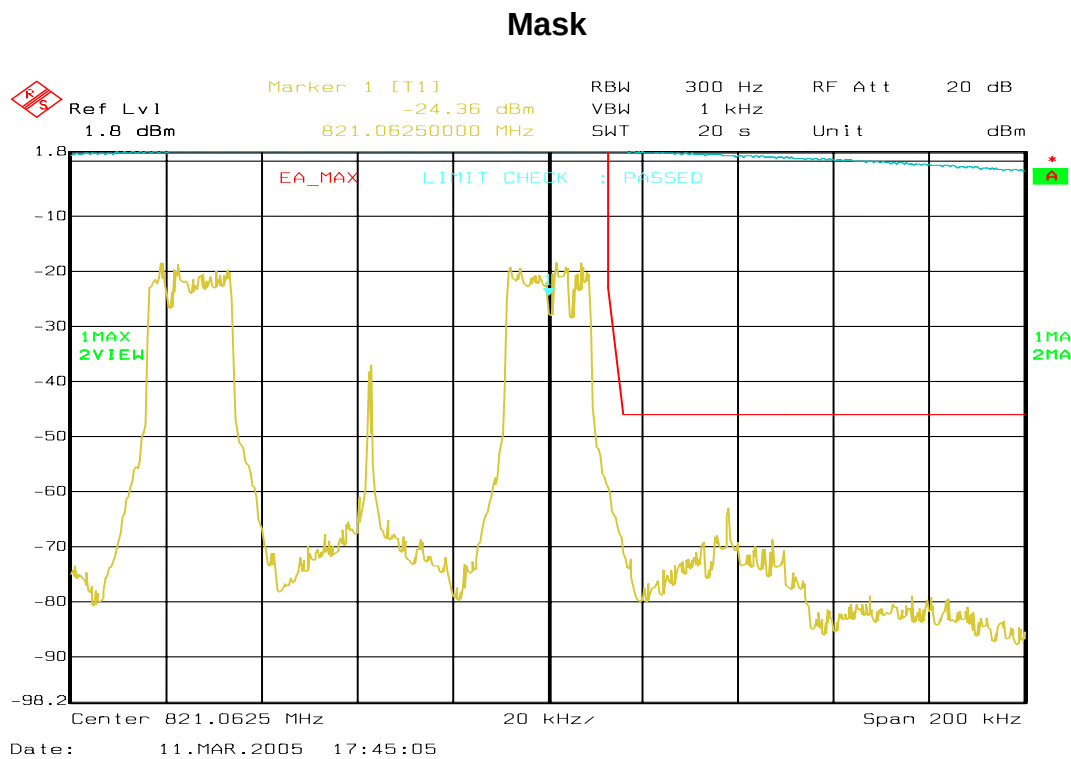
Figure 6a-58 . WiDEN_50_Split 800 MHz Band, QAM64, Maximum Power, EA Emission Mask
