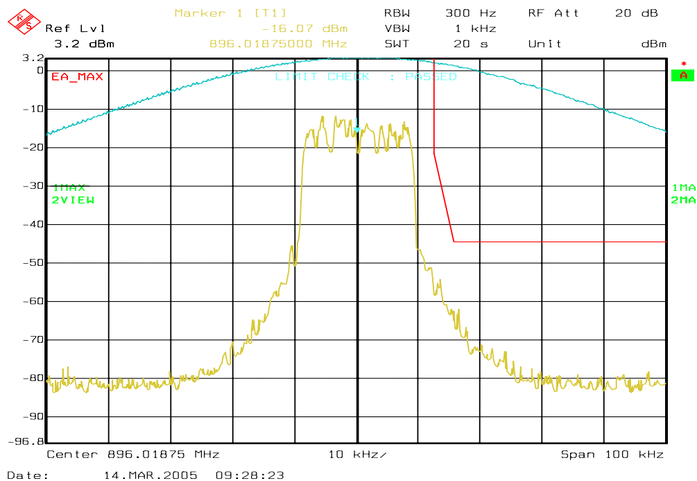
Figure 6a-62 . WiDEN25 900 MHz Band, QAM16, Maximum Power, EA Emission Mask
