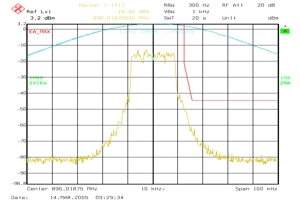
Figure 6a-64 . WiDEN25 900 MHz Band, QAM64, Maximum Power, EA Emission Mask
