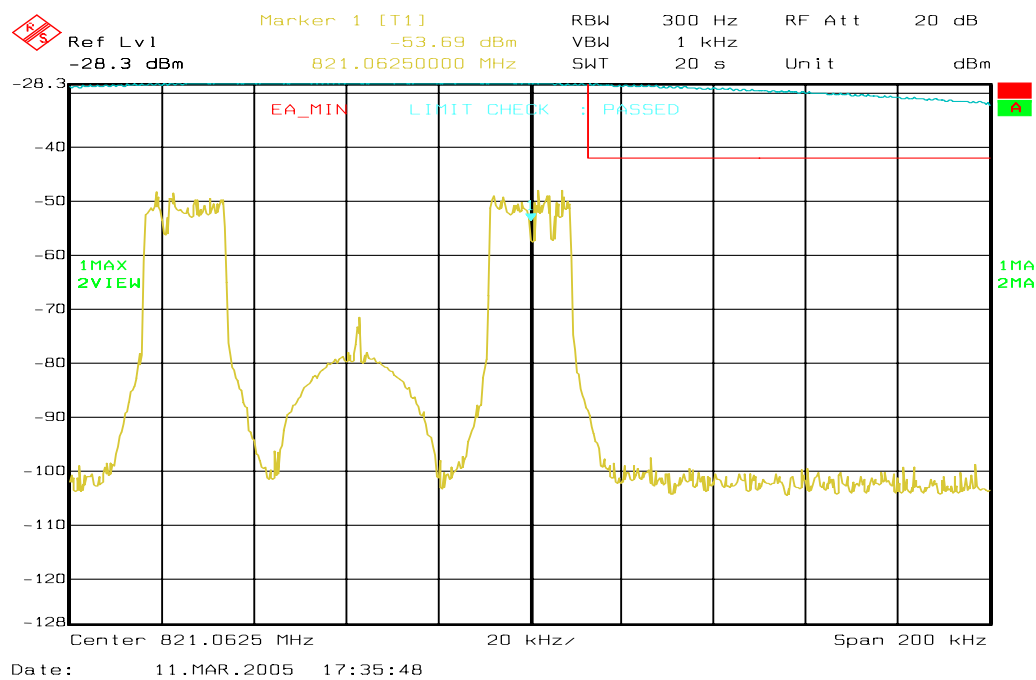
Figure 6a-59 . WiDEN_50_Split 800 MHz Band, QAM64, Minimum Power, EA Emission Mask
