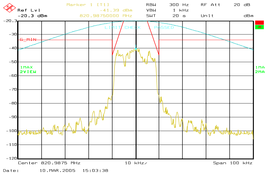
Figure 6a-7: iDEN 800 MHz Band, QPSK, Minimum Power, Emission Mask G
