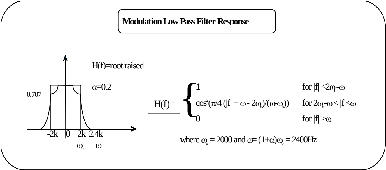
Figure 6a-1: Modulation Low Pass Filter Response
