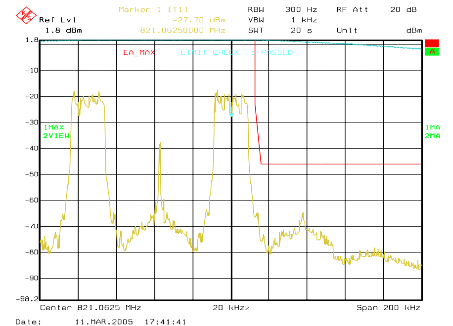
Figure 6a-54 . WiDEN_50_Split 800 MHz Band, Quad-QPSK, Maximum Power, EA Emission Mask
