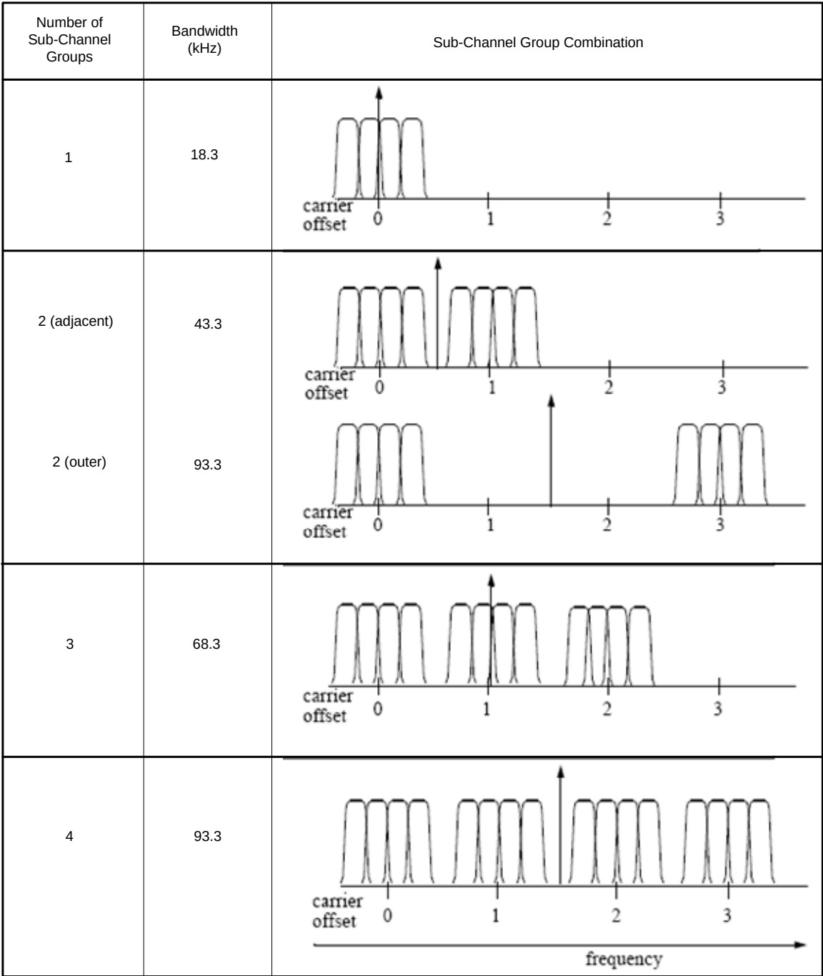
Figure 6a-2: Sub-Channel Group Combination Bandwidths
