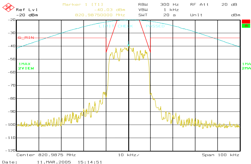
Figure 6a-29: WiDEN25 800 MHz Band, QAM16, Minimum Power, Emission Mask G
