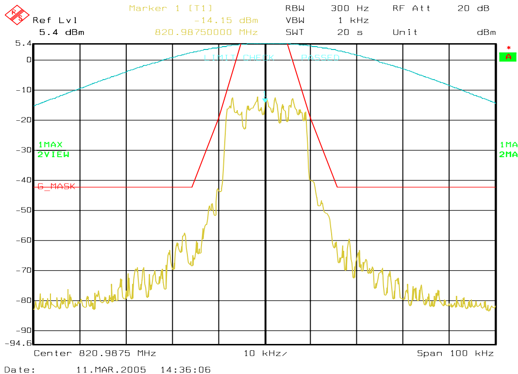
Figure 6a-24: WiDEN25 800 MHz Band, Quad-QPSK, Maximum Power, Emission Mask G
