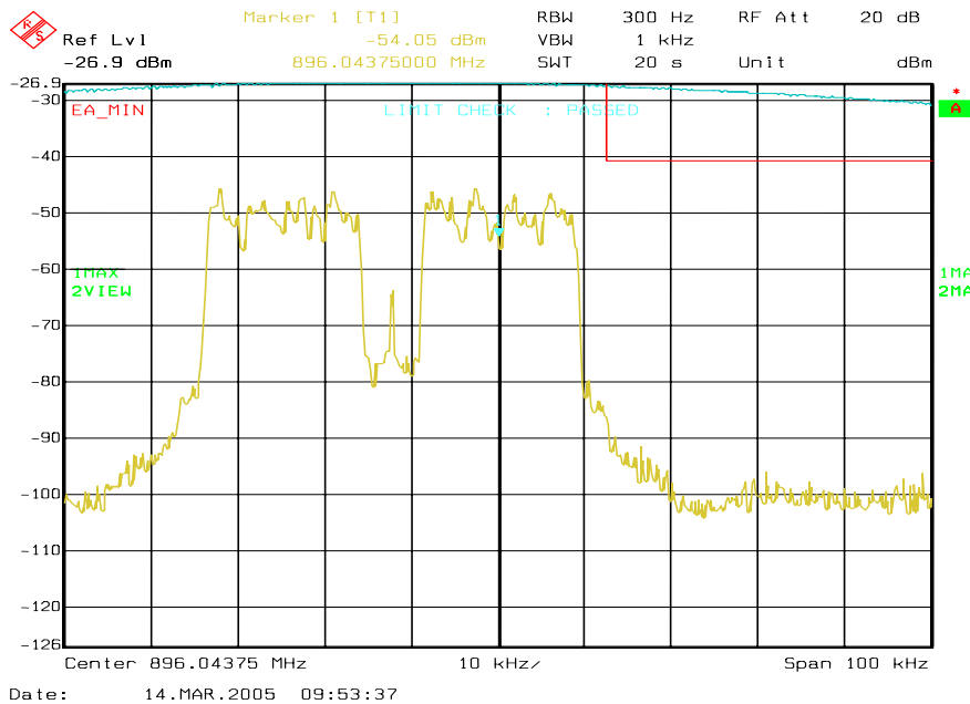
Figure 6a-67 . WiDEN50 900 MHz Band, Continuous Quad-QPSK, Minimum Power, EA Emission Mask
