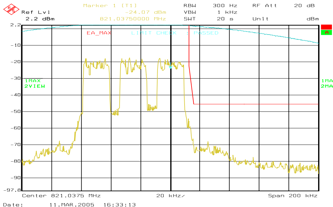
Figure 6a-42 . WiDEN75 800 MHz Band, Quad-QPSK, Maximum Power, EA Emission Mask
