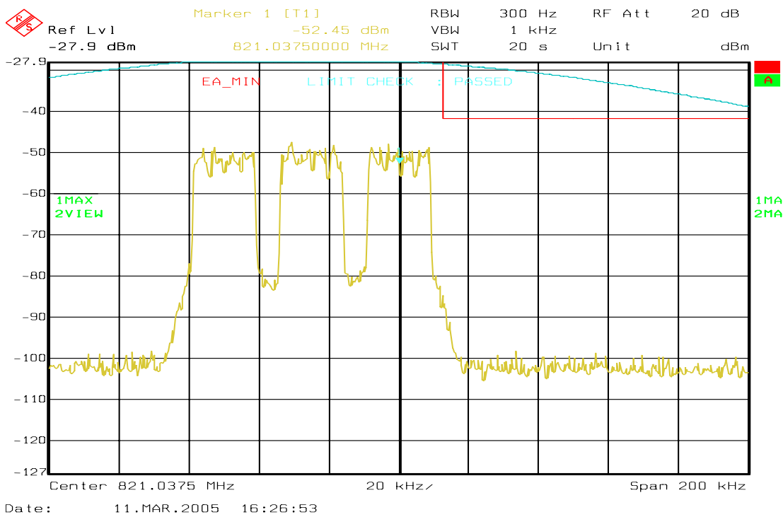
Figure 6a-47 . WiDEN75 800 MHz Band, QAM64, Minimum Power, EA Emission Mask
