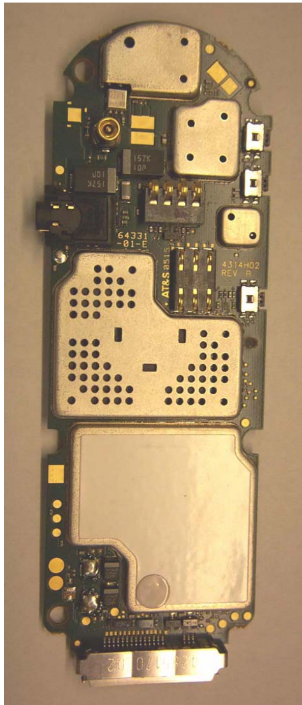
Photograph 9-2: Back side view of radio PCB.
