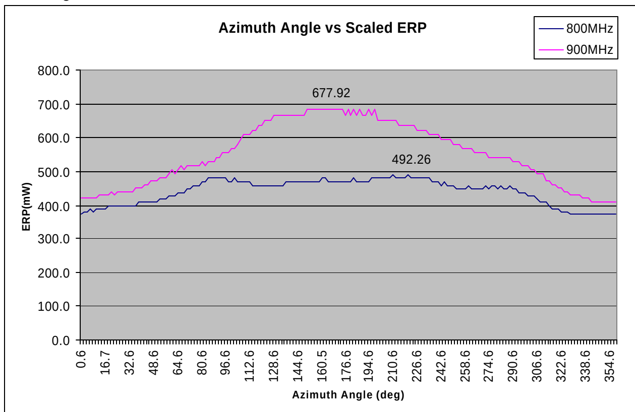
Figure 6-37: Scaled ERP vs. Azimuth Angle
