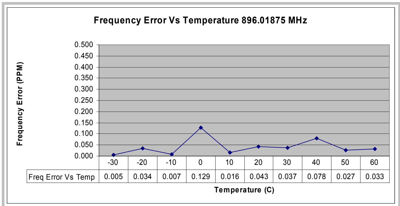
Figure 6-32: Transmitter Frequency Stability (900 MHz band) – Frequency Error vs. Temperature
