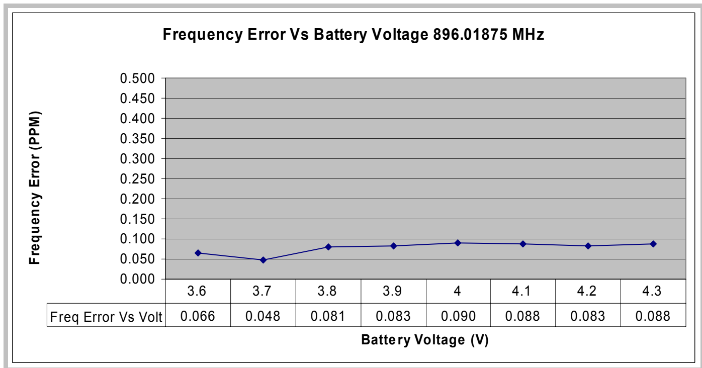
Figure 6-34: Transmitter Frequency Stability (900 MHz band)- Frequency Error vs. Voltage
