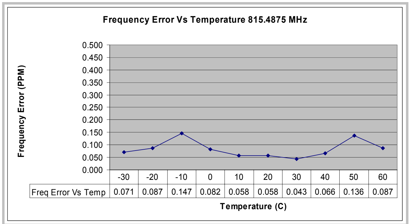
Figure 6-31: Transmitter Frequency Stability (800 MHz band) – Frequency Error vs. Temperature
