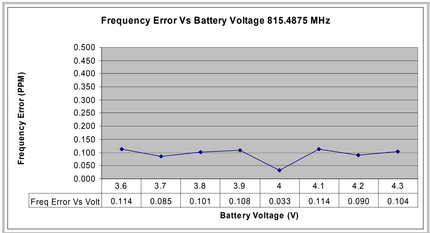
Figure 6-33: Transmitter Frequency Stability (800 MHz band) - Frequency Error vs. Voltage
