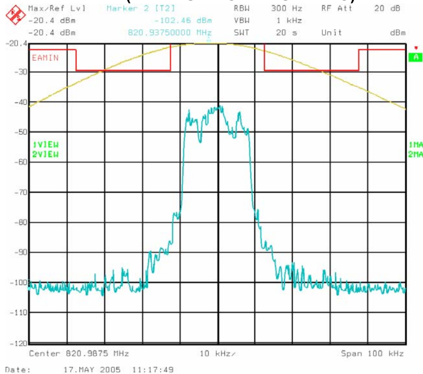
Figure 6-7: Quad-QPSK Modulation performance relative to EA-mask 47 CFR 90.691. (MAXIMUM POWER SETTING)
