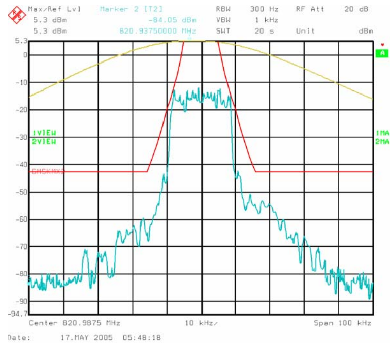
Figure 6-13: Quad-64QAM Modulation performance relative to G-mask 47 CFR 90.210(g) (MAXIMUM POWER SETTING)
