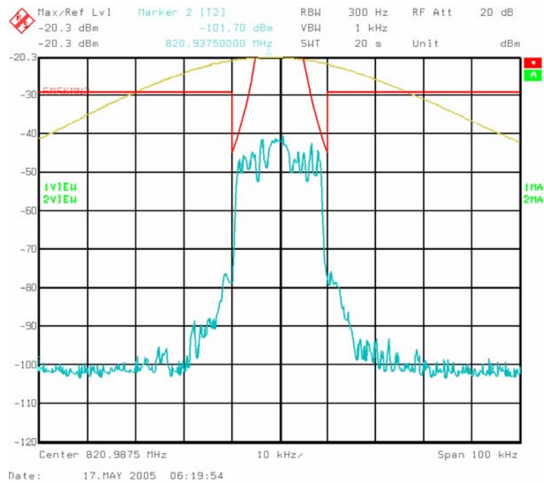
Figure 6-9a: Quad-16QAM Modulation performance relative to G-Mask 47 CFR 90.210(g) (MAXIMUM POWER SETTING)
