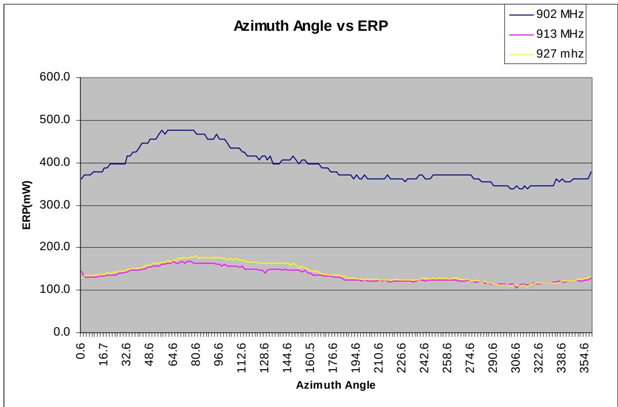
Figure 6b-5.2 MOTotalk ISM Band Scaled ERP v. Azimuth Angle.
