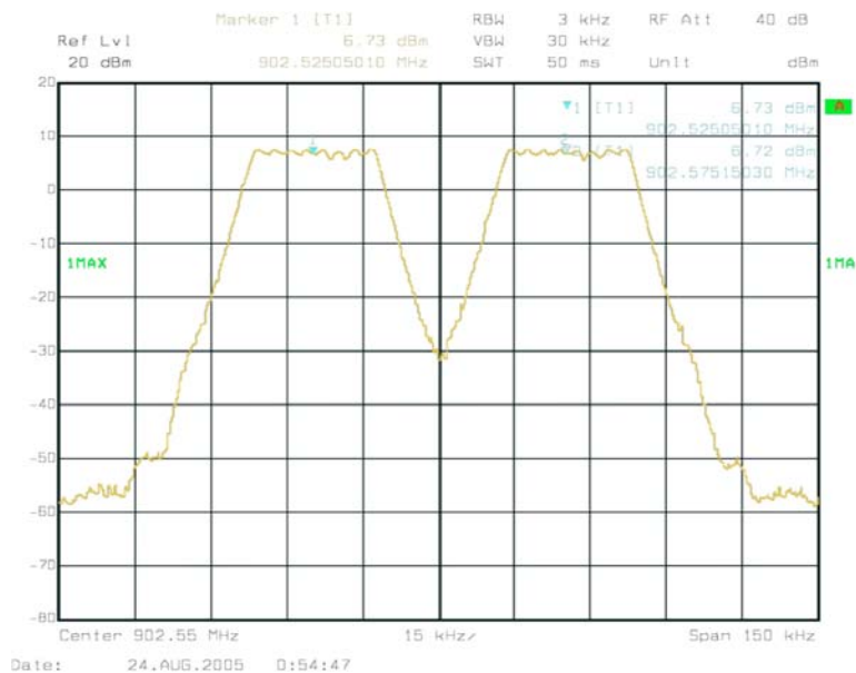
Figure 6b-2.2.3. Adjacent hopset separation with spectrum analyzer center frequency at 902.55 MHz.
