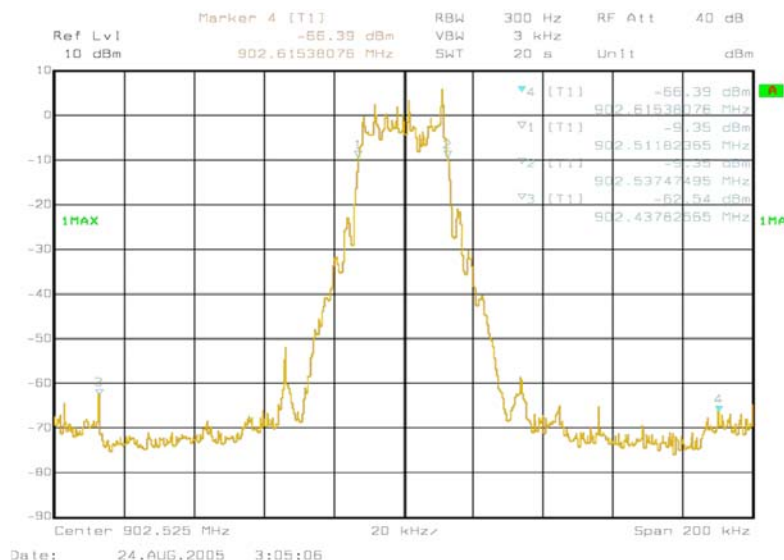
Figure 6b-2.2.2 MOTotalk ISM band occupied bandwidth with frequency span of 200 kHz with hopping function disabled at center frequency 902.525 MHz.
