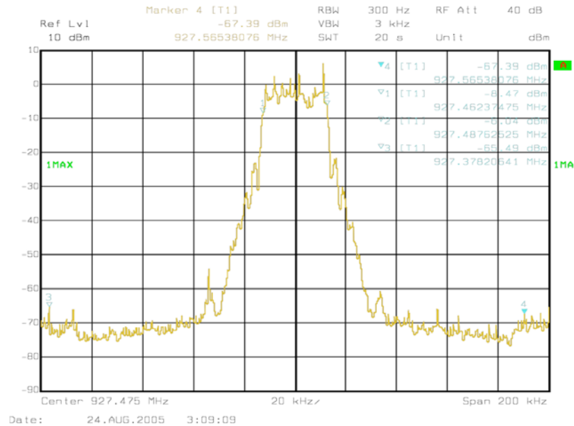
Figure 6b-2.2.6 MOTotalk ISM band occupied bandwidth with frequency span of 200 kHz with hopping function disabled, at center frequency 927.475.
