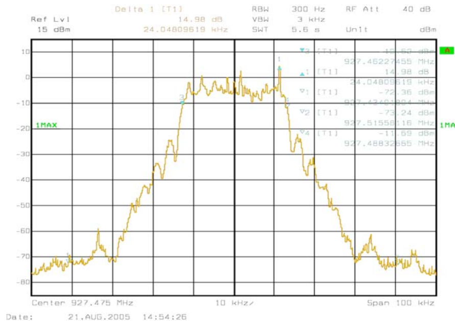
Figure 6b-2.2.5 Spectrum analyzer plot of MOTotalk ISM Band 8-FSK traffic channel signal's 99% bandwidth with hopping function disabled, at center frequency 927.475 MHz.
