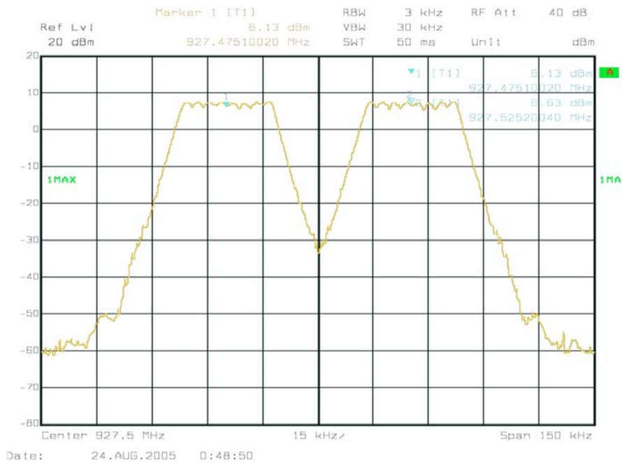
Figure 6b-2.2.7. Adjacent hopset separation with spectrum analyzer center frequency 927.5 MHz.
