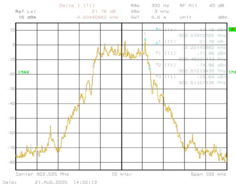
Figure 6b-2.2.1 Spectrum analyzer plot of MOTotalk ISM Band 8-FSK traffic channel signal's 99% bandwidth at center frequency 902.525 MHz with hopping function disabled.
