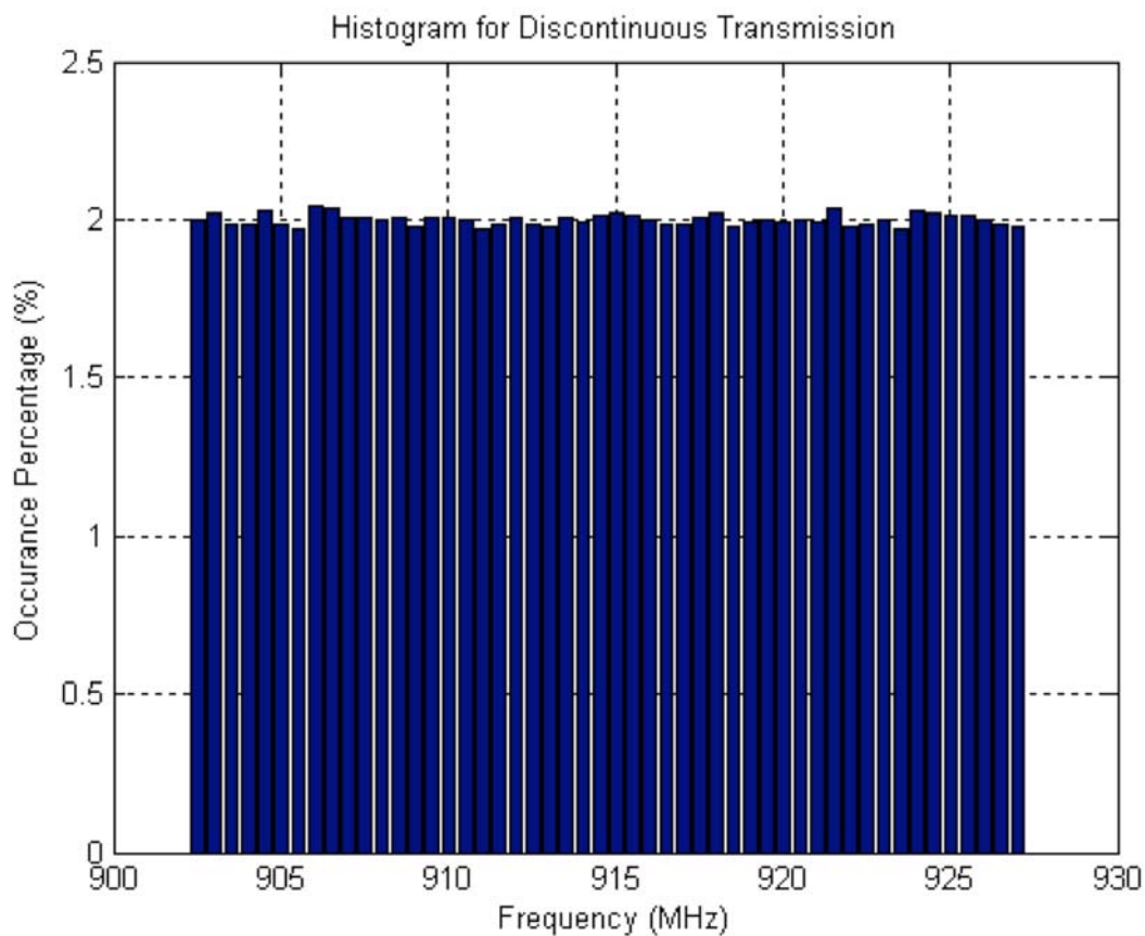
Figure 6b-2.7.1. Histogram for MOTotalk ISM Band Discontinuous Transmission
