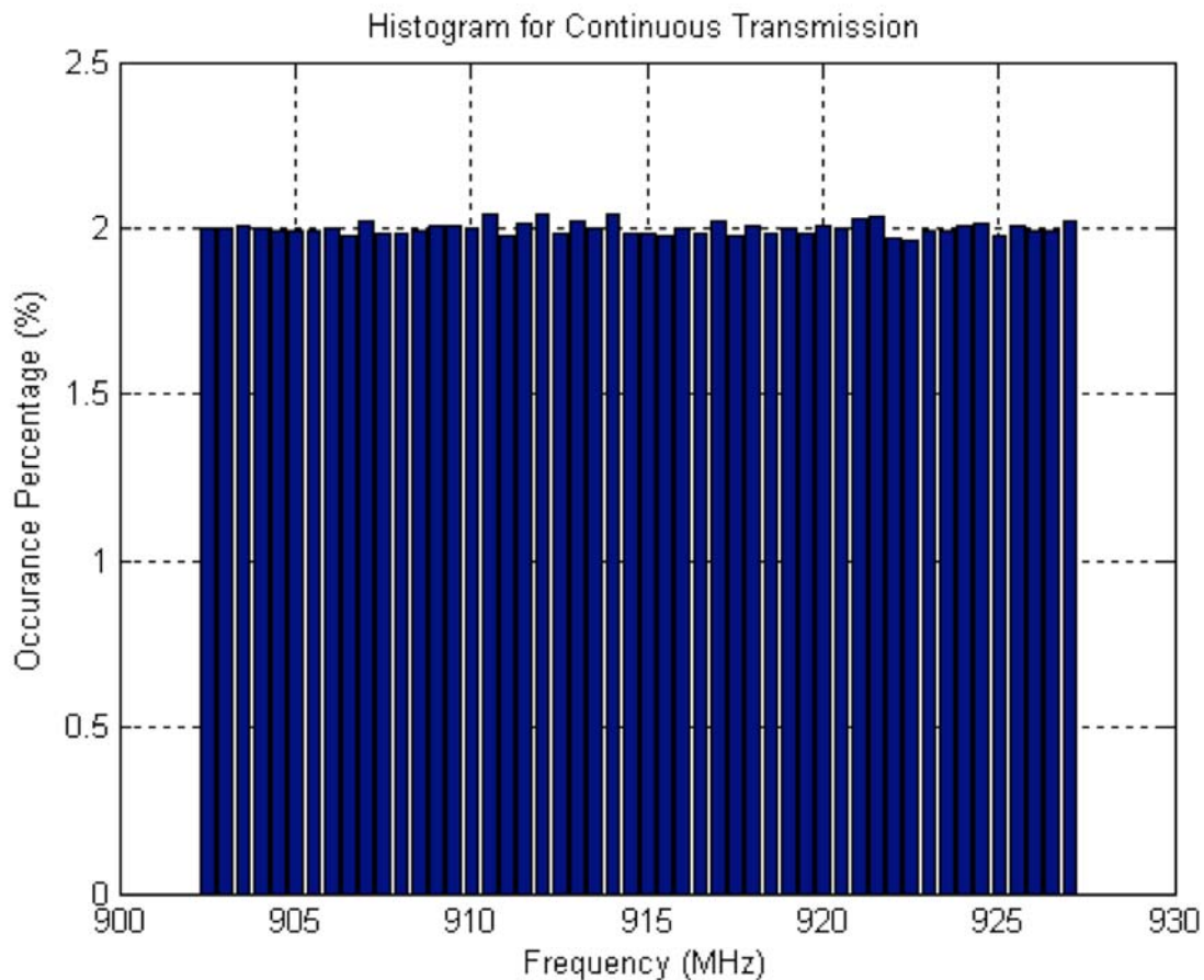
Figure 6b-2.6.1. Histogram for MOTotalk ISM Band Continuous Transmission
