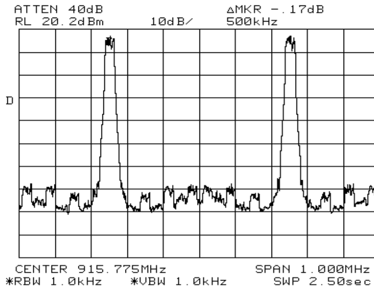
Figure 6b-2.1.1. Plot of MOTotalk ISM Band adjacent channel separation within a hopset
