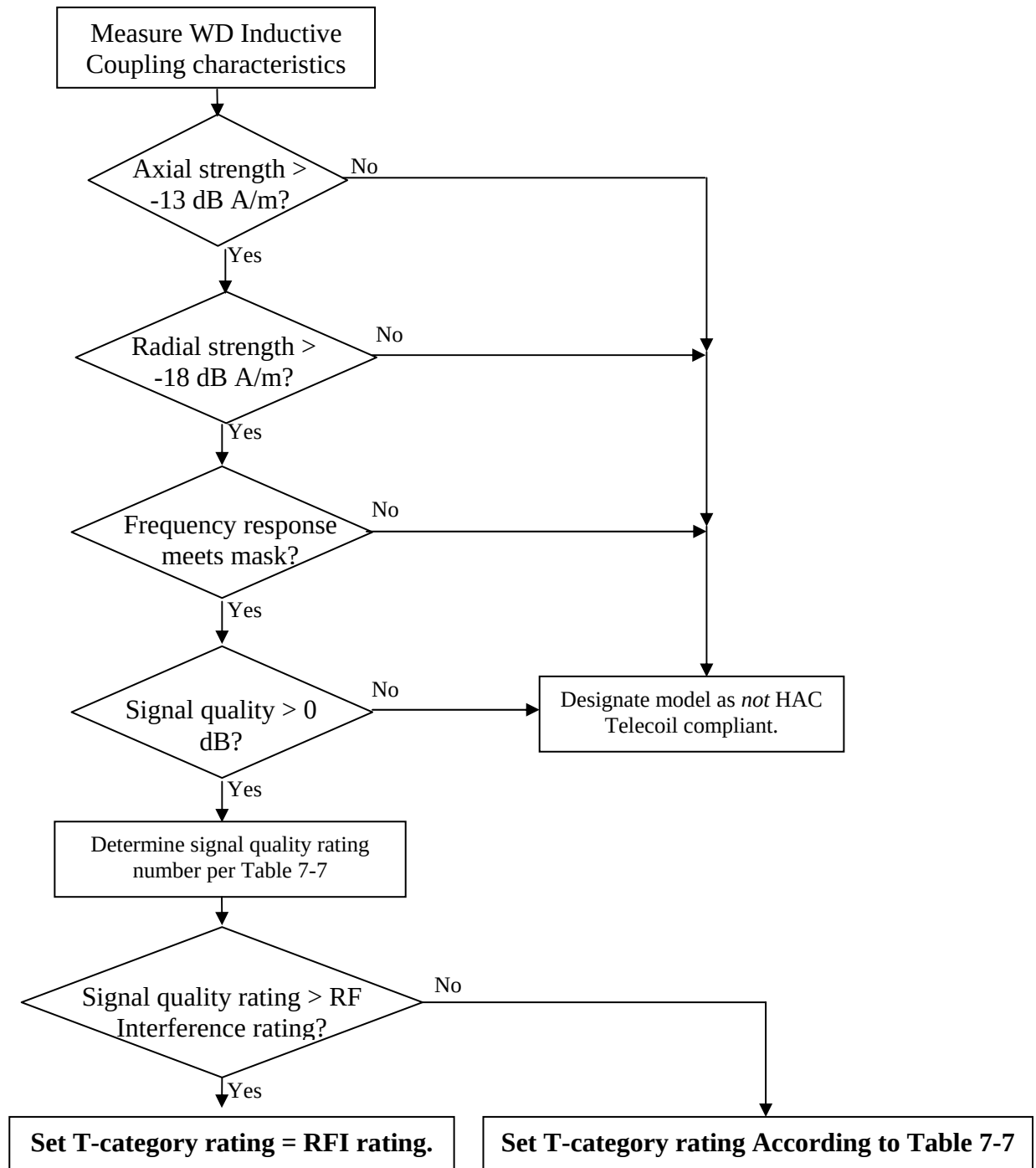
Figure 2-2 - WD Telecoil Category Rating Process
