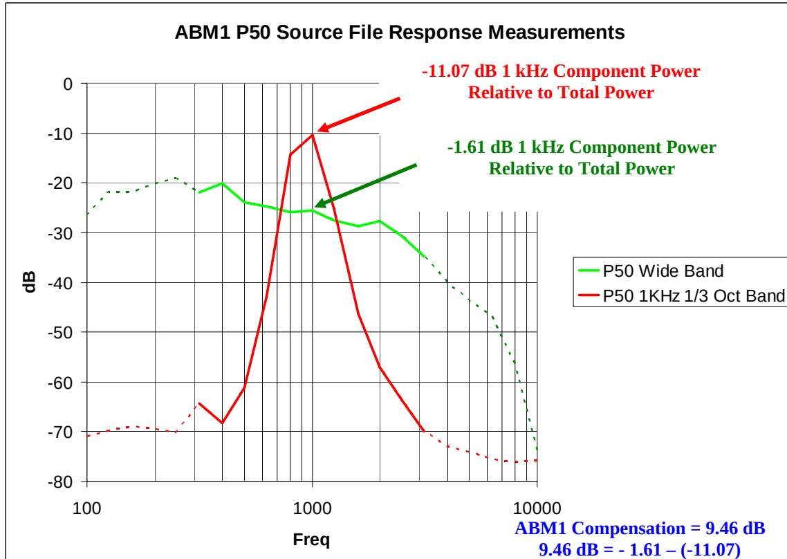
Figure 6-4-1 – P50 Source Characterization (Wideband v. Narrowband)
