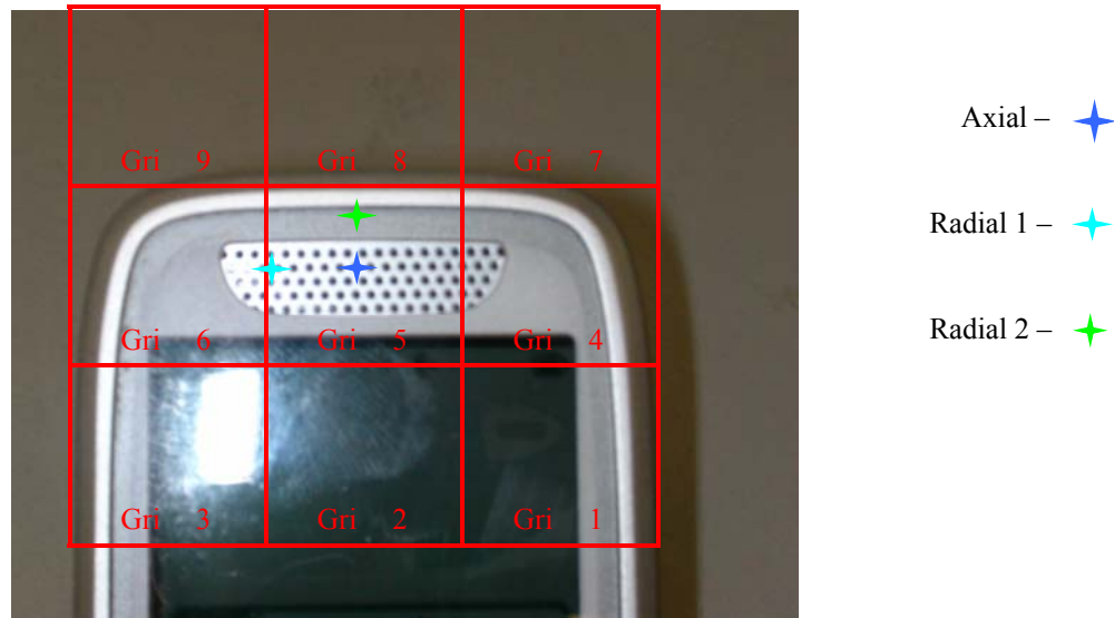
Figure 12 – Measurement Locations
