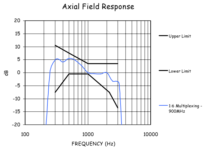
Figure 14D – 900MHz Measured Frequency response
