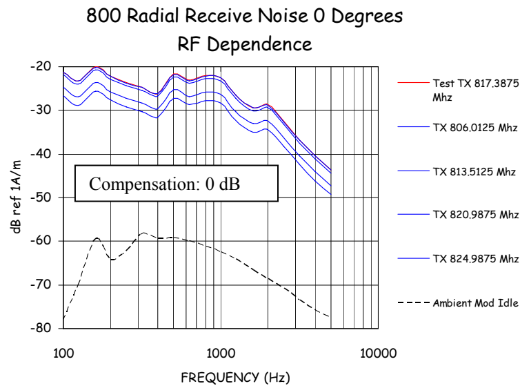
Figure 10B – 800 MHz Radial (0-degrees) Receive Noise Compensation
