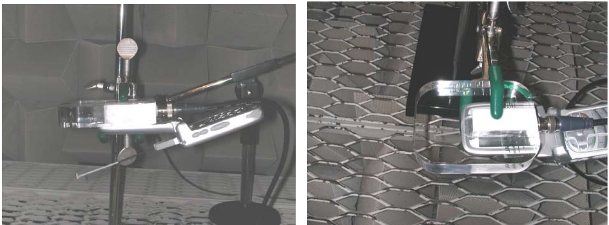
Figure 10 – Test holder
