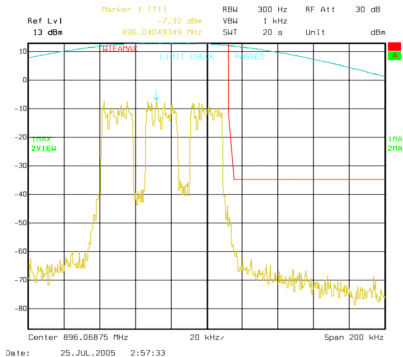
Figure 6a-2.10.1. WiDEN75 900 MHz Band, Quad-QPSK, Maximum Power, EA Emission Mask
