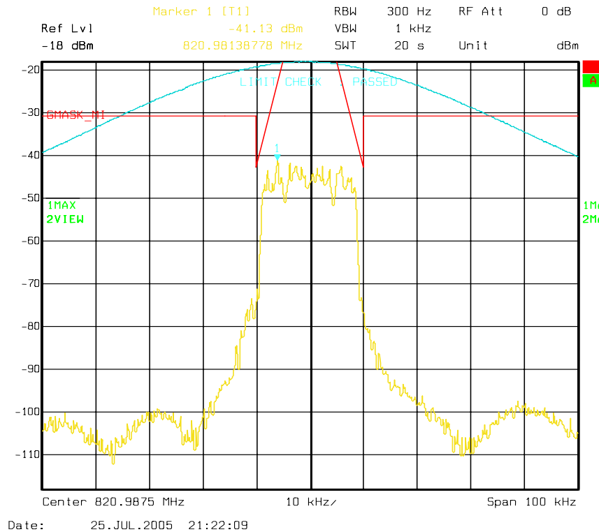
Figure 6a-2.1.6. iDEN 800 MHz Band, QAM16, Minimum Power, Emission Mask G
