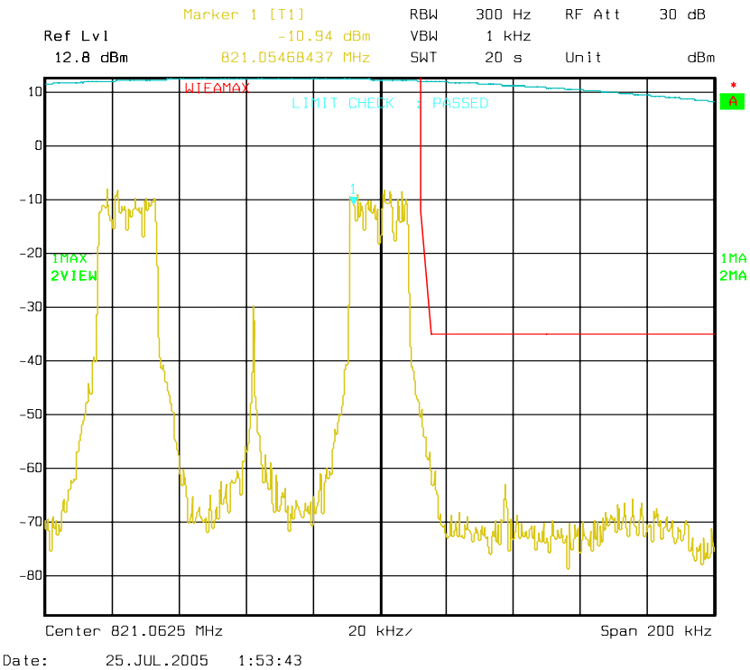
Figure 6a-2.7.5. WiDEN50_Split 800 MHz Band, QAM64, Maximum Power, EA Emission Mask
