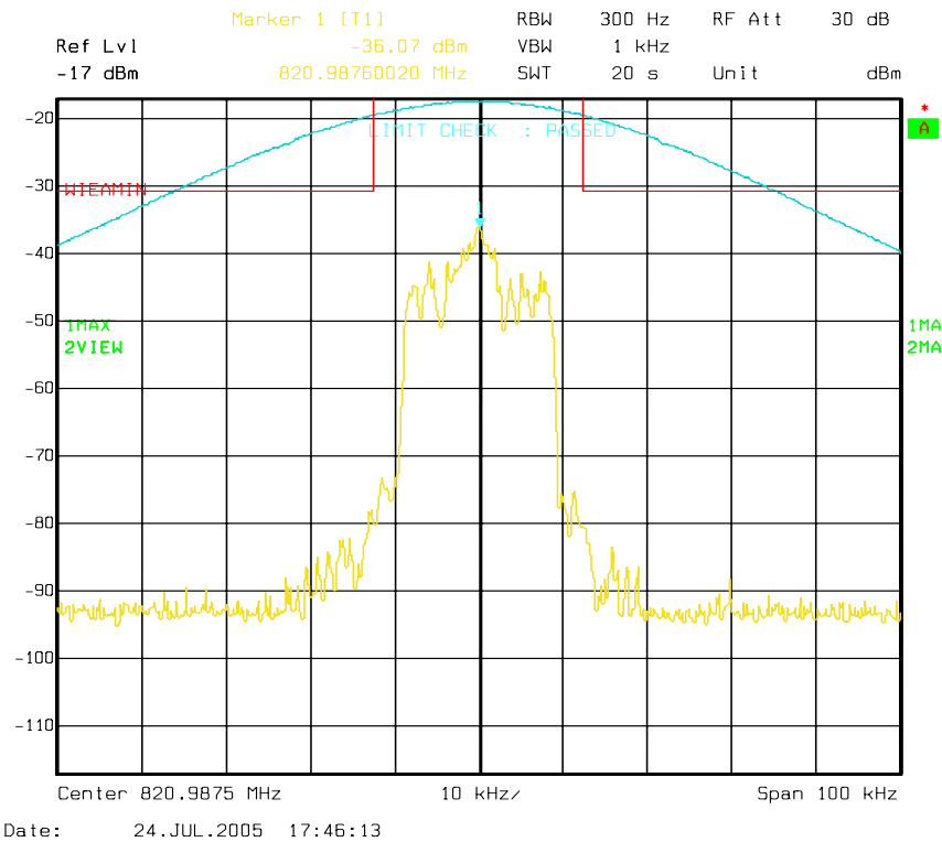
Figure 6a-2.3.8. WIDEN25 800 MHz Band, QAM16, Minimum Power, EA Emission Mask
