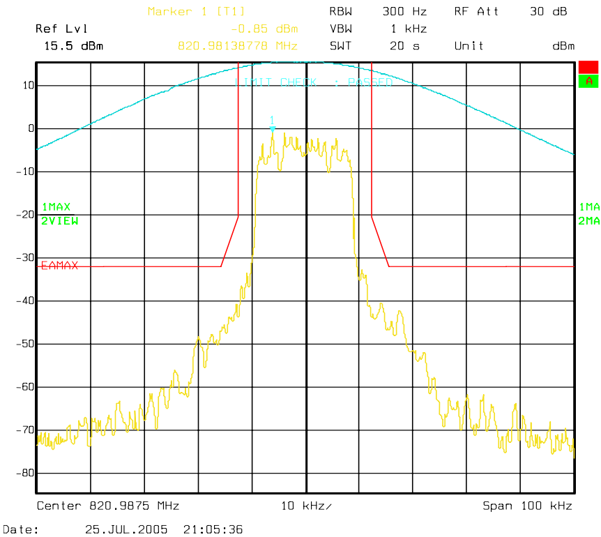
Figure 6a-2.1.7. iDEN 800 MHz Band, QAM16, Maximum Power, EA Emission Mask
