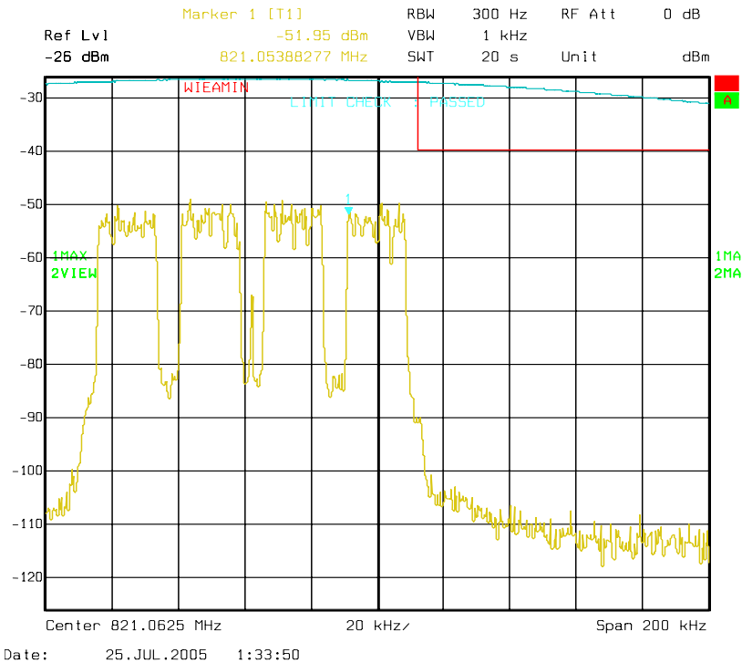
Figure 6a-2.6.6. WiDEN100 800 MHz Band, QAM64, Minimum Power, EA Emission Mask
