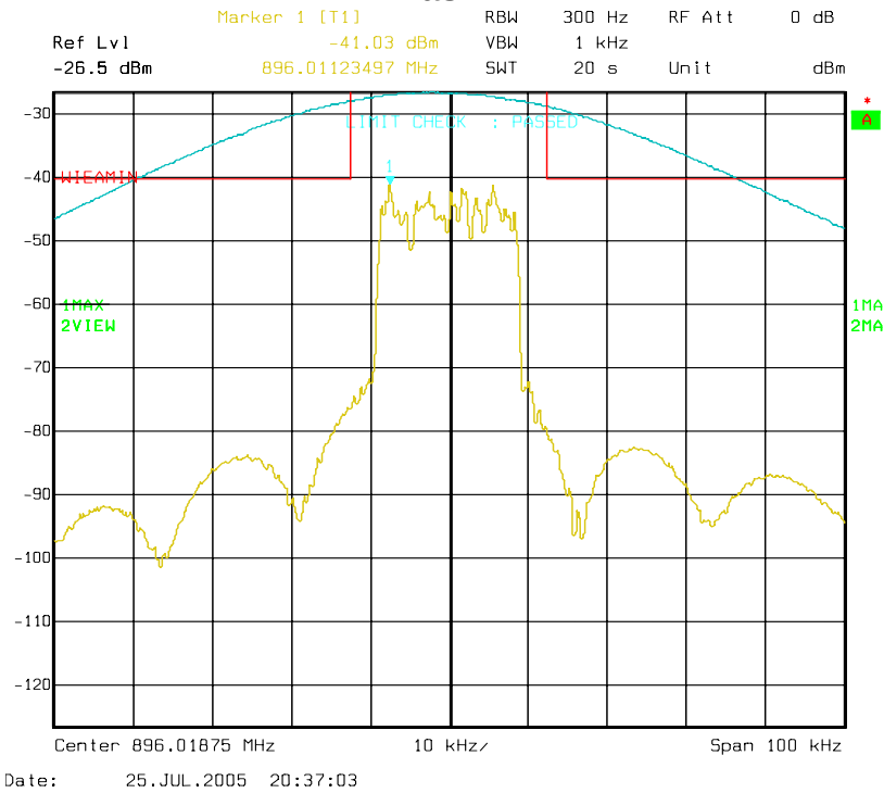
Figure 6a-2.8.1. WiDEN25 900 MHz Band, Quad-QPSK, Maximum Power, EA Emission Mask
