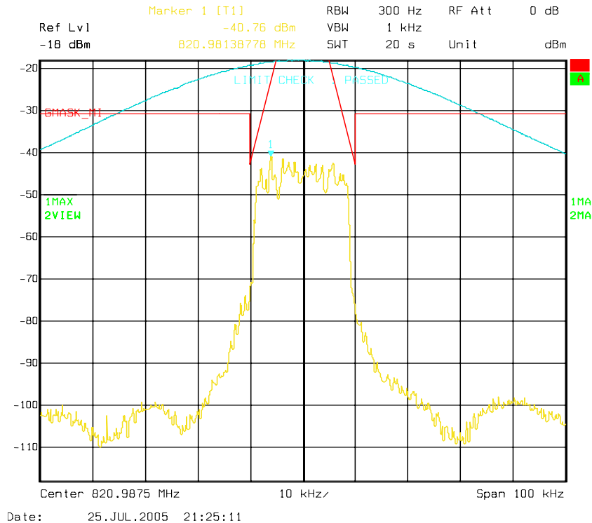
Figure 6a-2.1.10. iDEN 800 MHz Band, QAM64, Minimum Power, Emission Mask G
