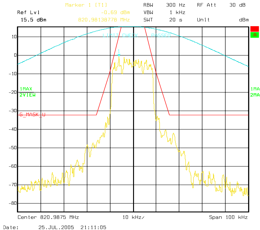
Figure 6a-2.1.9. iDEN 800 MHz Band, QAM64, Maximum Power, Emission Mask G
