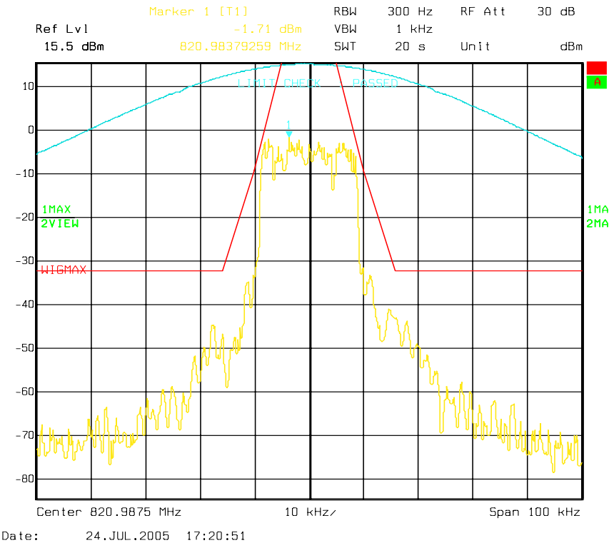
Figure 6a-2.3.1. WiDEN25 800 MHz Band, Quad-QPSK, Maximum Power, Emission Mask G
