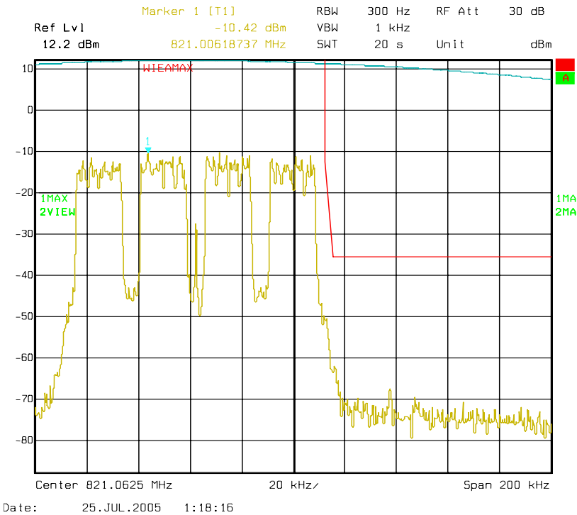
Figure 6a-2.6.5. WiDEN100 800 MHz Band, QAM64, Maximum Power, EA Emission Mask
