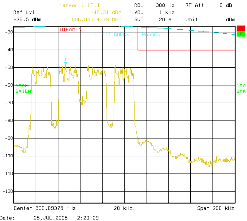
Figure 6a-2.11.2. WiDEN100 900 MHz Band, Quad-QPSK, Minimum Power, EA Emission Mask
