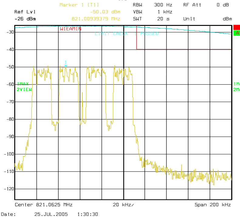
Figure 6a-2.6.1. WiDEN100 800 MHz Band, Quad-QPSK, Maximum Power, EA Emission Mask
