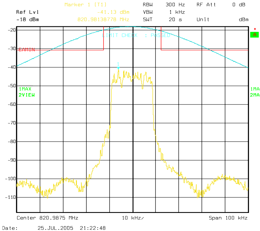
Figure 6a-2.1.8. iDEN 800 MHz Band, QAM16, Minimum Power, EA Emission Mask
