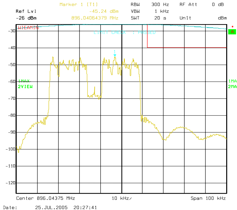
Figure 6a-2.9.1. WiDEN50 900 MHz Band, Continuous Quad-QPSK, Maximum Power, EA Emission Mask
