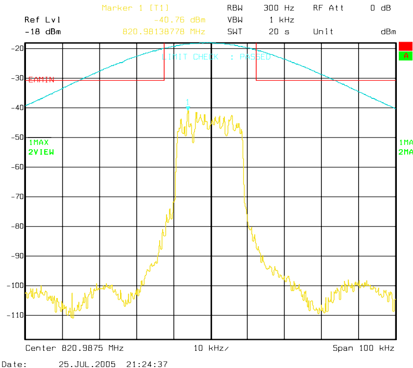
Figure 6a-2.1.12. iDEN 800 MHz Band, QAM64, Minimum Power, EA Emission Mask
