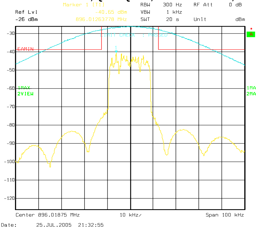
Figure 6a-2.2.2. iDEN 900 MHz Band, Quad-QPSK, Minimum Power, EA Emission Mask
