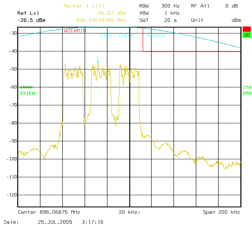
Figure 6a-2.10.2. WiDEN75 900 MHz Band, Quad-QPSK, Minimum Power, EA Emission Mask
