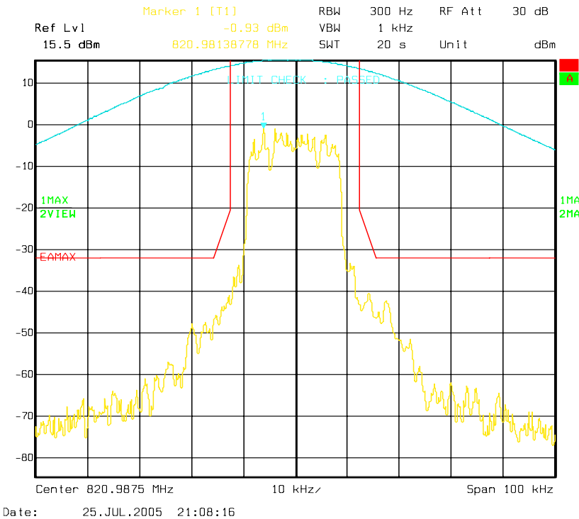
Figure 6a-2.1.3. iDEN 800 MHz Band, Quad-QPSK, Maximum Power, EA Emission Mask
