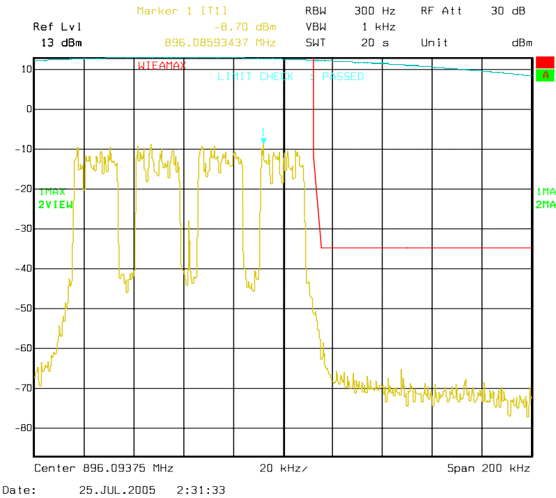
Figure 6a-2.11.1. WiDEN100 900 MHz Band, Quad-QPSK, Maximum Power, EA Emission Mask
