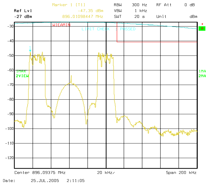
Figure 6a-2.12.2. WiDEN50_Split 900 MHz Band, Quad-QPSK, Minimum Power, EA Emission Mask
