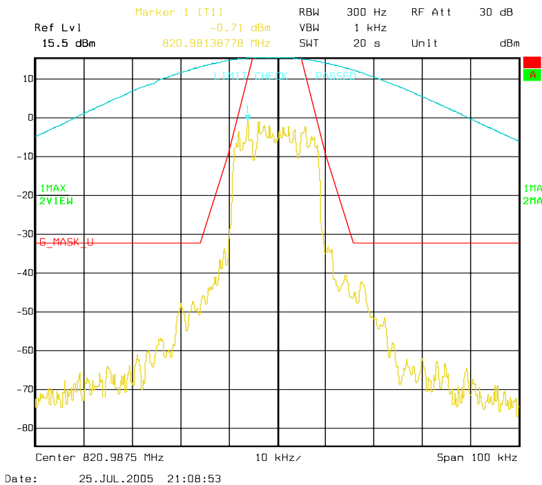
Figure 6a-2.1.1. iDEN 800 MHz Band, QPSK, Maximum Power, Emission Mask G
