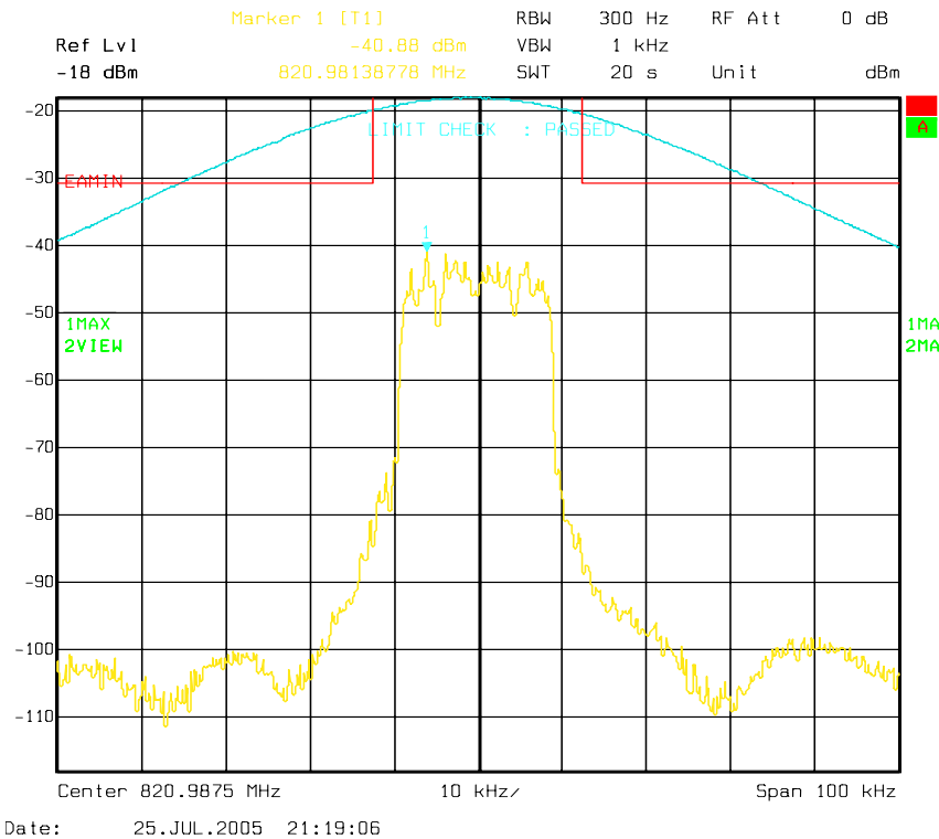
Figure 6a-2.1.4. iDEN 800 MHz Band, QPSK, Minimum Power, EA Emission Mask
