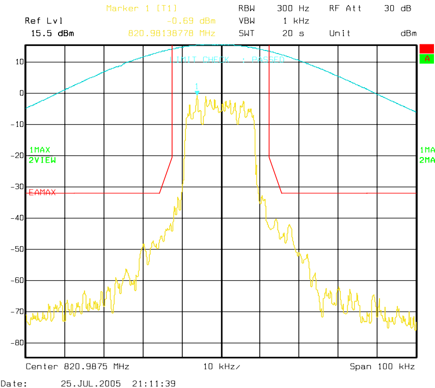
Figure 6a-2.1.11. iDEN 800 MHz Band, QAM64, Maximum Power, EA Emission Mask
