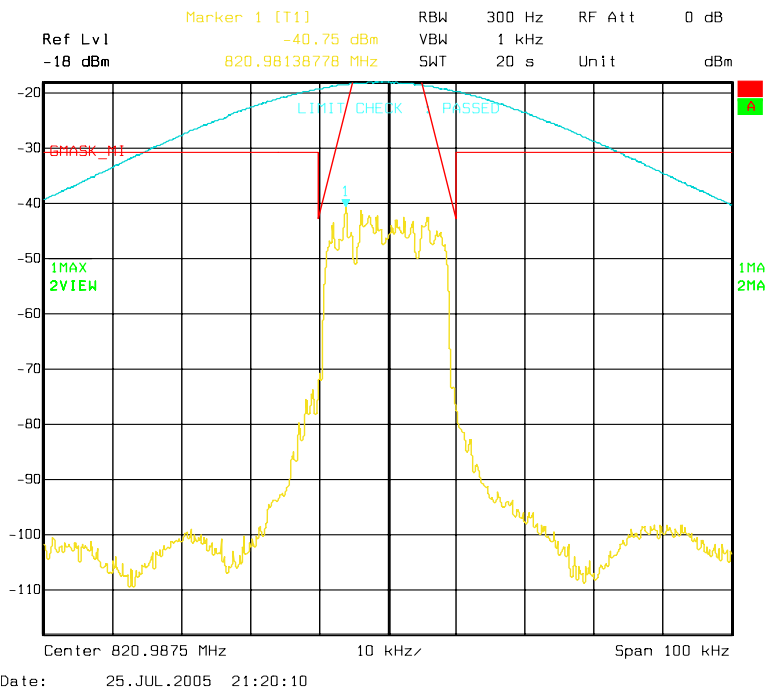
Figure 6a-2.1.2. iDEN 800 MHz Band, QPSK, Minimum Power, Emission Mask G
