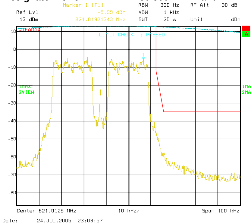
Figure 6a-2.4.1. WiDEN50 800 MHz Band, Continuous Quad-QPSK, Maximum Power, EA Emission Mask
