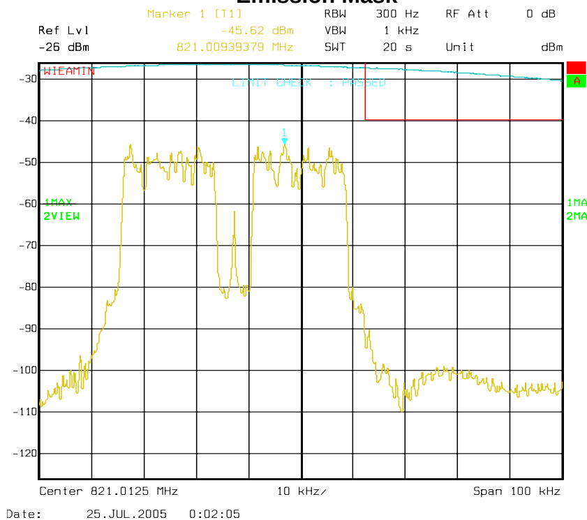
Figure 6a-2.4.2. WiDEN50 800 MHz Band, Continuous Quad-QPSK, Minimum Power, EA Emission Mask
