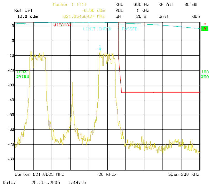
Figure 6a-2.7.1. WiDEN50_Split 800 MHz Band, Quad-QPSK, Maximum Power, EA Emission Mask
