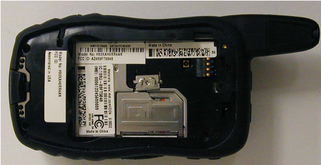
Figure 3-9 Battery Compartment of i580 radio.
