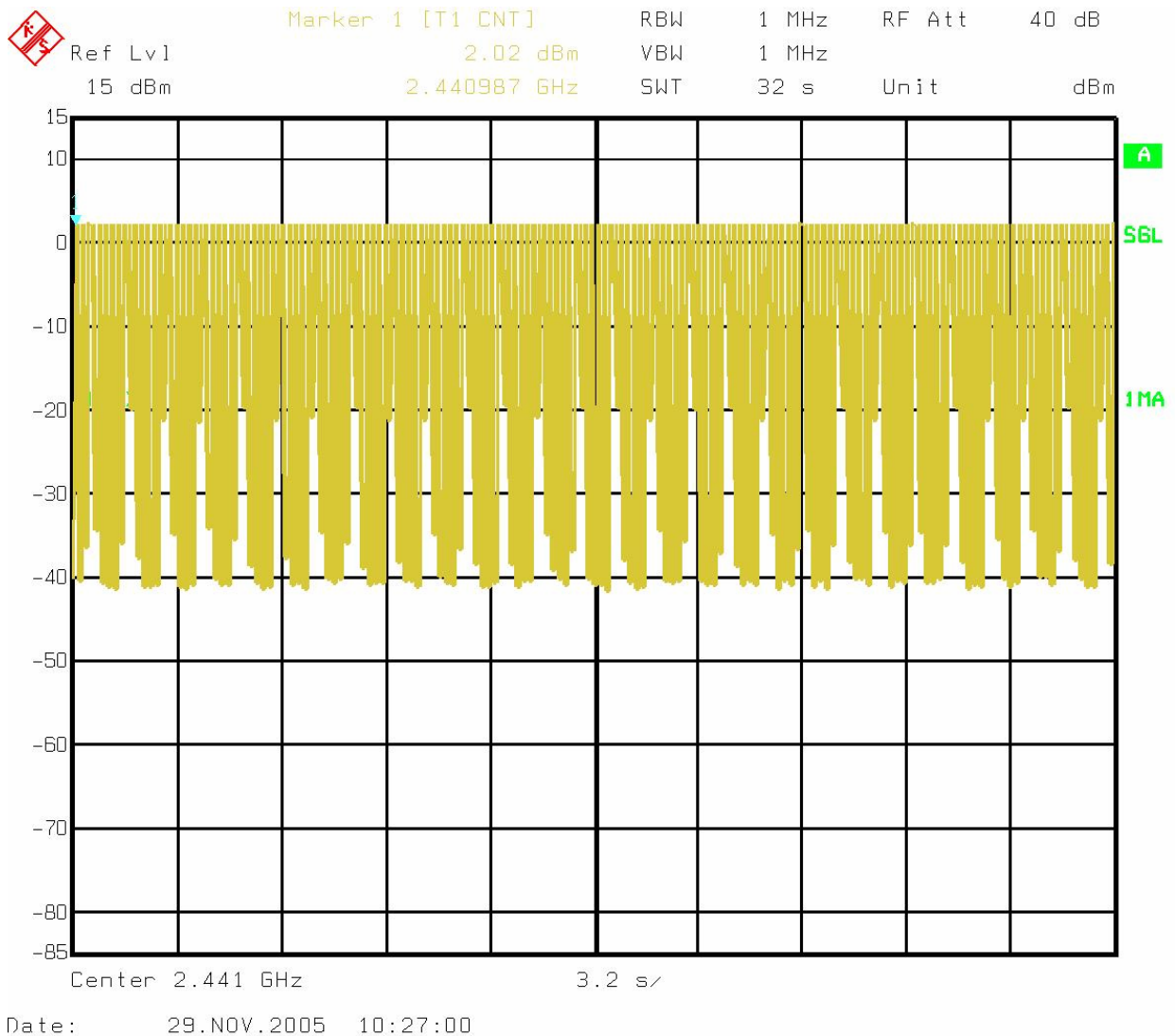
Figure 6-40: Plot of dwell time over 32 second period
