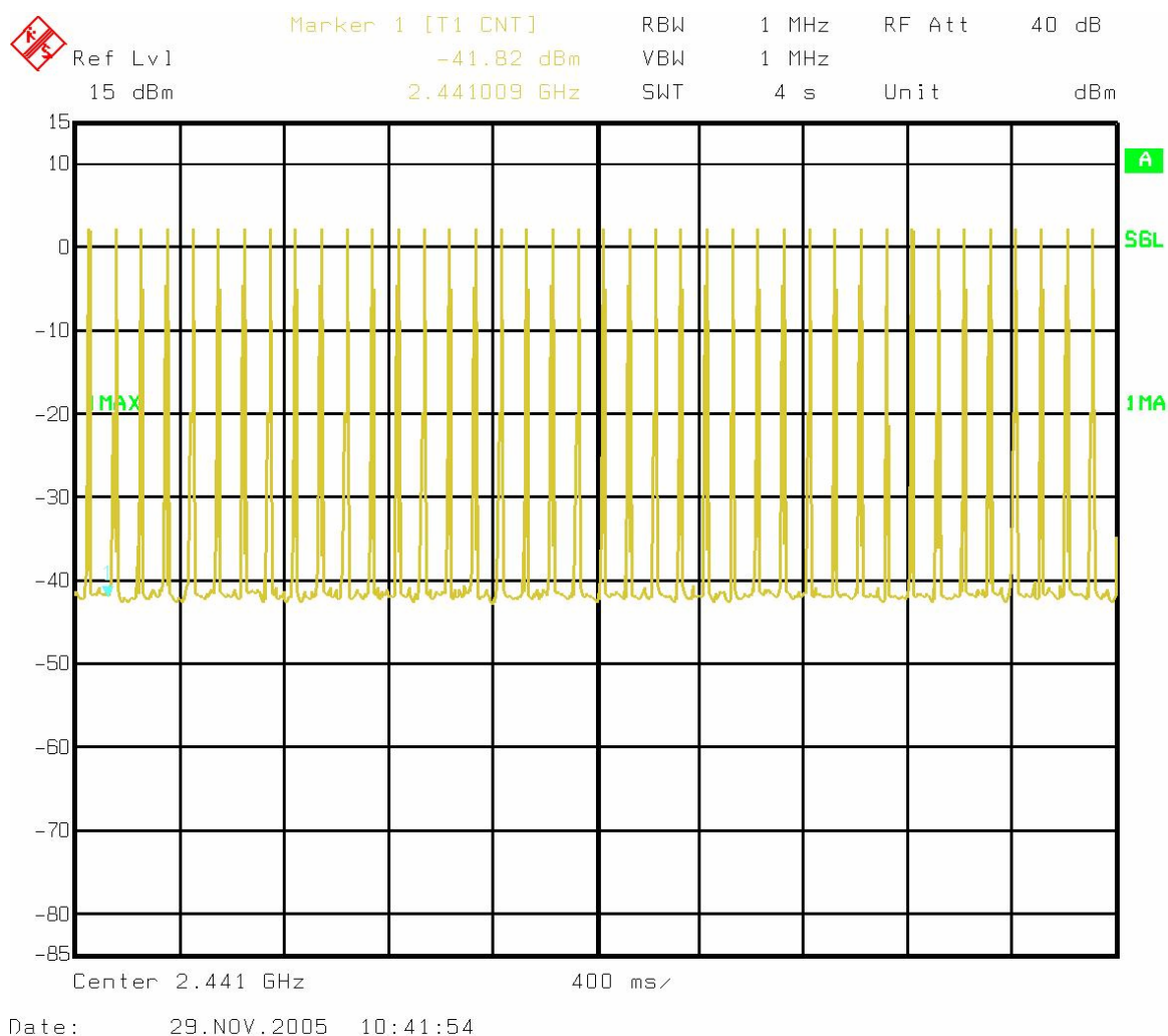
Figure 6-41: Plot of dwell time over 4 second period
