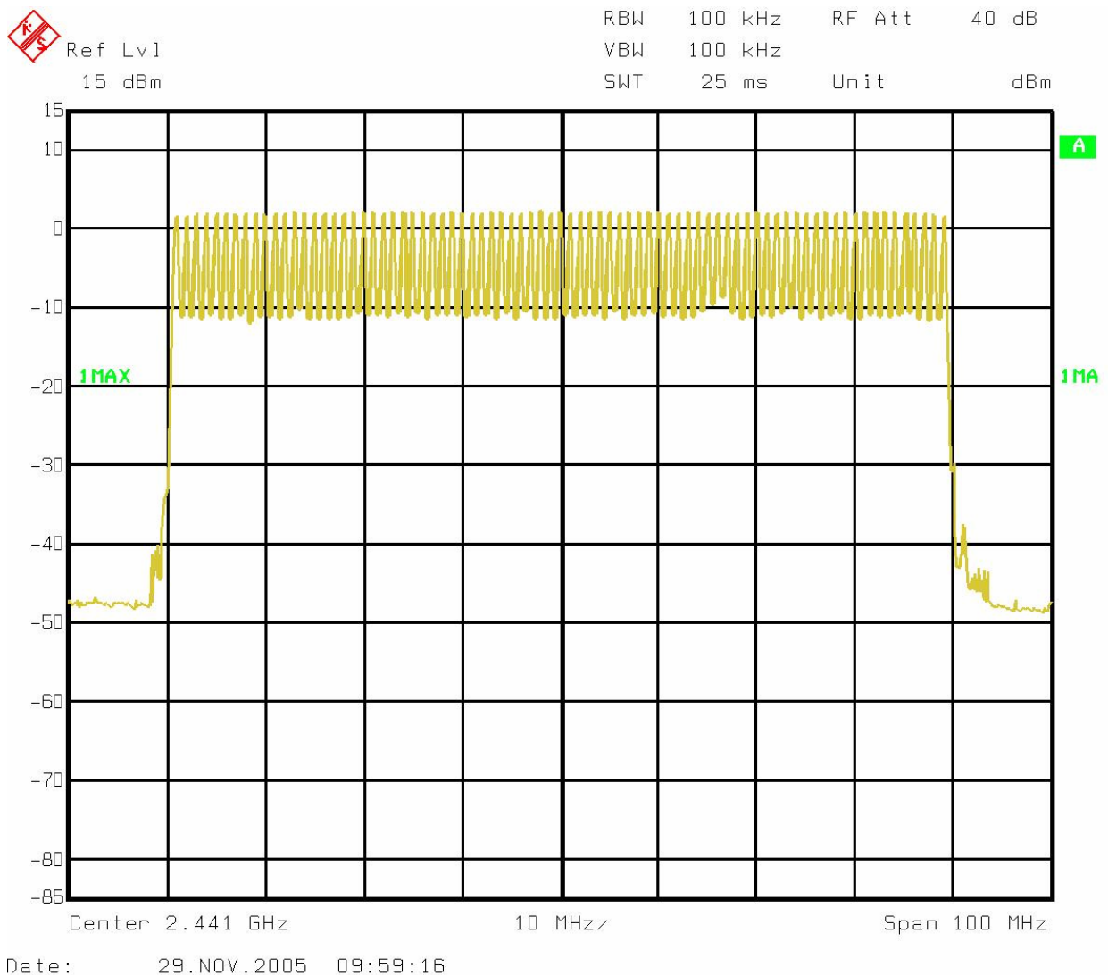
Figure 6-39: Plot of number of Bluetooth hopping frequencies
