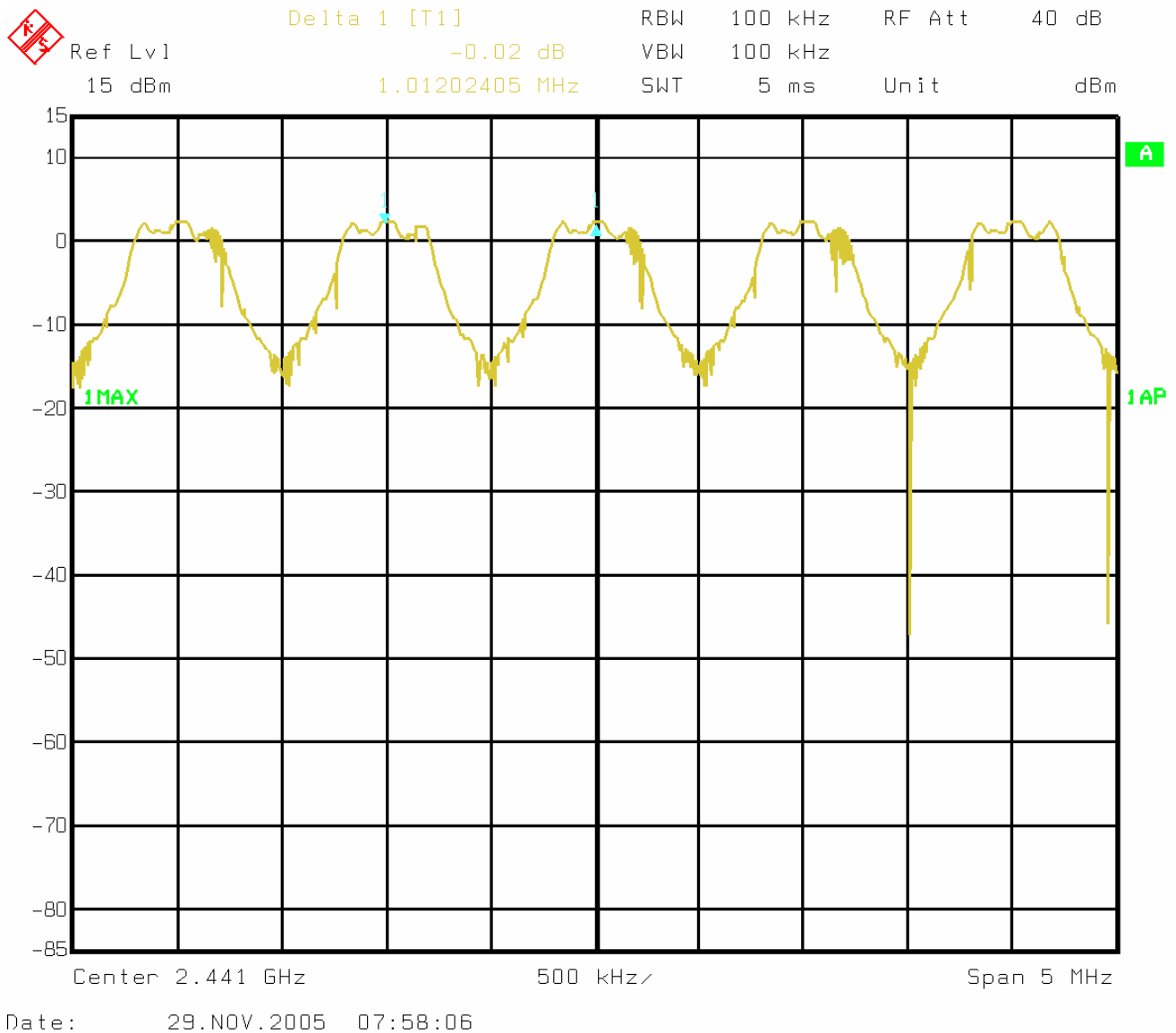
Figure 6-38: Plot of Bluetooth carrier frequency separation
