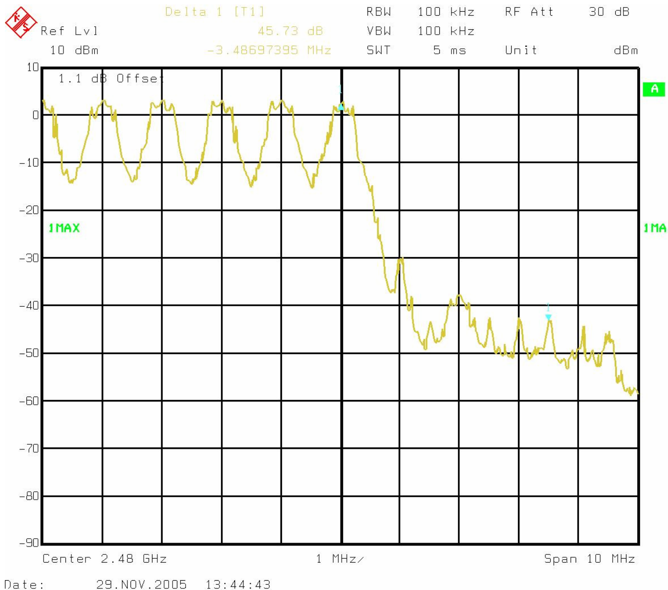
Figure 6-48: Plot of upper band-edge conducted emissions with hopping enabled
