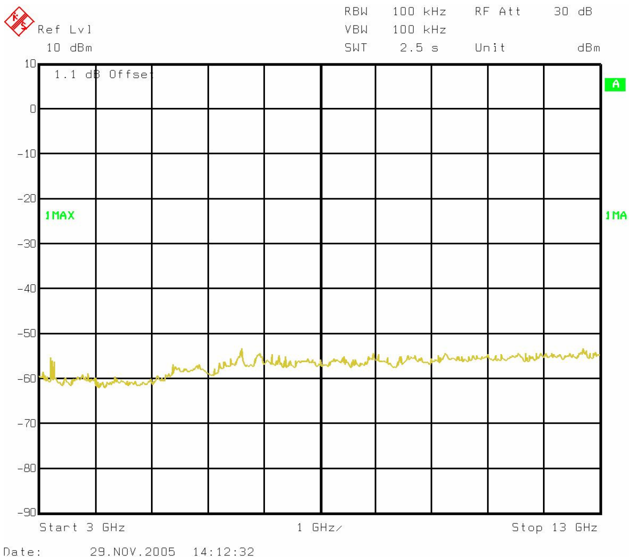
Figure 6-50: Plot of spurious conducted emissions 3 GHz – 13 GHz
