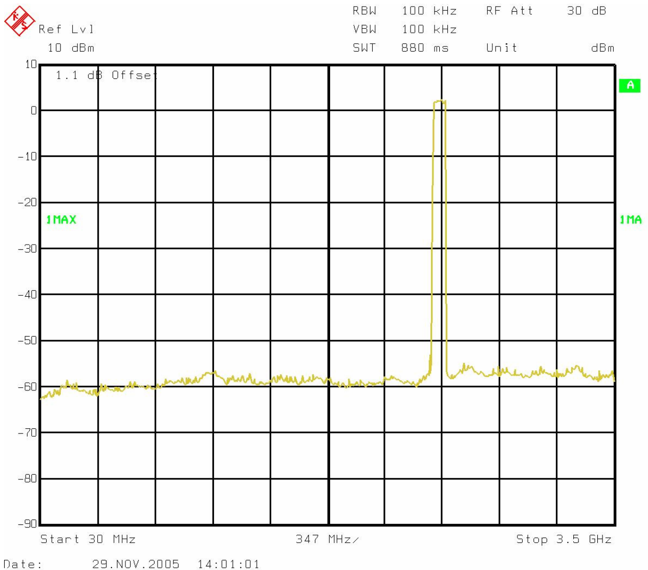
Figure 6-49: Plot of spurious conducted emissions 30 MHz – 3.5 GHz
