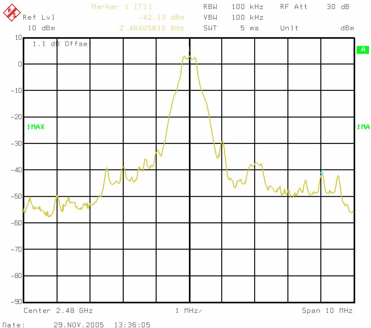
Figure 6-46: Plot of upper band-edge conducted emissions with hopping disabled
