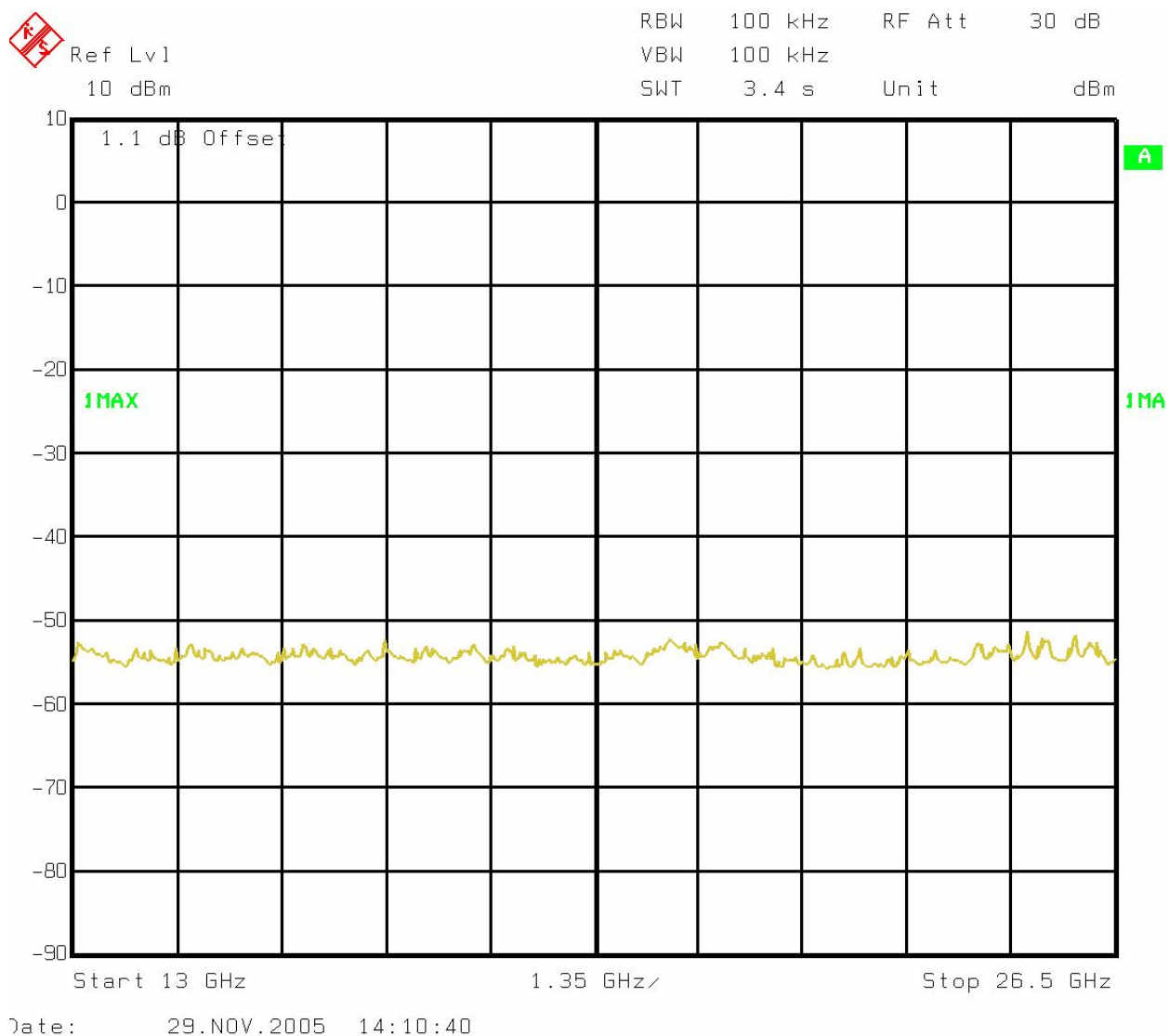
Figure 6-51: Plot of spurious conducted emissions 13 GHz – 26.5 GHz
