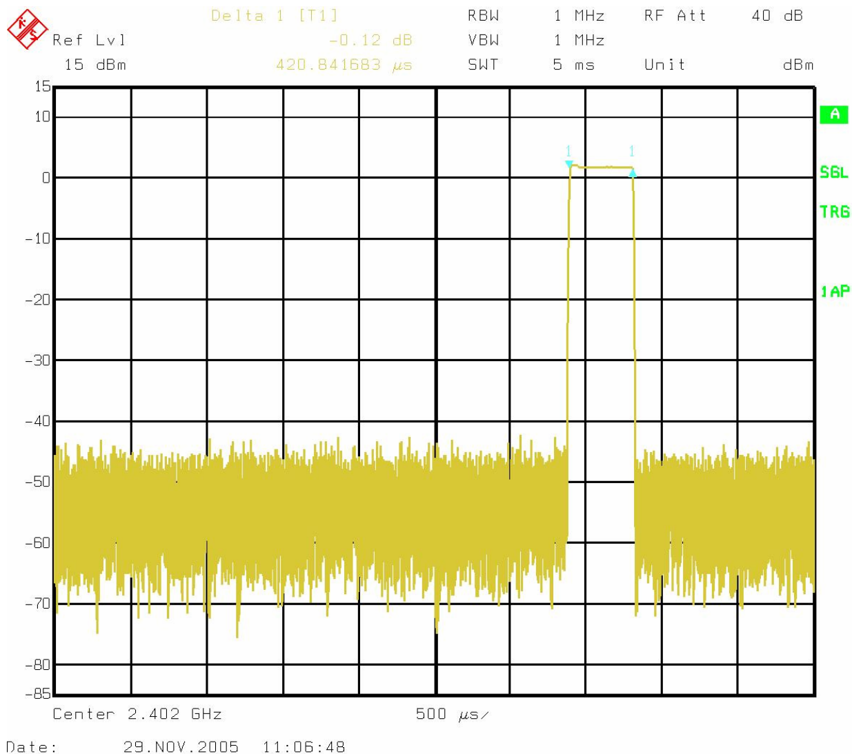
Figure 6-42: Plot of dwell time over 5 ms period
