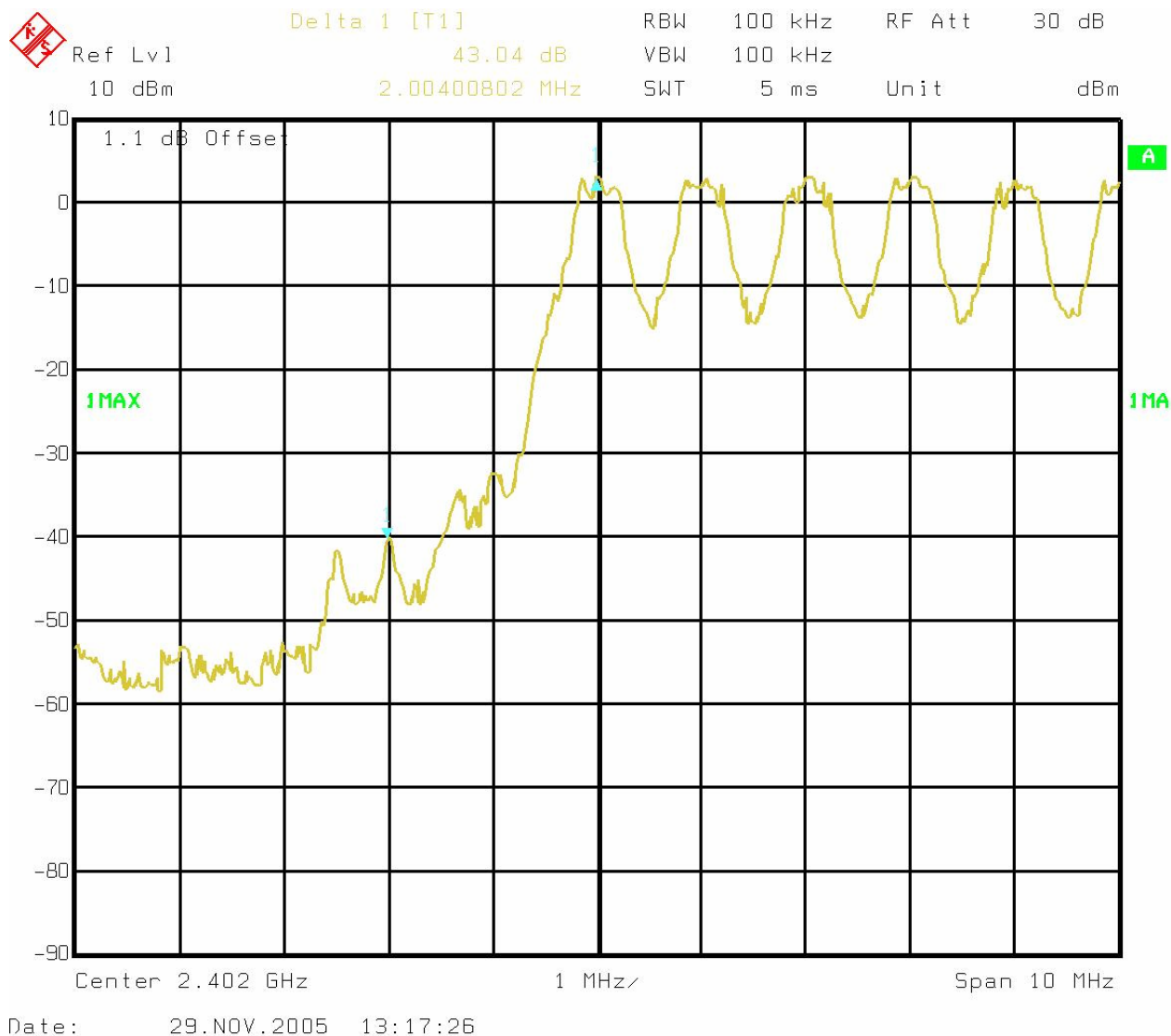
Figure 6-47: Plot of lower band-edge conducted emissions with hopping enabled
