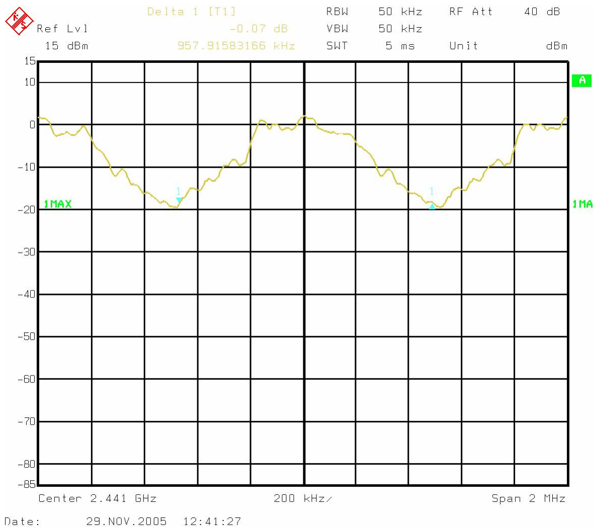
Figure 6-43: Plot of 20 – dB bandwidth
