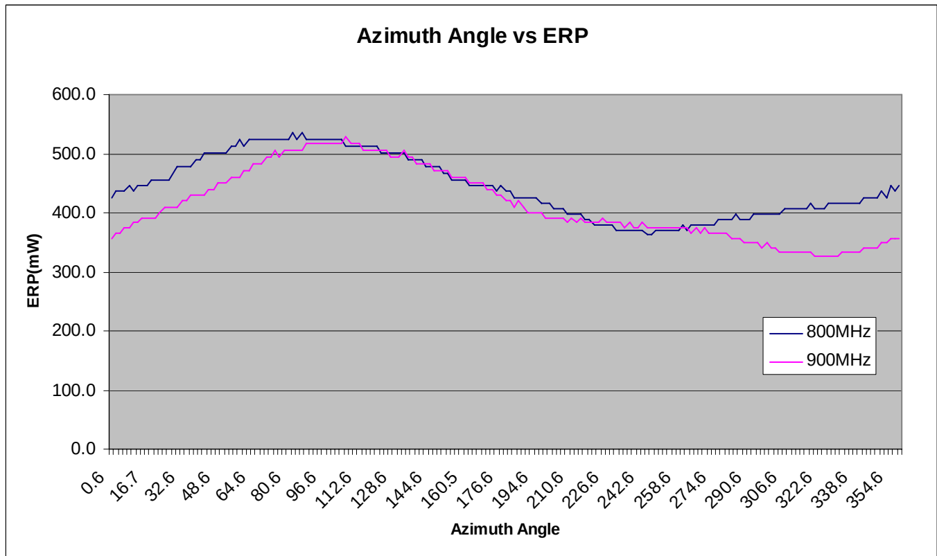
Figure 6a-94. Scaled ERP vs. Azimuth Angle
