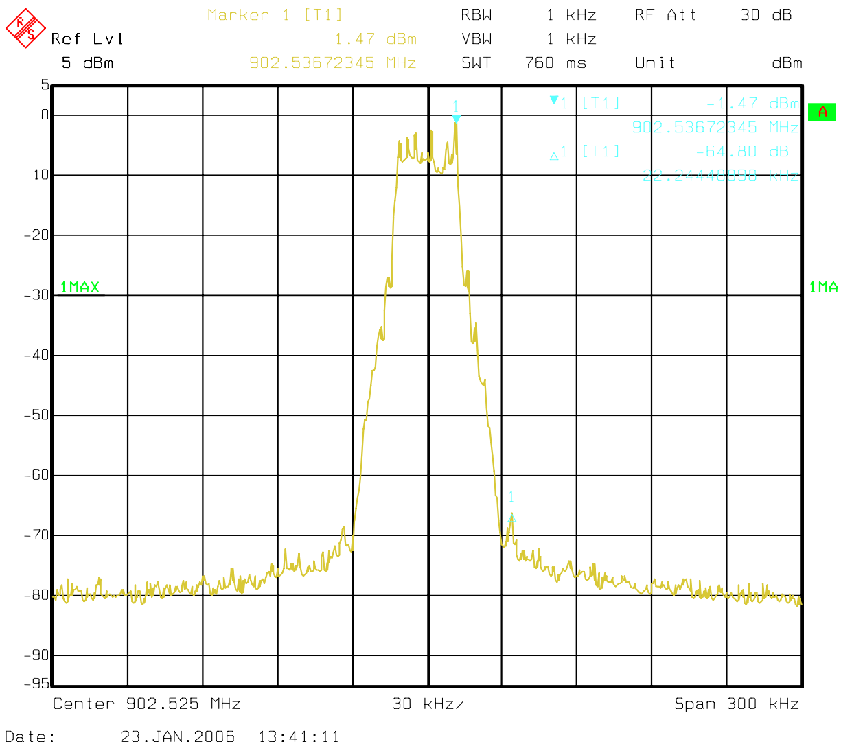
Figure 6b-2.2.3 MOTotalk Band Edge Emissions measurement at 902.525 MHz
