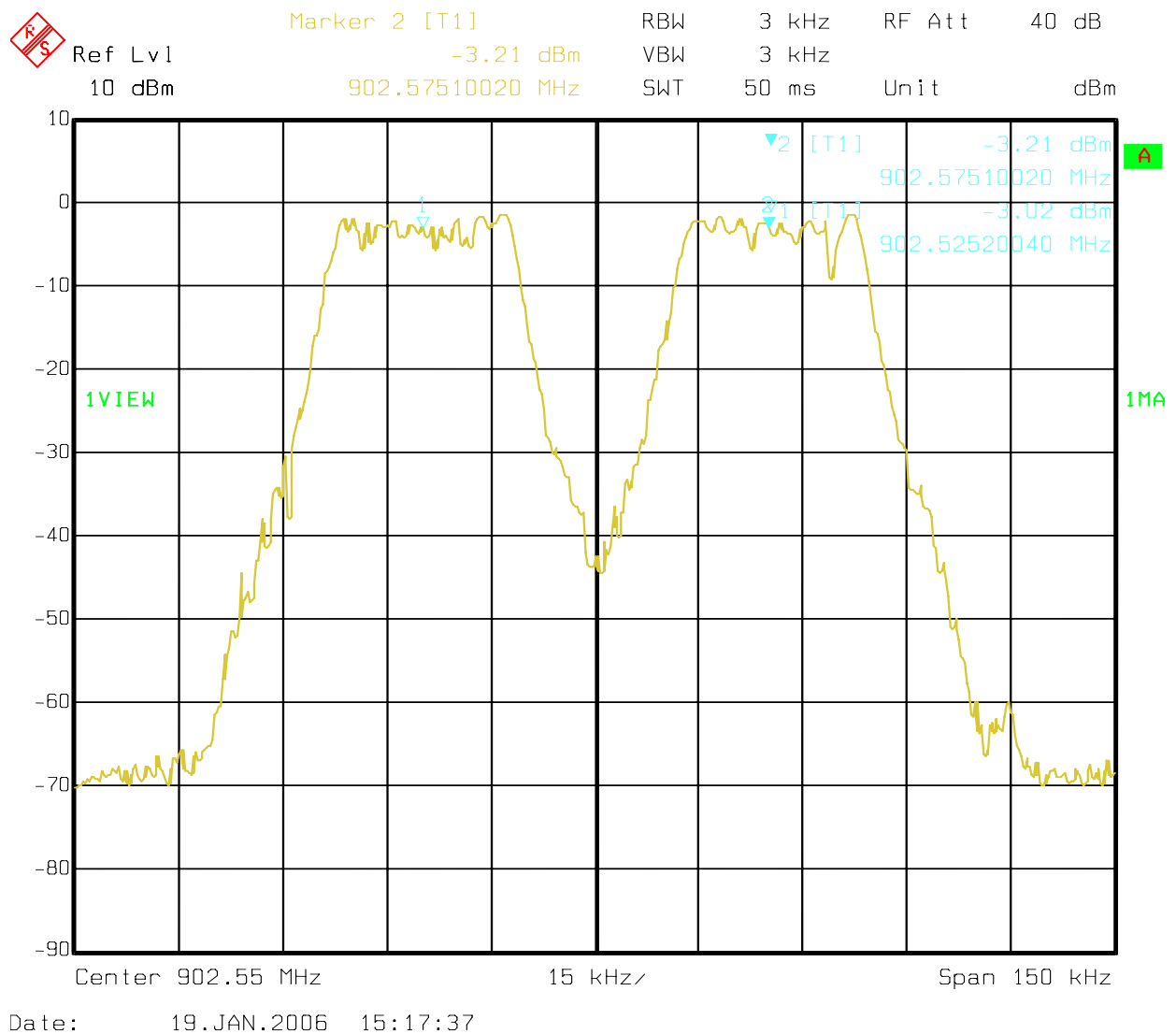
Figure 6b-2.2.2 MOTotalk Adjacent hop set separation between hopset1 @ 902.525 MHz and hopset2 @ 902.575 MHz
