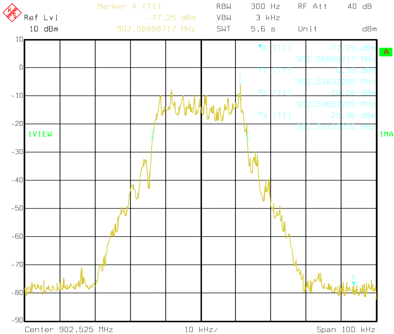
Figure 6b-2.2.1 MOTotalk 8-FSK traffic channel Occupied bandwidth at 902.525 MHz
