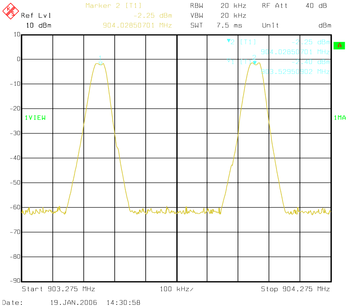
Figure 6b-2.1 Plot of MOTotalk ISM Band adjacent channel separation within a hopset
