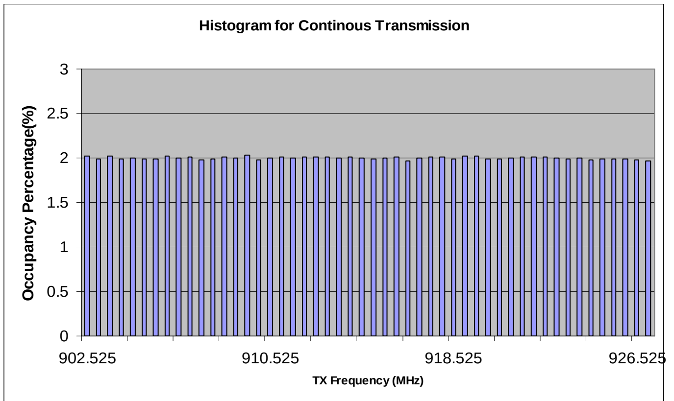
Figure 6b-2.6 Histogram for MOTotalk ISM Band Continuous Transmission
