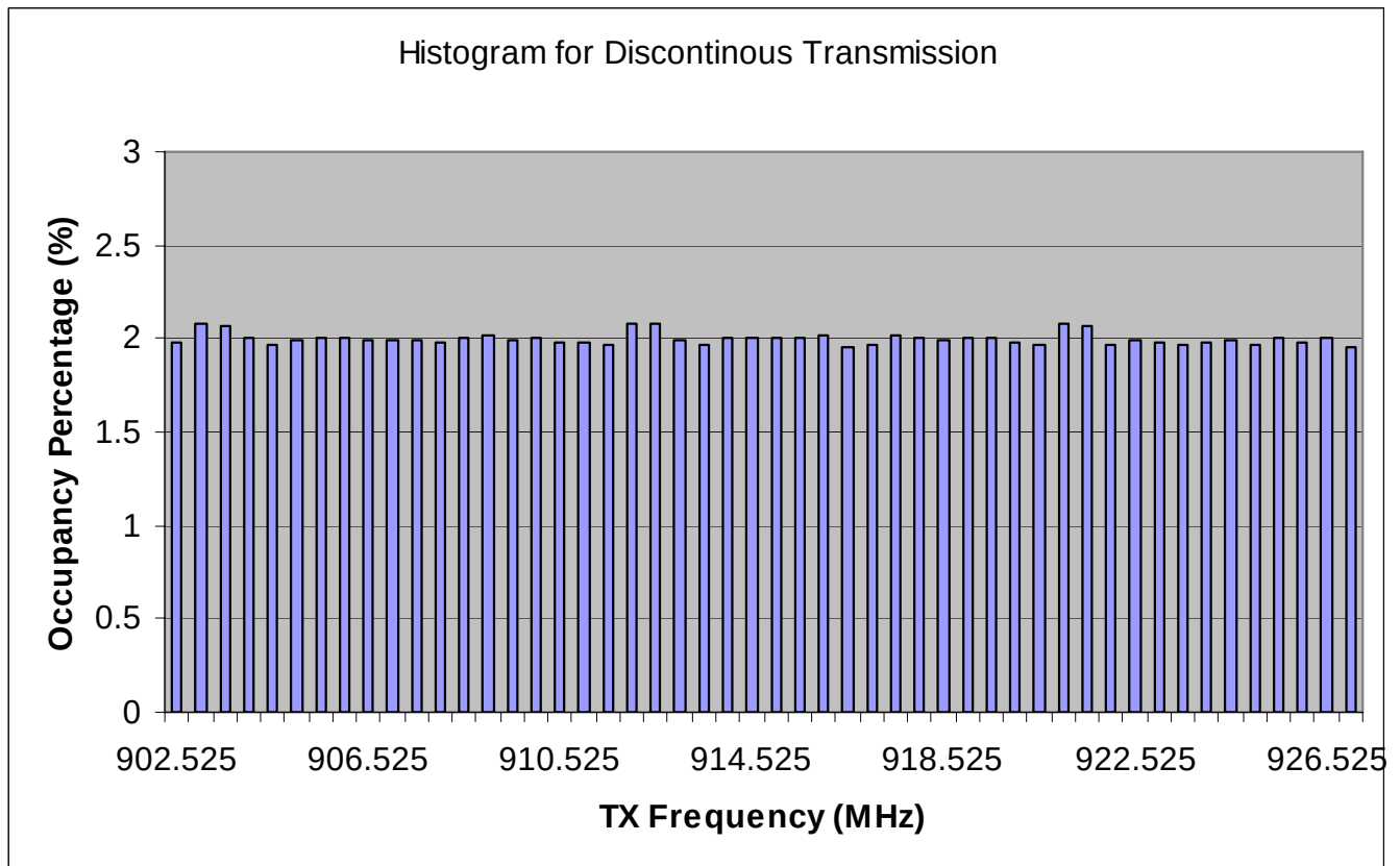
Figure 6b-2.7 Histogram for MOTotalk ISM Band Discontinuous Transmission
