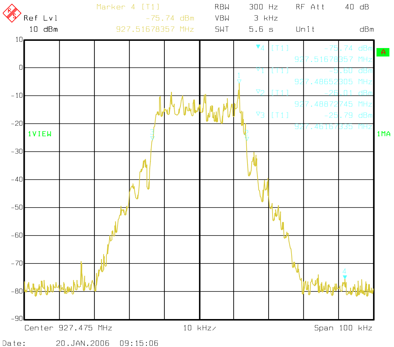
Figure 6b-2.2.4 MOTOTalk 8-FSK traffic channel Occupied bandwidth at 927.475 MHz
