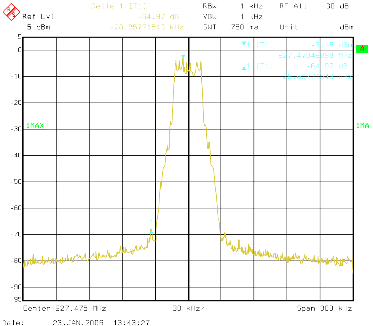
Figure 6b-2.2.6 Mototalk Band Edge Emissions measurement at 927.475 MHz
