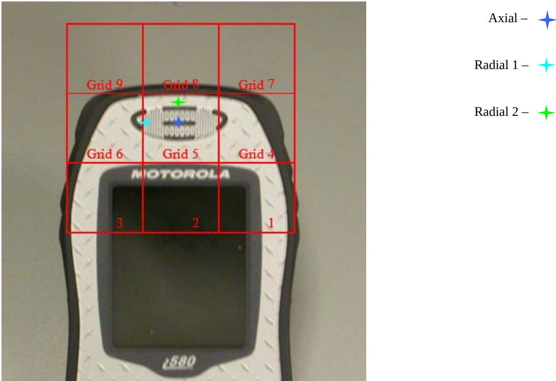
Figure 7-2 – Measurement Locations
