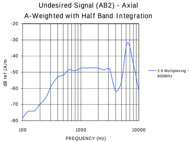
Figure 9-2-1 – 800MHz Undesired Signal (2:6)
