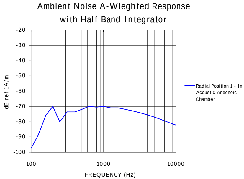
Figure 8-2 – Radial Position 1 Ambient Magnetic frequency distribution
