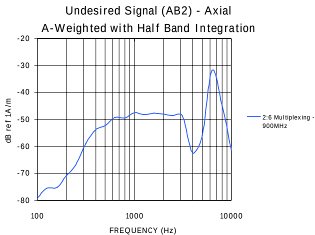
Figure 9-4-1 – 900MHz Undesired Signal (2:6)
