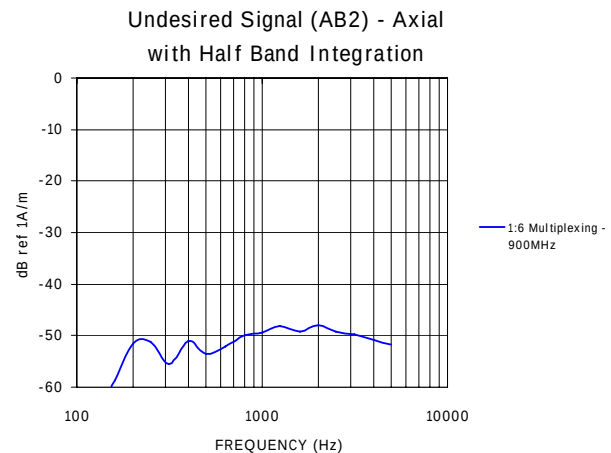
Figure 15B – 900MHz Undesired Signal (1:6)
