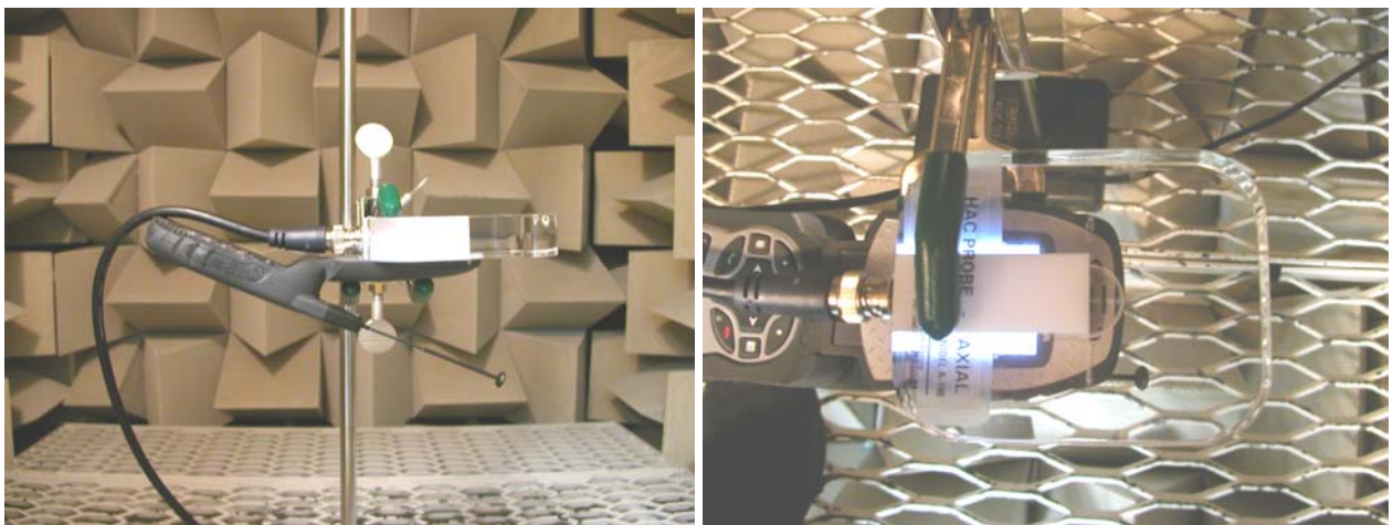
Figure 10 – Test holder
