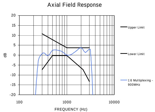
Figure 13D – 900MHz Measured Frequency response
