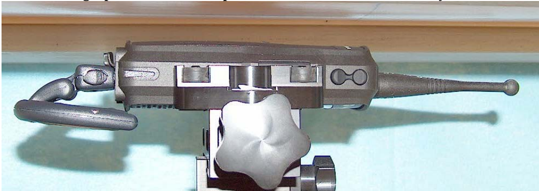
Figure 2: Body assessment DUT back housing separated 2.5cm from phantom with attached data accessory model NNTN5491A
