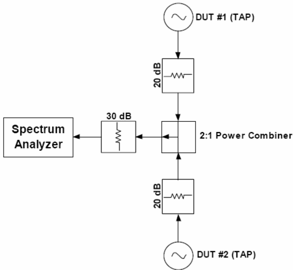
Figure 7-3: Test setup for multi-channel measurements.
