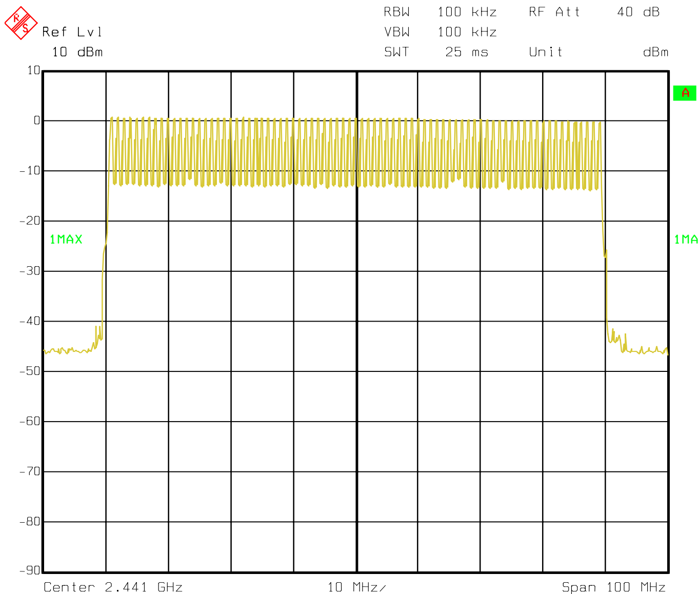
Figure 6-39: Plot of number of Bluetooth hopping frequencies
