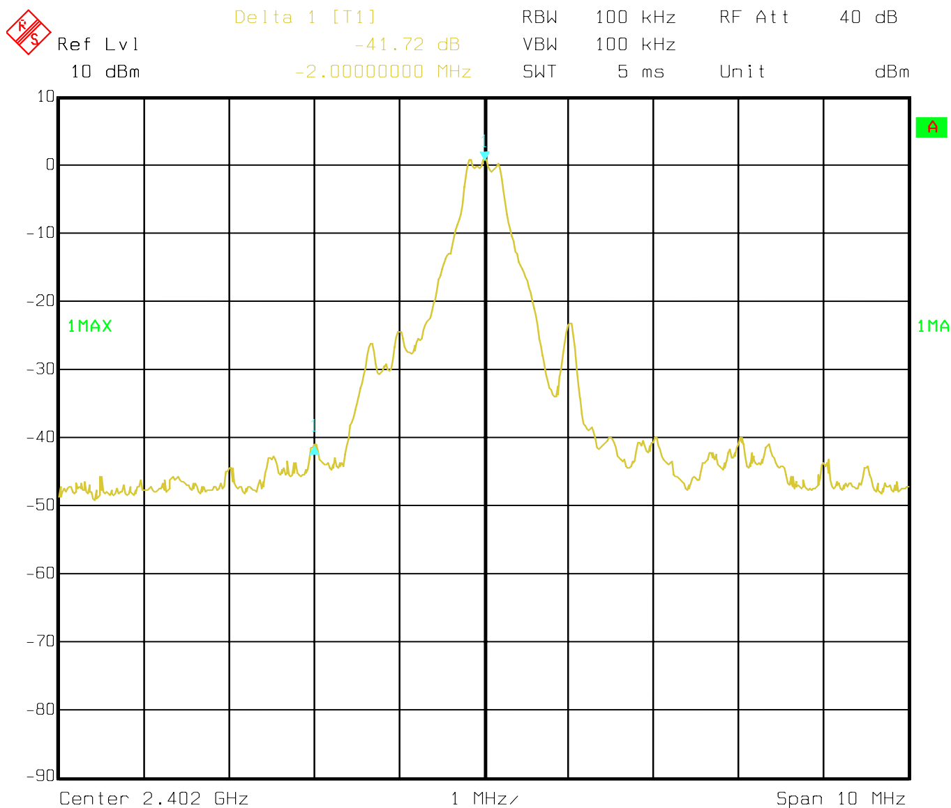
Figure 6-45: Plot of lower band-edge conducted emissions with hopping disabled
