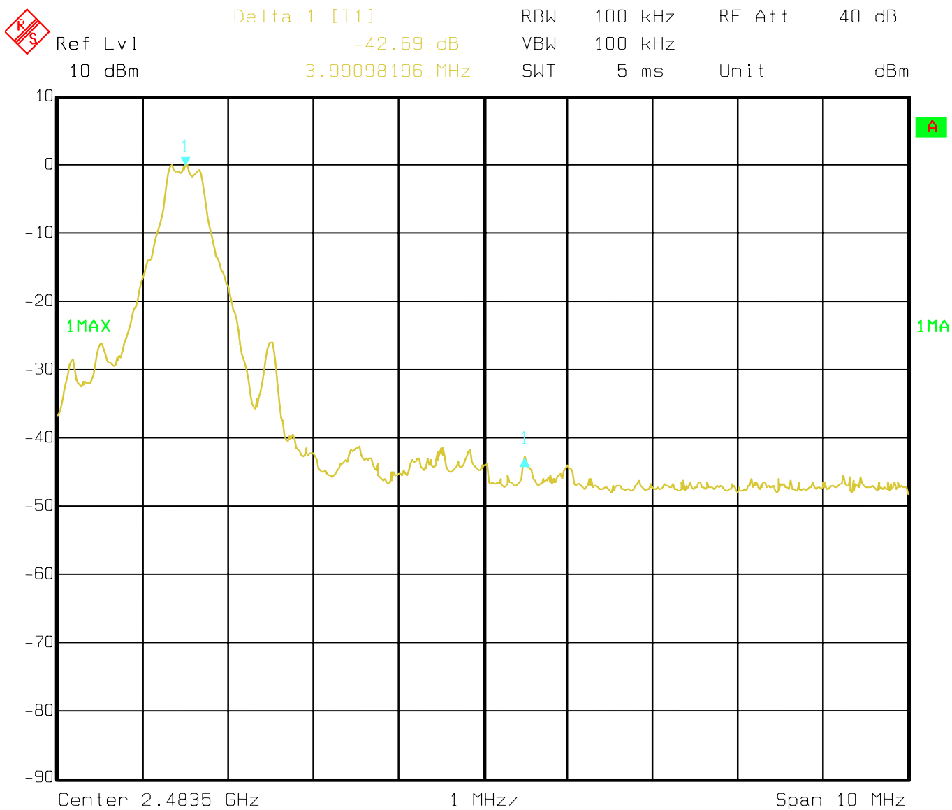
Figure 6-46: Plot of upper band-edge conducted emissions with hopping disabled
