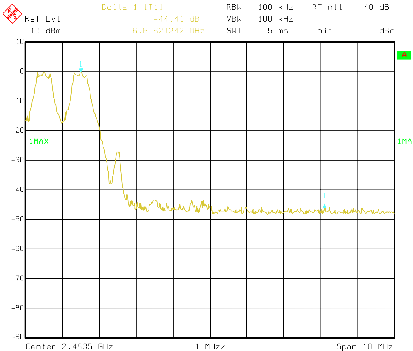
Figure 6-48: Plot of upper band-edge conducted emissions with hopping enabled
