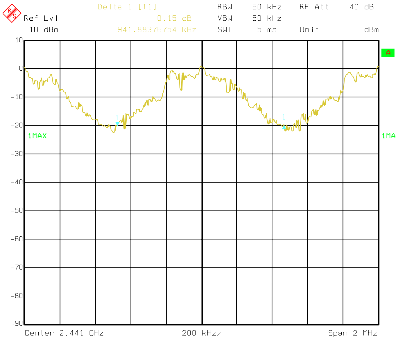
Figure 6-43: Plot of 20 – dB bandwidth
