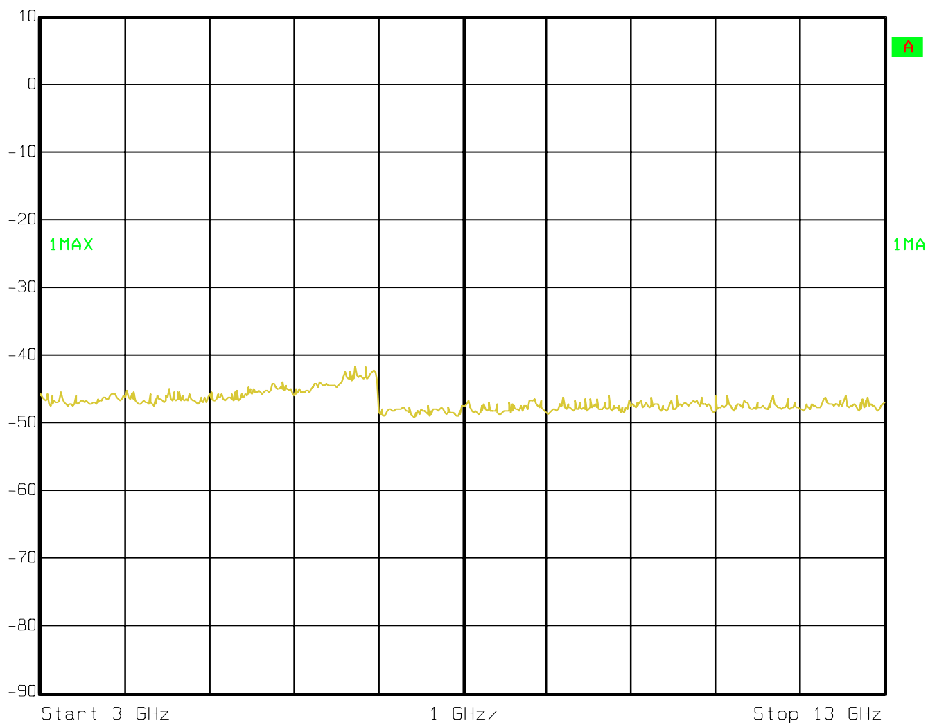
Figure 6-50: Plot of spurious conducted emissions 3 GHz – 13 GHz
