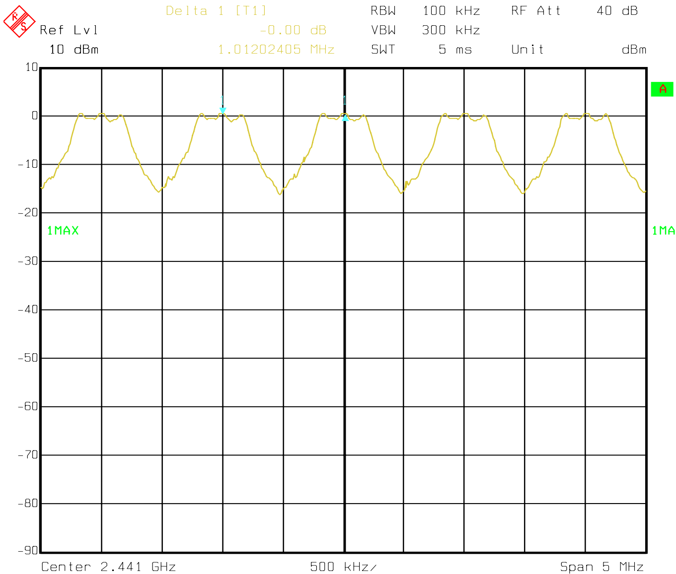
Figure 6-38: Plot of Bluetooth carrier frequency separation
