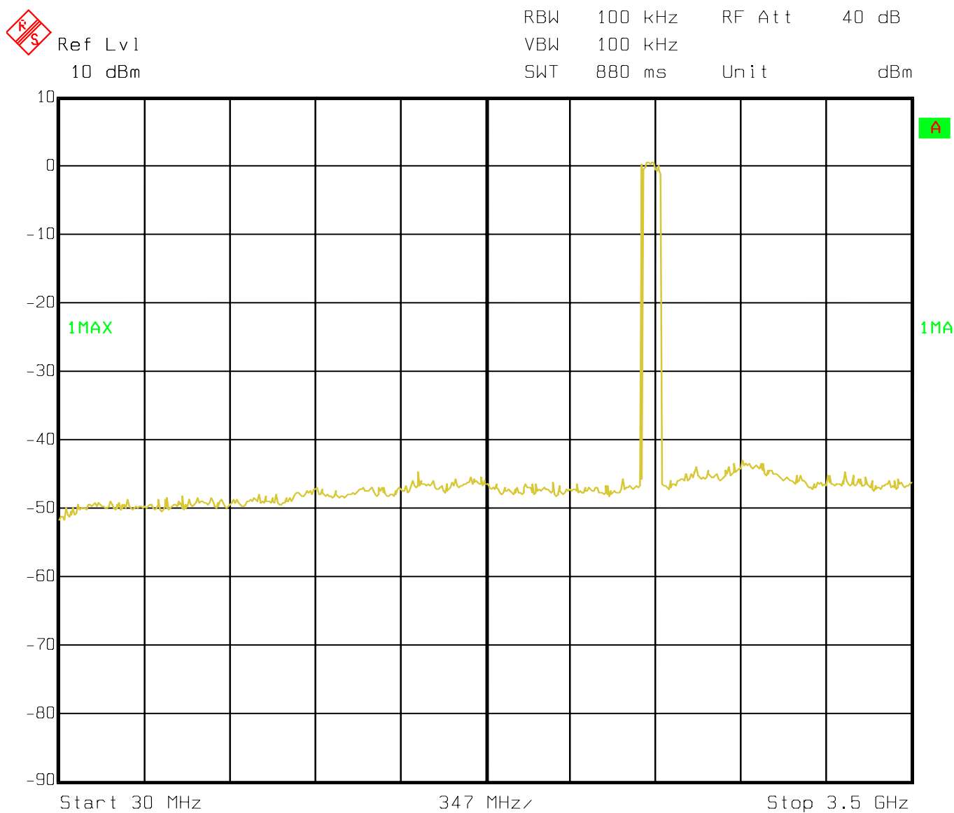
Figure 6-49: Plot of spurious conducted emissions 30 MHz – 3.5 GHz
