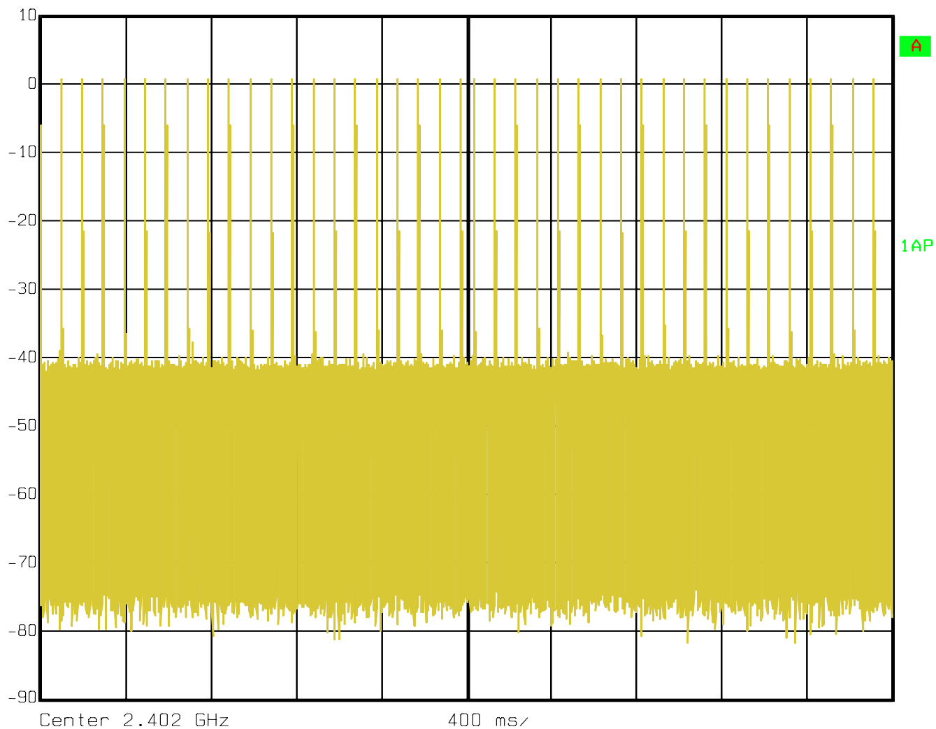
Figure 6-41: Plot of dwell time over 4 second period
