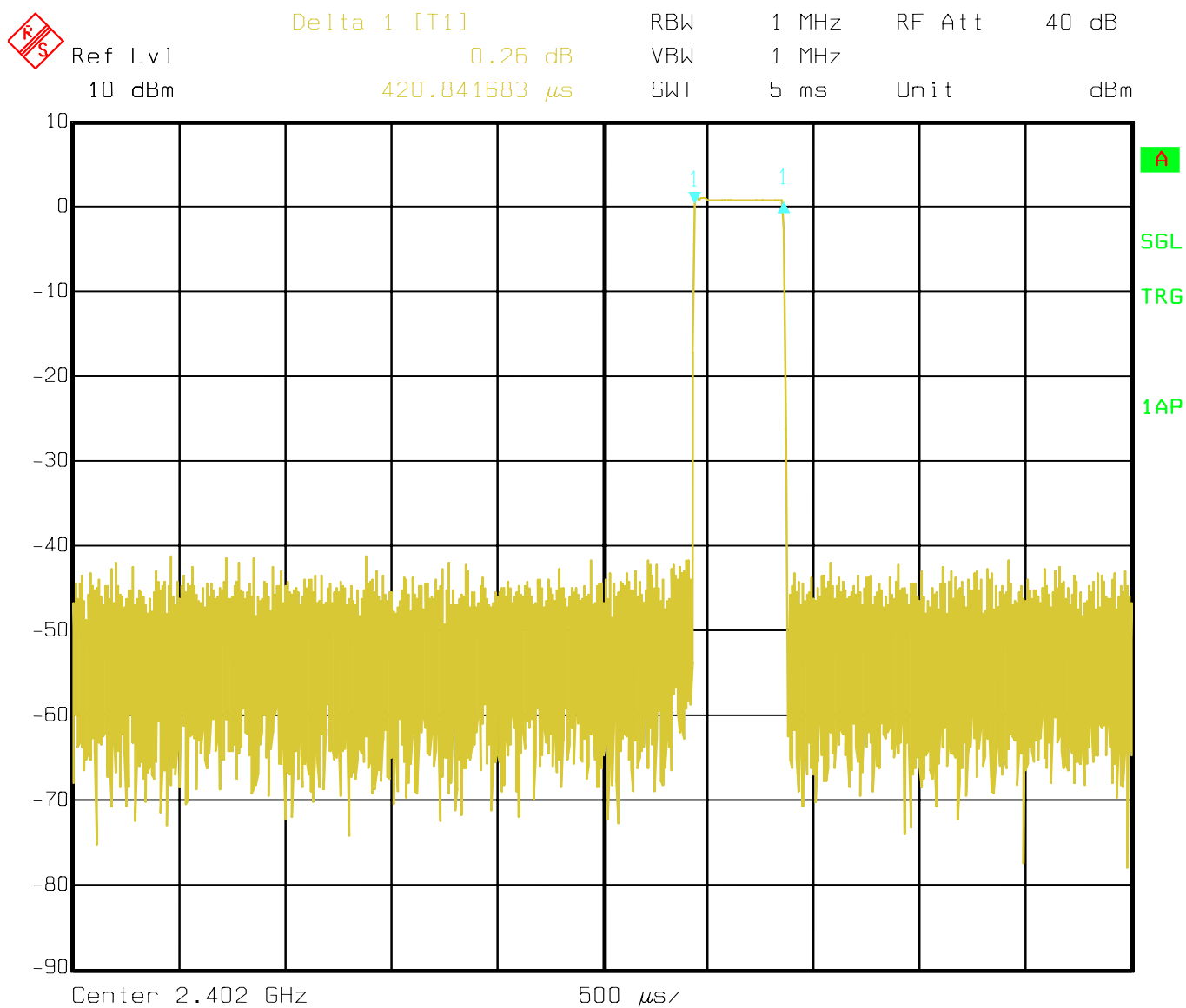
Figure 6-42: Plot of dwell time over 5 ms period
