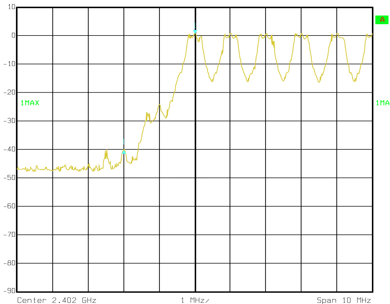
Figure 6-47: Plot of lower band-edge conducted emissions with hopping enabled
