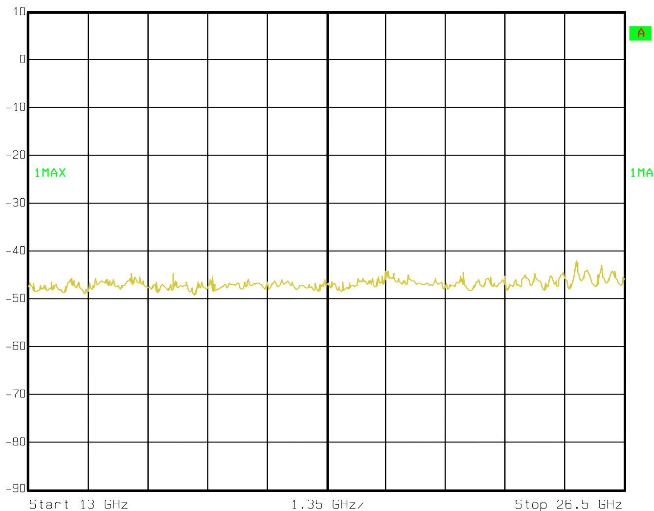
Figure 6-51: Plot of spurious conducted emissions 13 GHz – 26.5 GHz
