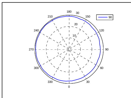
Figure 6a-6.3 Scaled ERP (dBm) vs different angle in 800 MHz band
