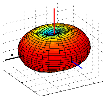
Figure 6a-6.2 i880 Antenna pattern at 900 MHz frequency band
