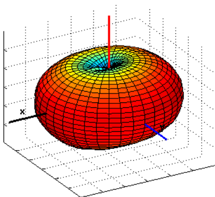
Figure 6a-6.1 i880 Antenna pattern at 800 MHz frequency band
