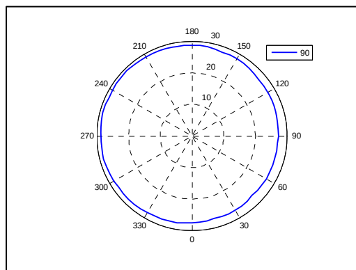
Figure 6a-6.4 Scaled ERP (dBm) vs different angle in 900 MHz Band
