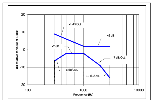
B - Mask for WDs with a field between -10 to -13dB at 1kHz
