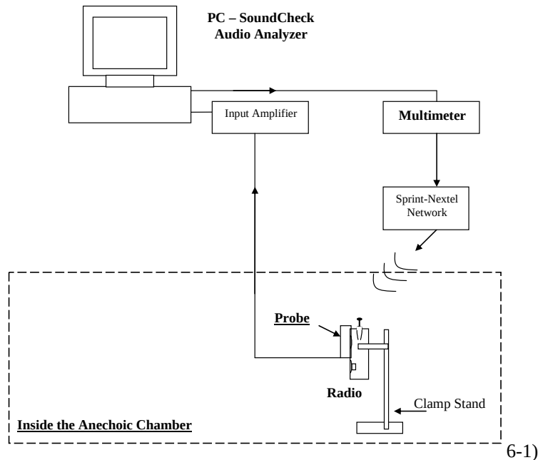
Figure 5-1 – Test setup
