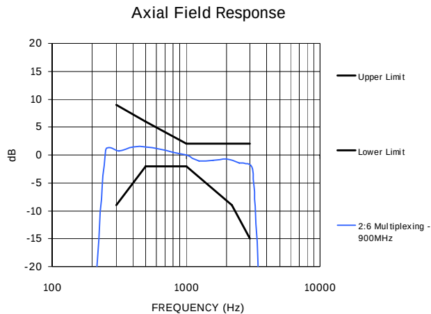
Figure 9-1-3 – 900 MHz Measured Frequency response
