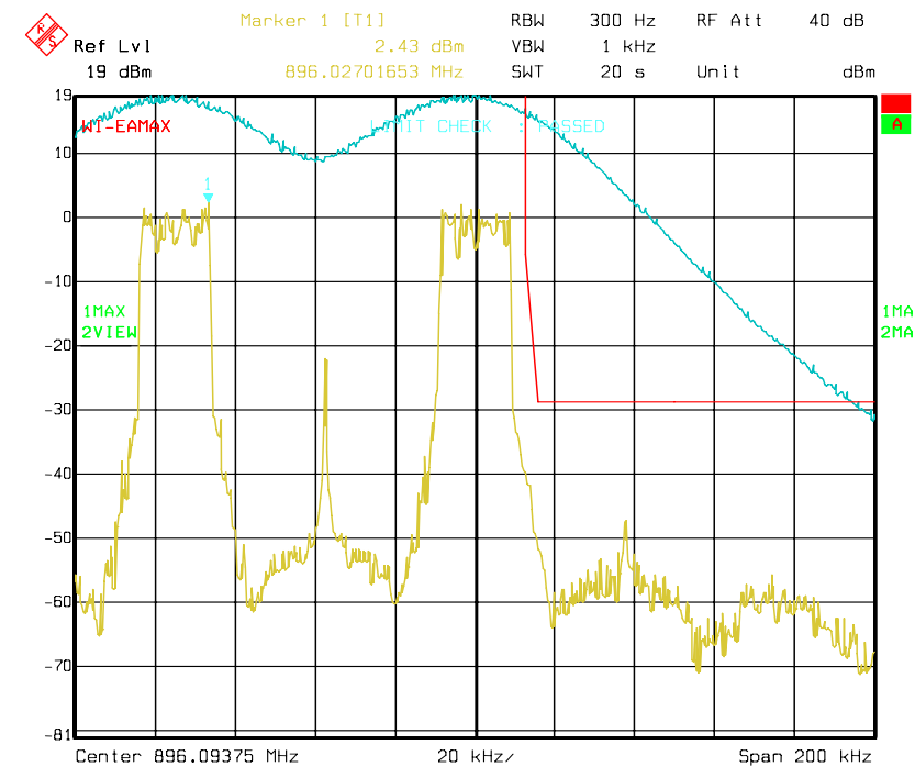
Figure 6a-2.12.3 WiDEN50_Split 900 MHz Band, QAM16, Maximum Power, EA Emission Mask
