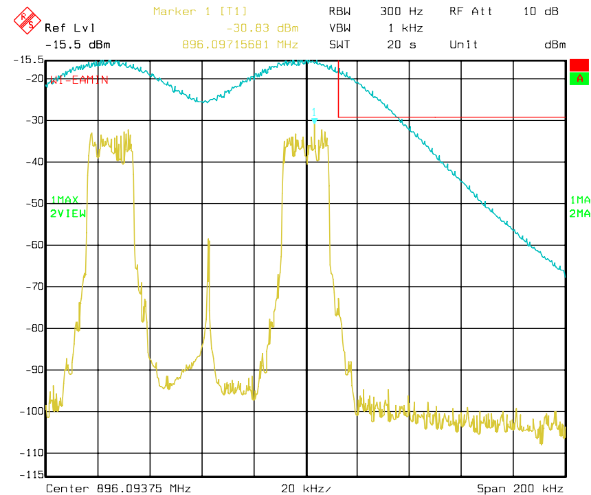
Figure 6a-2.12.4 WiDEN50_Split 900 MHz Band, QAM16, Minimum Power, EA Emission Mask
