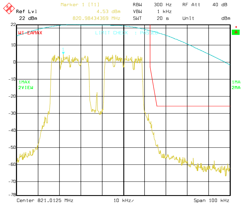
Figure 6a-2.4.5 WiDEN50 800 MHz Band, Continuous QAM64, Maximum Power, EA Emission Mask
