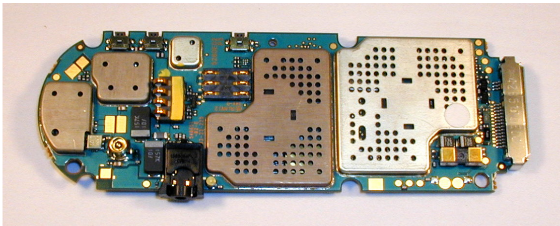
Photograph 9-1: Internal photo with shields intact
