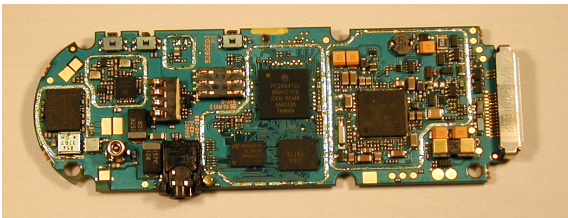
Photograph 9-4: Internal photo of electronic assembly with shields removed.
