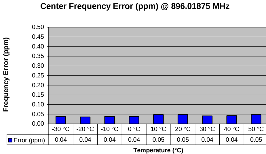
Figure 6a5-1: Transmitter Frequency Stability (900 MHz band) – Frequency Error vs. Temperature
