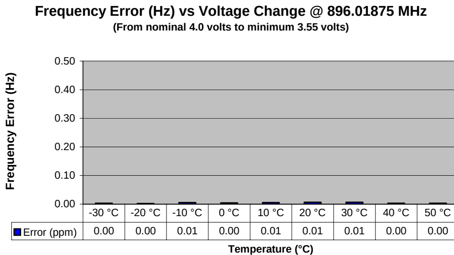
Figure 6a.5-2: Transmitter Frequency Stability (900 MHz band) - Frequency Error vs. Voltage
